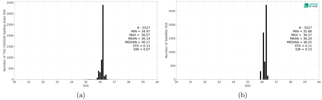
Figure 2: Histograms of SSS from TSG (GOSUD-Sailing-ship) (a) and CCI SSS L4 Merged-OI v4.4 - 7-day running (ESA) (b) considering all match-up pairs per bins of 0.1 over the Mississippi river plume Pi-MEP region and for the full satellite product period.
