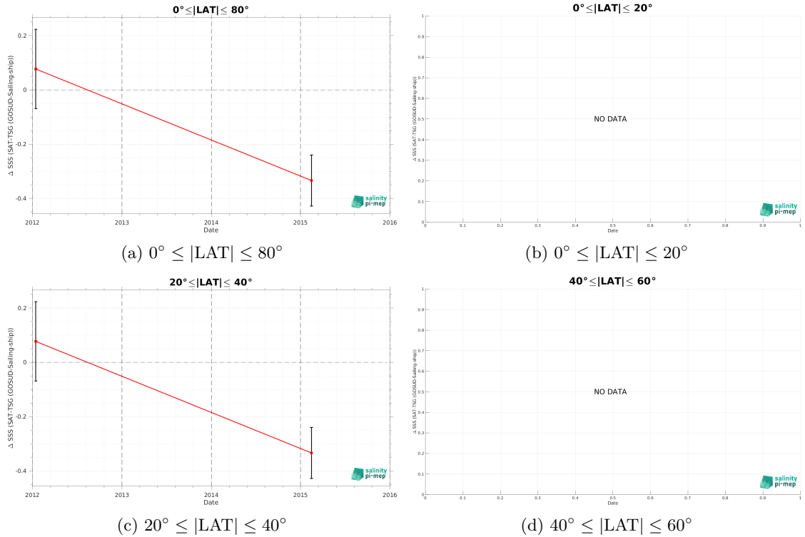
Figure 10: Monthly median (red curves) of \Delta SSS (Satellite - in situ ) between CCI SSS L4 Merged-OI v4.4 - 7-day running (ESA) and TSG (GOSUD-Sailing-ship) SSS as function of the geophysical conditions at match-up points. The median and std of \Delta SSS (Satellite - TSG (GOSUD-Sailing-ship)) is thus evaluated as function of the
