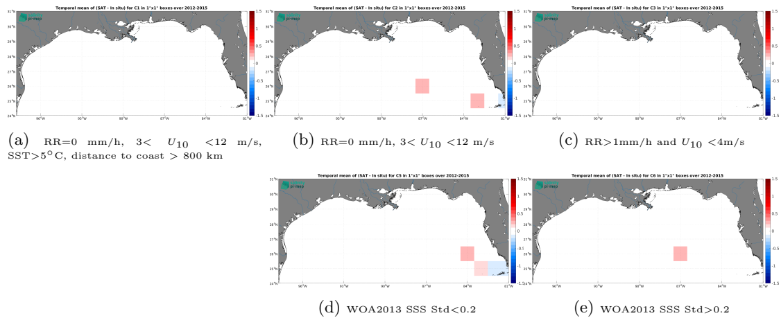
Figure 12: Temporal mean gridded over spatial boxes of size 1^{\circ}\times 1^{\circ} of \Delta SSS (CCI SSS L4 Merged-OI v4.4 - 7-day running (ESA) - TSG (GOSUD-Sailing-ship)) for 5 different subdatasets corresponding to: RR=0 mm/h, 3 < U_{10} < 12 m/s, SST > 5^{\circ}\text{C} , distance to coast > 800 km (a), RR=0 mm/h, 3 < U_{10} < 12 m/s (b), RR > 1 mm/h and U_{10} < 4 m/s (c), WOA2013 SSS Std < 0.2 (d), WOA2013 SSS Std > 0.2 (e).
