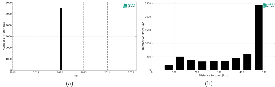
Figure 1: Number of match-ups between TSG (GOSUD-Sailing-ship) and CCI SSS L4 Merged-OI v4.4 - 7-day running (ESA) SSS as a function of time (a) and as function of the distance to coast (b) over the Mississippi river plume Pi-MEP region and for the full satellite product period.
