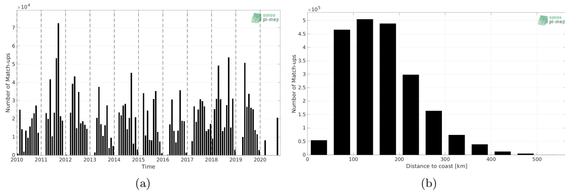
Figure 1: Number of match-ups between TSG (SAMOS) and CCI SSS L4 Merged-OI v3.2 - 7-day running (ESA) SSS as a function of time (a) and as function of the distance to coast (b) over the Mississippi river plume Pi-MEP region and for the full satellite product period.
