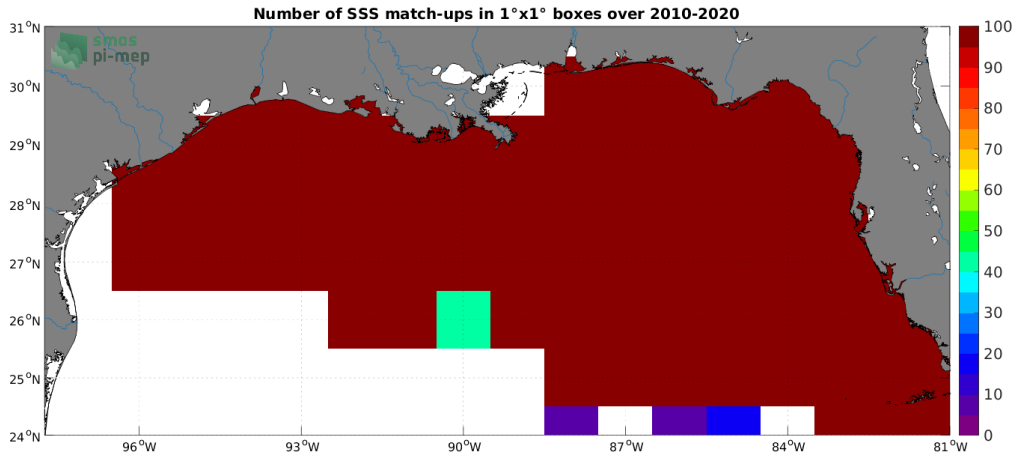
Figure 4: Number of SSS match-ups between TSG (SAMOS) SSS and the CCI SSS L4 Merged-OI v3.2 - 7-day running (ESA) SSS product for the Mississippi river plume Pi-MEP region over 1^\circ \times 1^\circ boxes and for the full satellite product period.
