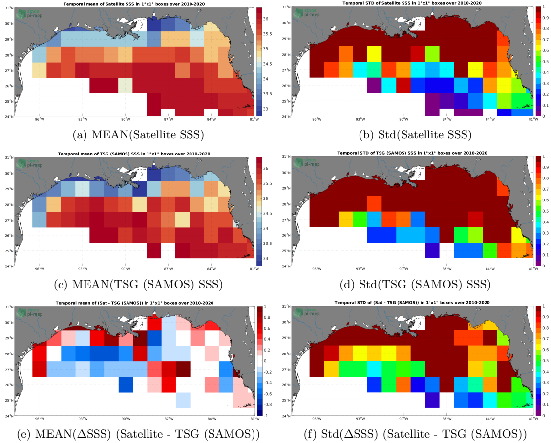
Figure 6: Temporal mean (left) and Std (right) of SSS from CCI SSS L4 Merged-OI v3.2 - 7-day running (ESA) (top), TSG (SAMOS) (middle), and of \Delta\text{SSS} (Satellite - TSG (SAMOS)). Only match-up pairs are used to generate these maps.
