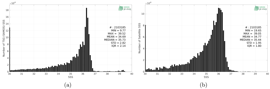
Figure 2: Histograms of SSS from TSG (SAMOS) (a) and CCI SSS L4 Merged-OI v3.2 - 7-day running (ESA) (b) considering all match-up pairs per bins of 0.1 over the Mississippi river plume Pi-MEP region and for the full satellite product period.
