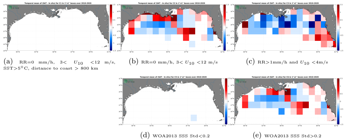
Figure 12: Temporal mean gridded over spatial boxes of size 1^{\circ}\times 1^{\circ} of \Delta\text{SSS} (CCI SSS L4 Merged-OI v3.2 - 7-day running (ESA) - TSG (SAMOS)) for 5 different subdatasets corresponding to:RR=0 mm/h, 3 < U_{10} < 12 m/s, SST >5^{\circ}\text{C} , distance to coast > 800 km (a), RR=0 mm/h, 3 < U_{10} < 12 m/s (b), RR >1 mm/h and U_{10} < 4 m/s (c), WOA2013 SSS Std <0.2 (d), WOA2013 SSS Std >0.2 (e).
