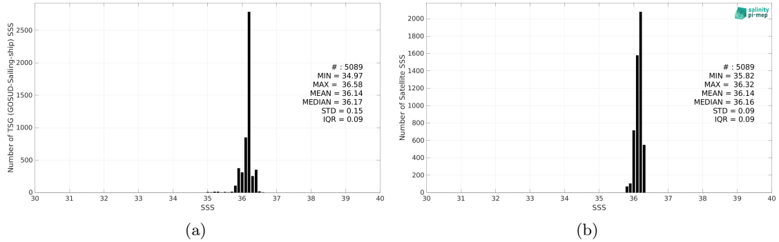
Figure 2: Histograms of SSS from TSG (GOSUD-Sailing-ship) (a) and CCI SSS L4 Merged-OI v3.2 - 7-day running (ESA) (b) considering all match-up pairs per bins of 0.1 over the Mississippi river plume Pi-MEP region and for the full satellite product period.
