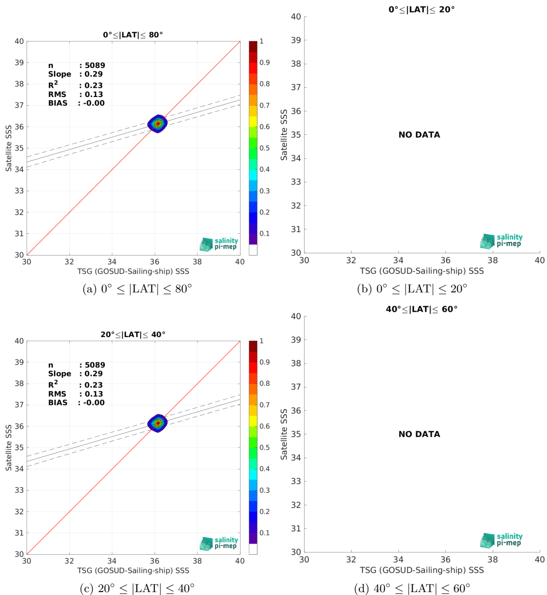
Figure 9: Contour maps of the concentration of CCI SSS L4 Merged-OI v3.2 - 7-day running (ESA) SSS (y-axis) versus TSG (GOSUD-Sailing-ship) SSS (x-axis) at match-up pairs for different latitude bands. For each plot, the red line shows x=y . The black thin and dashed lines indicate a linear fit through the data cloud and the \pm 95\% confidence levels, respectively. The number match-up pairs n , the slope and R^2 coefficient of the linear fit, the root mean square (RMS) and the mean bias between satellite and in situ data are indicated for each latitude band in each plots.
