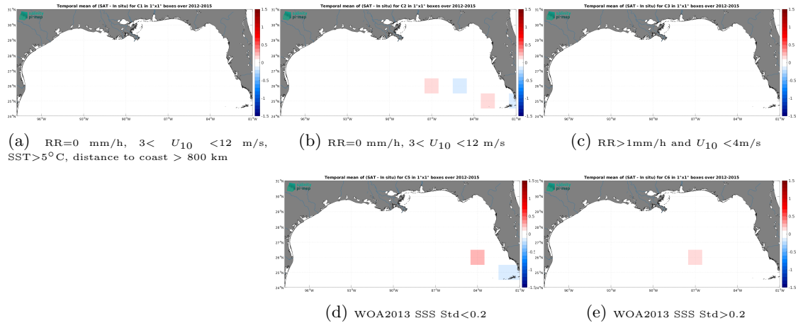
Figure 12: Temporal mean gridded over spatial boxes of size 1^{\circ}\times 1^{\circ} of \Delta SSS (CCI SSS L4 Merged-OI v3.2 - 7-day running (ESA) - TSG (GOSUD-Sailing-ship)) for 5 different subdatasets corresponding to: RR=0 mm/h, 3 < U_{10} < 12 m/s, SST > 5^{\circ}\text{C} , distance to coast > 800 km (a), RR=0 mm/h, 3 < U_{10} < 12 m/s (b), RR > 1 mm/h and U_{10} < 4 m/s (c), WOA2013 SSS Std < 0.2 (d), WOA2013 SSS Std > 0.2 (e).
