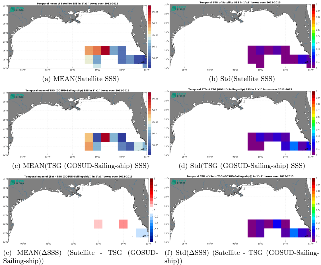
Figure 6: Temporal mean (left) and Std (right) of SSS from CCI SSS L4 Merged-OI v3.2 - 7-day running (ESA) (top), TSG (GOSUD-Sailing-ship) (middle), and of \Delta\text{SSS} (Satellite - TSG (GOSUD-Sailing-ship)). Only match-up pairs are used to generate these maps.
