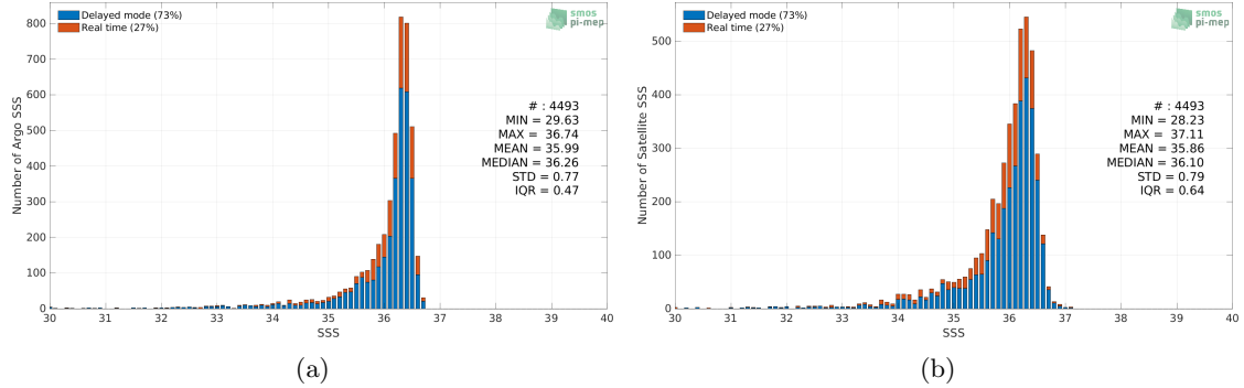
Figure 2: Histograms of SSS from Argo (a) and CCI SSS L4 Merged-OI v3.2 - 7-day running (ESA) (b) considering all match-up pairs per bins of 0.1 over the Mississippi river plume Pi-MEP region and for the full satellite product period.
