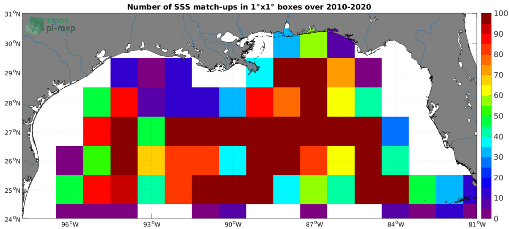
Figure 4: Number of SSS match-ups between Argo SSS and the CCI SSS L4 Merged-OI v3.2 - 7-day running (ESA) SSS product for the Mississippi river plume Pi-MEP region over 1^\circ \times 1^\circ boxes and for the full satellite product period.
