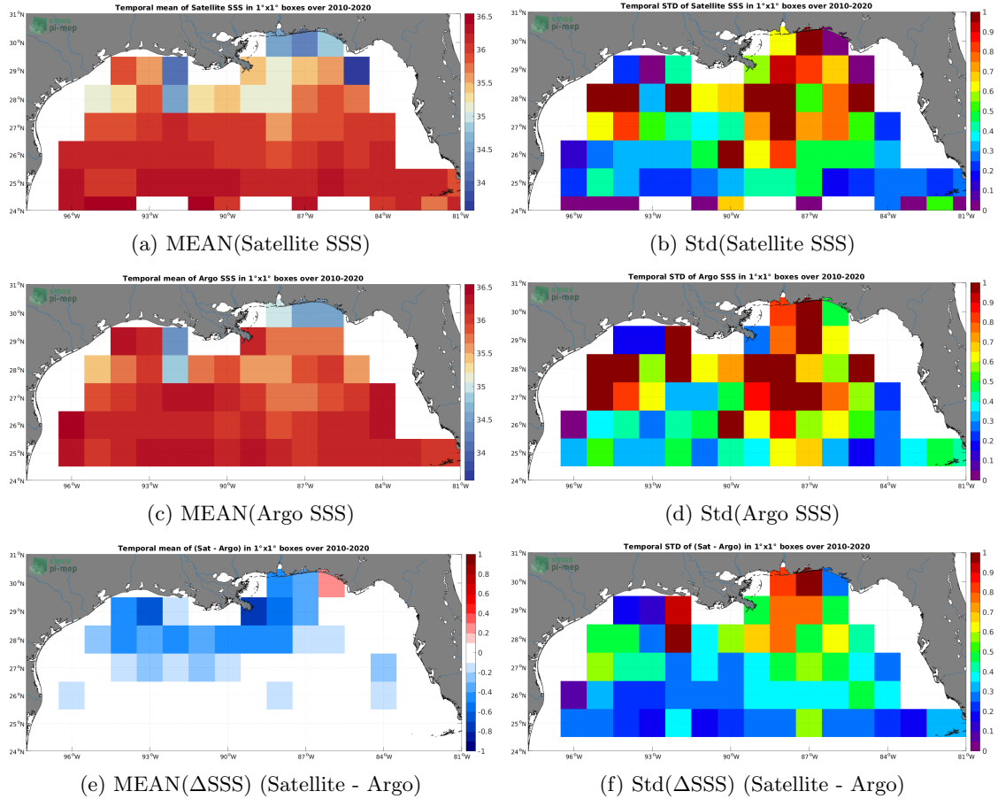
Figure 6: Temporal mean (left) and Std (right) of SSS from CCI SSS L4 Merged-OI v3.2 - 7-day running (ESA) (top), Argo (middle), and of \Delta\text{SSS} (Satellite - Argo). Only match-up pairs are used to generate these maps.
