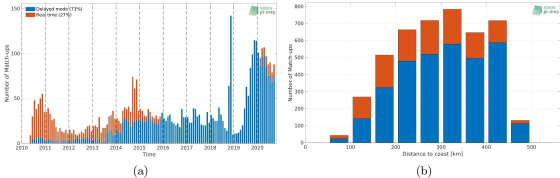
Figure 1: Number of match-ups between Argo and CCI SSS L4 Merged-OI v3.2 - 7-day running (ESA) SSS as a function of time (a) and as function of the distance to coast (b) over the Mississippi river plume Pi-MEP region and for the full satellite product period.
