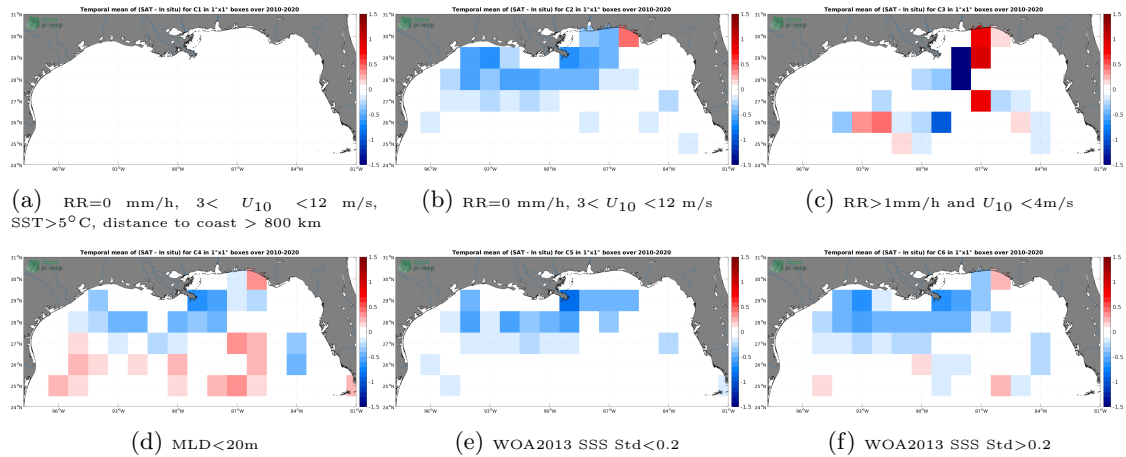
Figure 12: Temporal mean gridded over spatial boxes of size 1^{\circ}\times 1^{\circ} of \Delta\text{SSS} (CCI SSS L4 Merged-OI v3.2 - 7-day running (ESA) - Argo) for 6 different subdatasets corresponding to:RR=0 mm/h, 3 < U_{10} < 12 m/s, SST > 5^{\circ}\text{C} , distance to coast > 800 km (a), RR=0 mm/h, 3 < U_{10} < 12 m/s (b), RR > 1\text{mm/h} and U_{10} < 4\text{m/s} (c),MLD < 20\text{m} (d),WOA2013 SSS Std < 0.2 (e),WOA2013 SSS Std > 0.2 (f).
