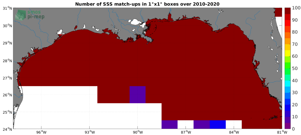
Figure 4: Number of SSS match-ups between TSG (SAMOS) SSS and the CCI SSS L4 Merged-OI v3.2 - 30-day running (ESA) SSS product for the Mississippi river plume Pi-MEP region over 1^\circ \times 1^\circ boxes and for the full satellite product period.
