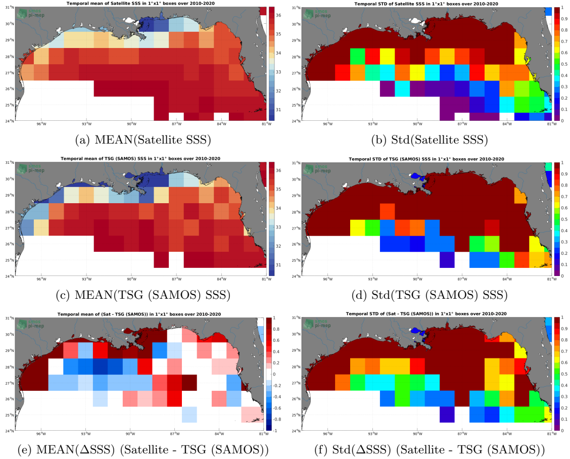
Figure 6: Temporal mean (left) and Std (right) of SSS from CCI SSS L4 Merged-OI v3.2 - 30-day running (ESA) (top), TSG (SAMOS) (middle), and of \Delta\text{SSS} (Satellite - TSG (SAMOS)). Only match-up pairs are used to generate these maps.
