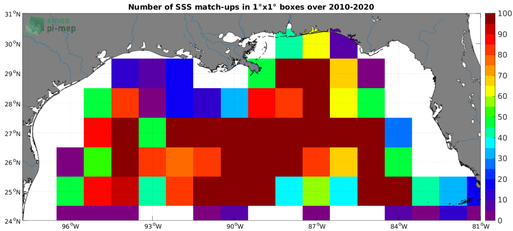
Figure 4: Number of SSS match-ups between Argo SSS and the CCI SSS L4 Merged-OI v3.2 - 30-day running (ESA) SSS product for the Mississippi river plume Pi-MEP region over 1^\circ \times 1^\circ boxes and for the full satellite product period.
