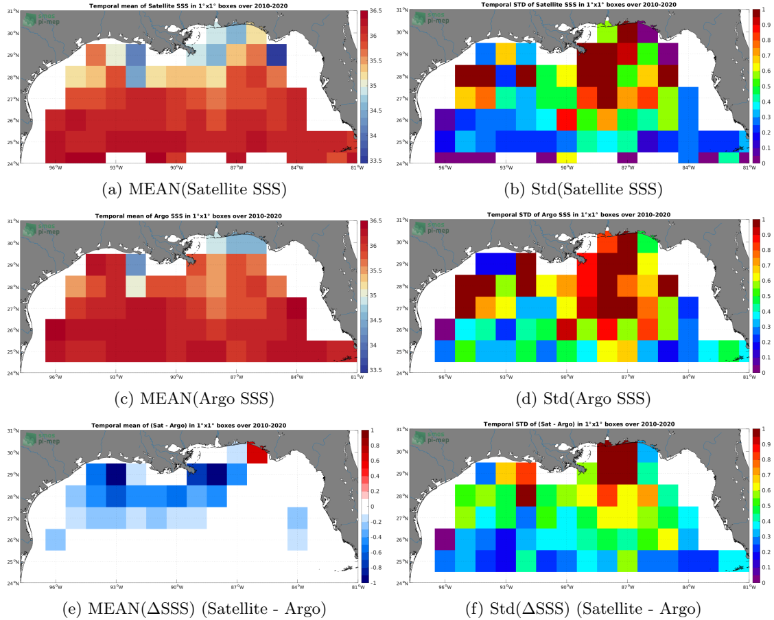
Figure 6: Temporal mean (left) and Std (right) of SSS from CCI SSS L4 Merged-OI v3.2 - 30-day running (ESA) (top), Argo (middle), and of \Delta\text{SSS} (Satellite - Argo). Only match-up pairs are used to generate these maps.
