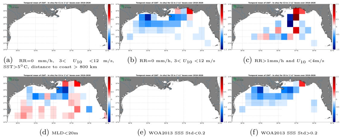
Figure 12: Temporal mean gridded over spatial boxes of size 1^{\circ}\times 1^{\circ} of \Delta\text{SSS} (CCI SSS L4 Merged-OI v3.2 - 30-day running (ESA) - Argo) for 6 different subdatasets corresponding to:RR=0 mm/h, 3 < U_{10} < 12 m/s, \text{SST} > 5^{\circ}\text{C} , distance to coast > 800 km (a), RR=0 mm/h, 3 < U_{10} < 12 m/s (b), RR >1 mm/h and U_{10} < 4\text{m/s} (c),MLD <20\text{m} (d),WOA2013 SSS Std <0.2 (e),WOA2013 SSS Std >0.2 (f).
