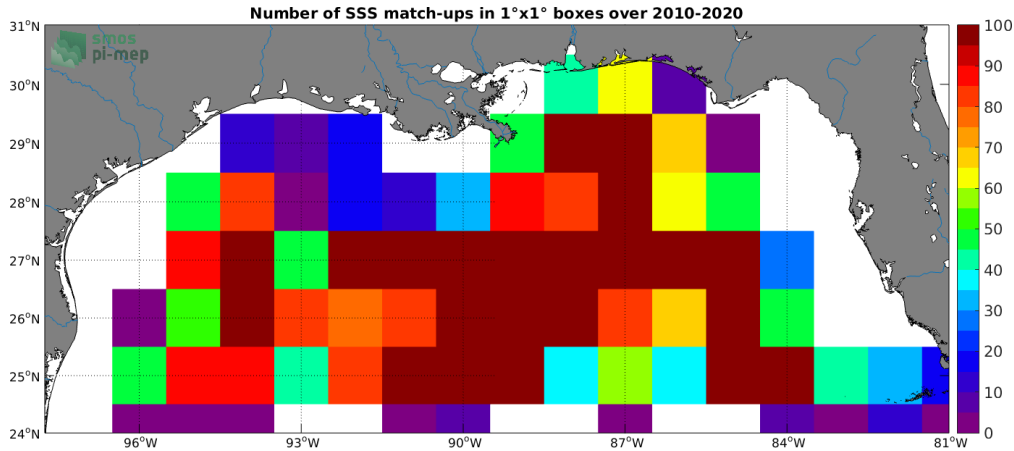
Figure 4: Number of SSS match-ups between Argo SSS and the CCI SSS L4 Merged-OI v3.2 - 30-day running (ESA) SSS product for the Mississippi river plume Pi-MEP region over 1^{\circ} \times 1^{\circ} boxes and for the full satellite product period.
