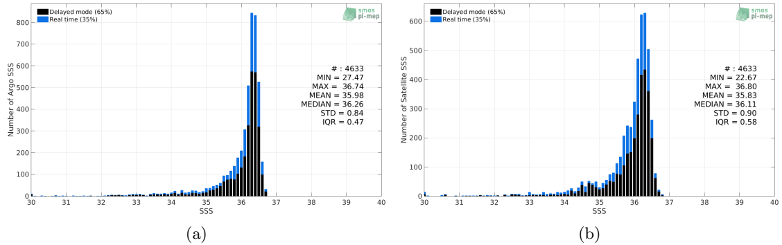
Figure 2: Histograms of SSS from Argo (a) and CCI SSS L4 Merged-OI v3.2 - 30-day running (ESA) (b) considering all match-up pairs per bins of 0.1 over the Mississippi river plume Pi-MEP region and for the full satellite product period.
