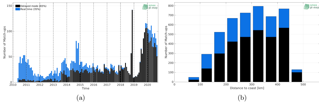
Figure 1: Number of match-ups between Argo and CCI SSS L4 Merged-OI v3.2 - 30-day running (ESA) SSS as a function of time (a) and as function of the distance to coast (b) over the Mississippi river plume Pi-MEP region and for the full satellite product period.
