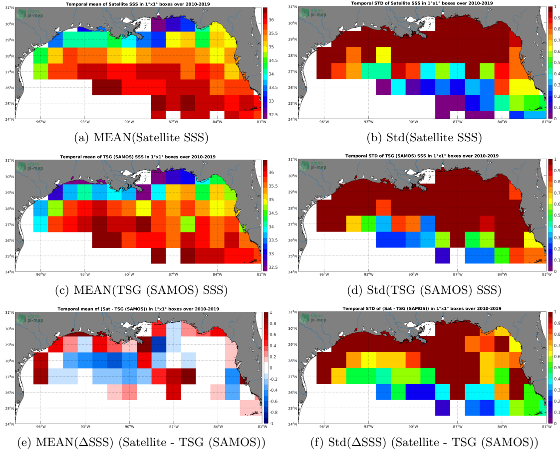
Figure 6: Temporal mean (left) and Std (right) of SSS from CCI SSS L4 Merged-OI v2.31 - 7-day running (ESA) (top), TSG (SAMOS) (middle), and of \Delta\text{SSS} (Satellite - TSG (SAMOS)). Only match-up pairs are used to generate these maps.
