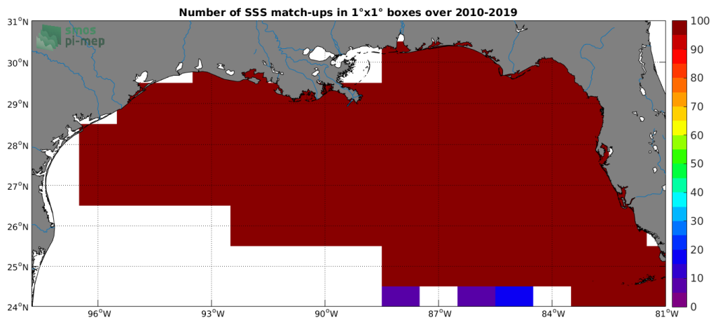
Figure 4: Number of SSS match-ups between TSG (SAMOS) SSS and the CCI L4 Merged-OI v2.31 - 7-day running (ESA) SSS product for the Mississippi river plume Pi-MEP region over 1^\circ \times 1^\circ boxes and for the full satellite product period.
