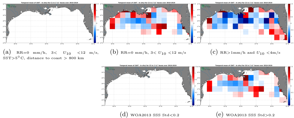
Figure 12: Temporal mean gridded over spatial boxes of size 1^{\circ}\times 1^{\circ} of \Delta\text{SSS} (CCI L4 Merged-OI v2.31 - 7-day running (ESA) - TSG (SAMOS)) for 5 different subdatasets corresponding to:RR=0 mm/h, 3 < U_{10} < 12 m/s, SST >5^{\circ}\text{C} , distance to coast > 800 km (a), RR=0 mm/h, 3 < U_{10} < 12 m/s (b), RR >1 mm/h and U_{10} < 4 m/s (c), WOA2013 SSS Std <0.2 (d), WOA2013 SSS Std >0.2 (e).
