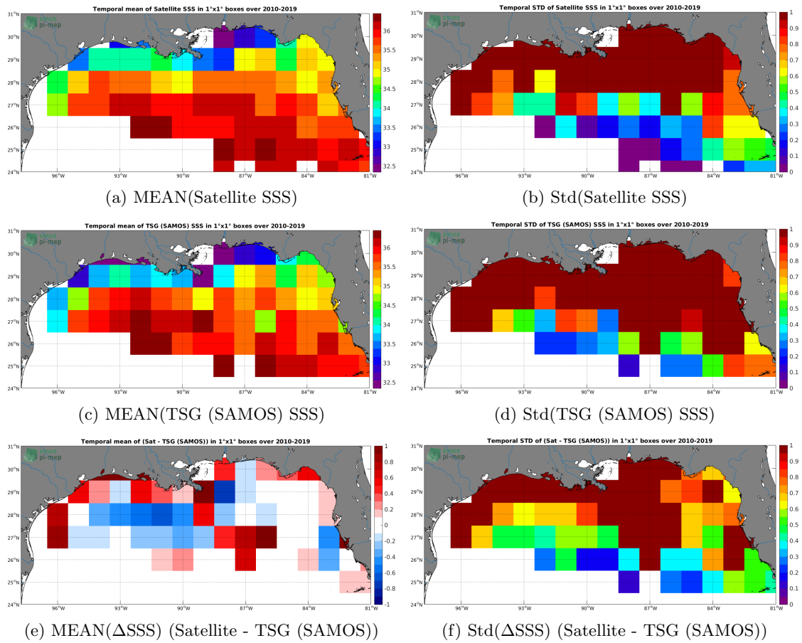
Figure 6: Temporal mean (left) and Std (right) of SSS from CCI L4 Merged-OI v2.31 - 7-day running (ESA) (top), TSG (SAMOS) (middle), and of \Delta SSS (Satellite - TSG (SAMOS)). Only match-up pairs are used to generate these maps.
