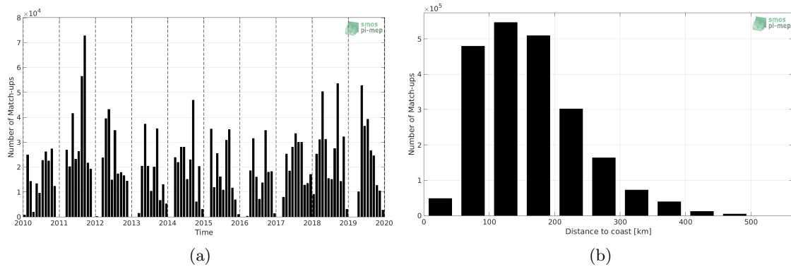
Figure 1: Number of match-ups between TSG (SAMOS) and CCI L4 Merged-OI v2.31 - 7-day running (ESA) SSS as a function of time (a) and as function of the distance to coast (b) over the Mississippi river plume Pi-MEP region and for the full satellite product period.
