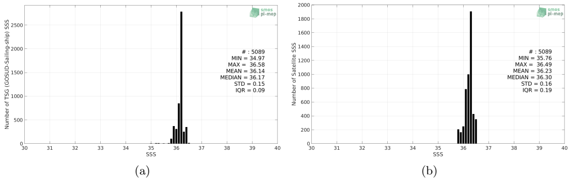
Figure 2: Histograms of SSS from TSG (GOSUD-Sailing-ship) (a) and CCI SSS L4 Merged-OI v2.31 - 7-day running (ESA) (b) considering all match-up pairs per bins of 0.1 over the Mississippi river plume Pi-MEP region and for the full satellite product period.
