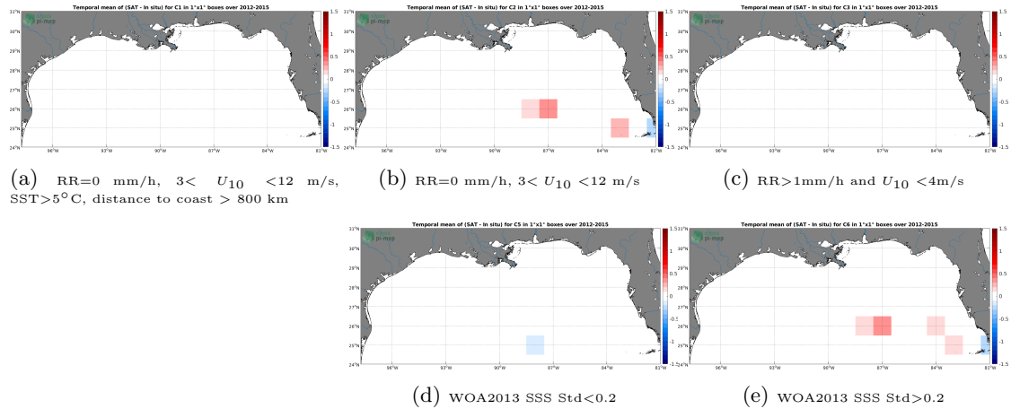
Figure 12: Temporal mean gridded over spatial boxes of size 1^{\circ}\times 1^{\circ} of \Delta SSS (CCI SSS L4 Merged-OI v2.31 - 7-day running (ESA) - TSG (GOSUD-Sailing-ship)) for 5 different subdatasets corresponding to:RR=0 mm/h, 3 < U_{10} < 12 m/s, SST >5^{\circ}\text{C} , distance to coast > 800 km (a), RR=0 mm/h, 3 < U_{10} < 12 m/s (b), RR >1 mm/h and U_{10} < 4 m/s (c), WOA2013 SSS Std <0.2 (d), WOA2013 SSS Std >0.2 (e).
