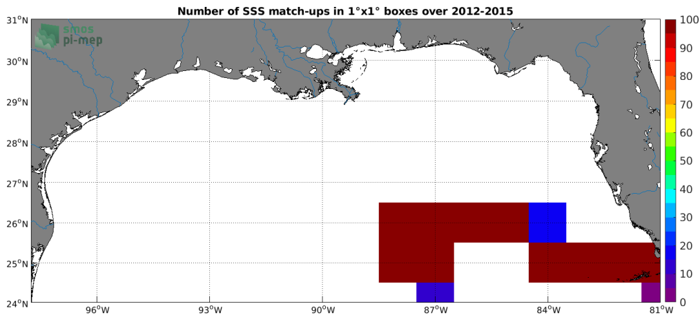
Figure 4: Number of SSS match-ups between TSG (GOSUD-Sailing-ship) SSS and the CCI SSS L4 Merged-OI v2.31 - 7-day running (ESA) SSS product for the Mississippi river plume Pi-MEP region over 1°x1° boxes and for the full satellite product period.
