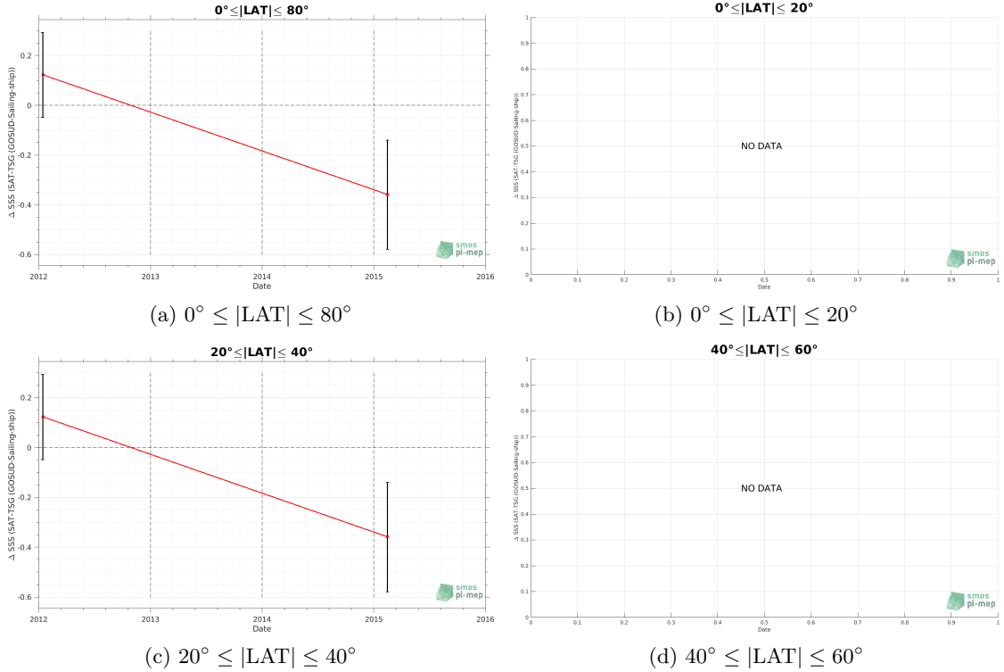
Figure 10: Monthly median (red curves) of \Delta SSS (Satellite - in situ ) between CCI SSS L4 Merged-OI v2.31 - 7-day running (ESA) and TSG (GOSUD-Sailing-ship) SSS as function of time for all the collected Pi-MEP match-up pairs estimated over the Mississippi river plume Pi-MEP region and for the full satellite product period are shown for different latitude bands: (a) 80^\circ\text{S}-80^\circ\text{N} , (b) 20^\circ\text{S}-20^\circ\text{N} , (c) 40^\circ\text{S}-20^\circ\text{S} and 20^\circ\text{N}-40^\circ\text{N} and (d) 60^\circ\text{S}-40^\circ\text{S} and 40^\circ\text{N}-60^\circ\text{N} .
