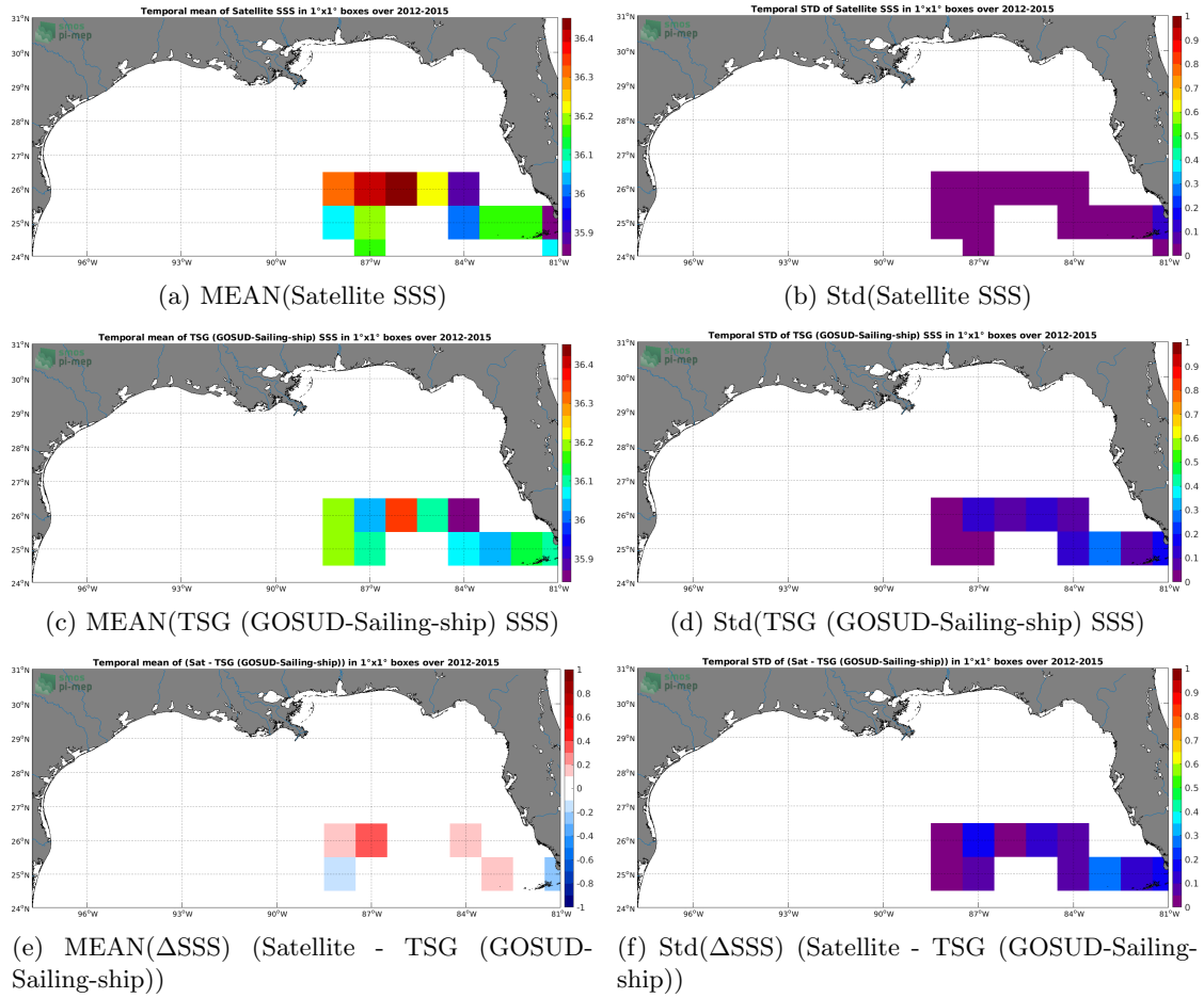
Figure 6: Temporal mean (left) and Std (right) of SSS from CCI SSS L4 Merged-OI v2.31 - 7-day running (ESA) (top), TSG (GOSUD-Sailing-ship) (middle), and of \Delta SSS (Satellite - TSG (GOSUD-Sailing-ship)). Only match-up pairs are used to generate these maps.
