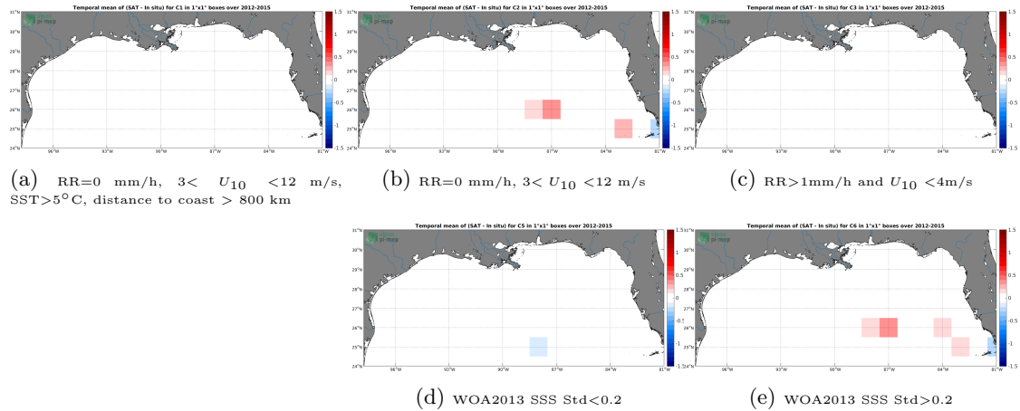
Figure 12: Temporal mean gridded over spatial boxes of size 1^\circ \times 1^\circ of \Delta SSS (CCI L4 Merged-OI v2.31 - 7-day running (ESA) - TSG (GOSUD-Sailing-ship)) for 5 different subdatasets corresponding to: RR=0 mm/h, 3 < U_{10} < 12 m/s, SST > 5^\circ\text{C} , distance to coast > 800 km (a), RR=0 mm/h, 3 < U_{10} < 12 m/s (b), RR > 1 mm/h and U_{10} < 4 m/s (c), WOA2013 SSS Std < 0.2 (d), WOA2013 SSS Std > 0.2 (e).
