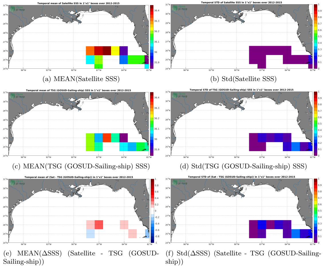
Figure 6: Temporal mean (left) and Std (right) of SSS from CCI L4 Merged-OI v2.31 - 7-day running (ESA) (top), TSG (GOSUD-Sailing-ship) (middle), and of \Delta SSS (Satellite - TSG (GOSUD-Sailing-ship)). Only match-up pairs are used to generate these maps.
