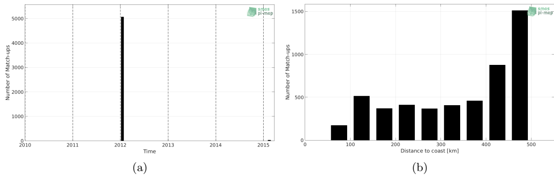
Figure 1: Number of match-ups between TSG (GOSUD-Sailing-ship) and CCI L4 Merged-OI v2.31 - 7-day running (ESA) SSS as a function of time (a) and as function of the distance to coast (b) over the Mississippi river plume Pi-MEP region and for the full satellite product period.
