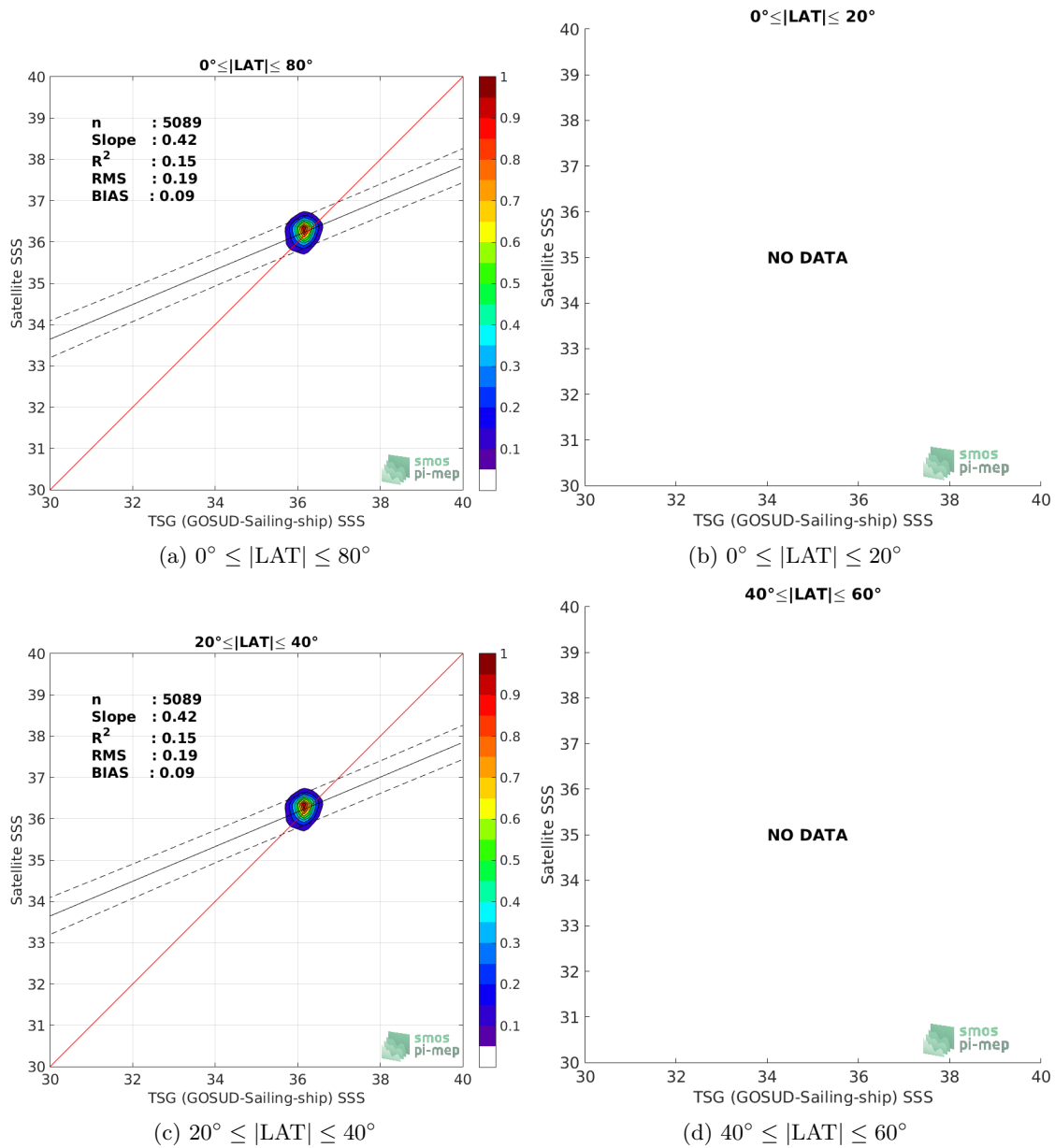
Figure 9: Contour maps of the concentration of CCI L4 Merged-OI v2.31 - 7-day running (ESA) SSS (y-axis) versus TSG (GOSUD-Sailing-ship) SSS (x-axis) at match-up pairs for different latitude bands. For each plot, the red line shows x=y . The black thin and dashed lines indicate a linear fit through the data cloud and the \pm 95\% confidence levels, respectively. The number match-up pairs n , the slope and R^2 coefficient of the linear fit, the root mean square (RMS) and the mean bias between satellite and in situ data are indicated for each latitude band in each plots.
