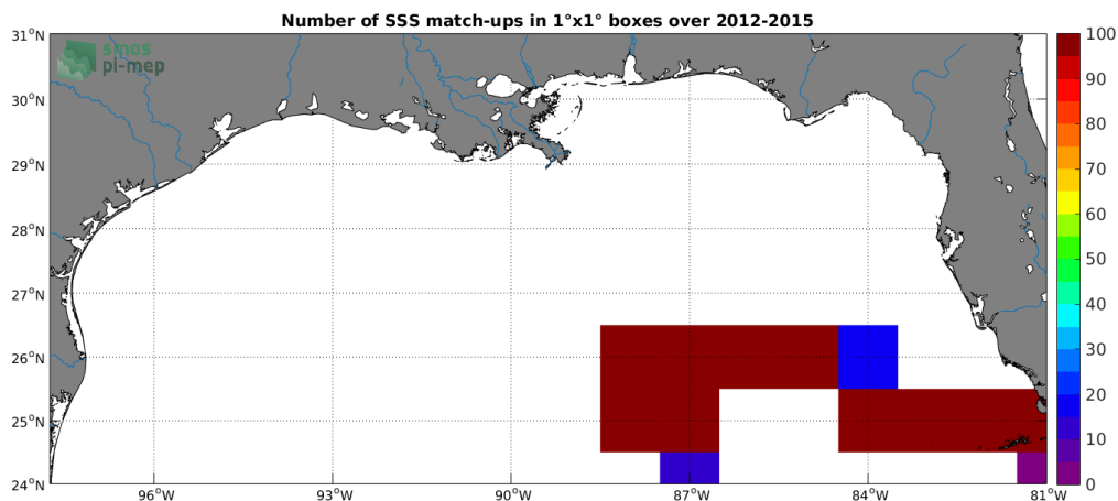
Figure 4: Number of SSS match-ups between TSG (GOSUD-Sailing-ship) SSS and the CCI L4 Merged-OI v2.31 - 7-day running (ESA) SSS product for the Mississippi river plume Pi-MEP region over 1°x1° boxes and for the full satellite product period.
