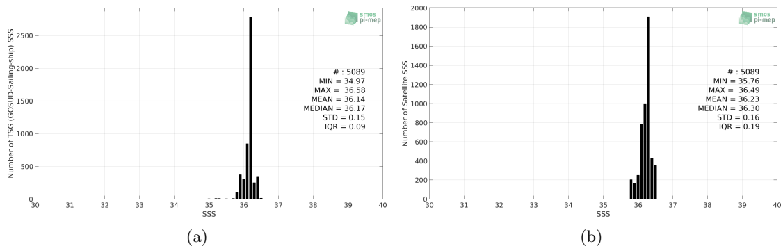
Figure 2: Histograms of SSS from TSG (GOSUD-Sailing-ship) (a) and CCI L4 Merged-OI v2.31 - 7-day running (ESA) (b) considering all match-up pairs per bins of 0.1 over the Mississippi river plume Pi-MEP region and for the full satellite product period.
