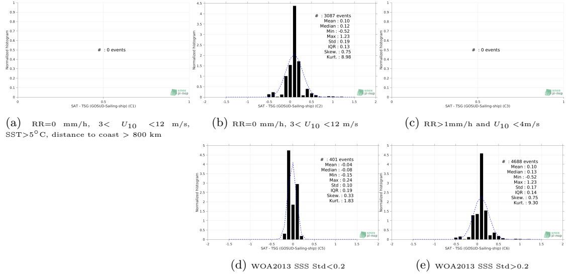
Figure 13: Normalized histogram of \Delta\text{SSS} (CCI L4 Merged-OI v2.31 - 7-day running (ESA) - TSG (GOSUD-Sailing-ship)) for 5 different subdatasets corresponding to: RR=0 mm/h, 3 < U_{10} < 12 m/s, SST > 5^\circ\text{C} , distance to coast > 800 km (a), RR=0 mm/h, 3 < U_{10} < 12 m/s (b), RR > 1\text{mm/h} and U_{10} < 4\text{m/s} (c), WOA2013 SSS Std < 0.2 (d), WOA2013 SSS Std > 0.2 (e).
