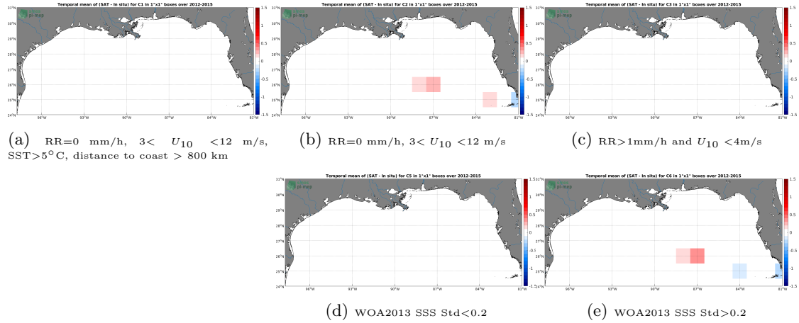
Figure 12: Temporal mean gridded over spatial boxes of size 1^\circ \times 1^\circ of \Delta SSS (CCI SSS L4 Merged-OI v2.31 - 30-day running (ESA) - TSG (GOSUD-Sailing-ship)) for 5 different subdatasets corresponding to: RR=0 mm/h, 3 < U_{10} < 12 m/s, SST >5^\circ\text{C} , distance to coast > 800 km (a), RR=0 mm/h, 3 < U_{10} < 12 m/s (b), RR >1 mm/h and U_{10} < 4 m/s (c), WOA2013 SSS Std <0.2 (d), WOA2013 SSS Std >0.2 (e).
