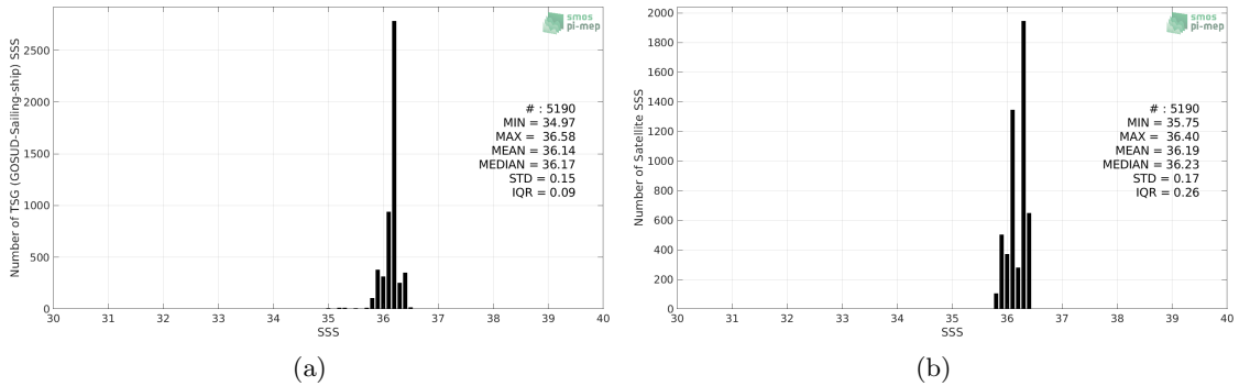
Figure 2: Histograms of SSS from TSG (GOSUD-Sailing-ship) (a) and CCI SSS L4 Merged-OI v2.31 - 30-day running (ESA) (b) considering all match-up pairs per bins of 0.1 over the Mississippi river plume Pi-MEP region and for the full satellite product period.
