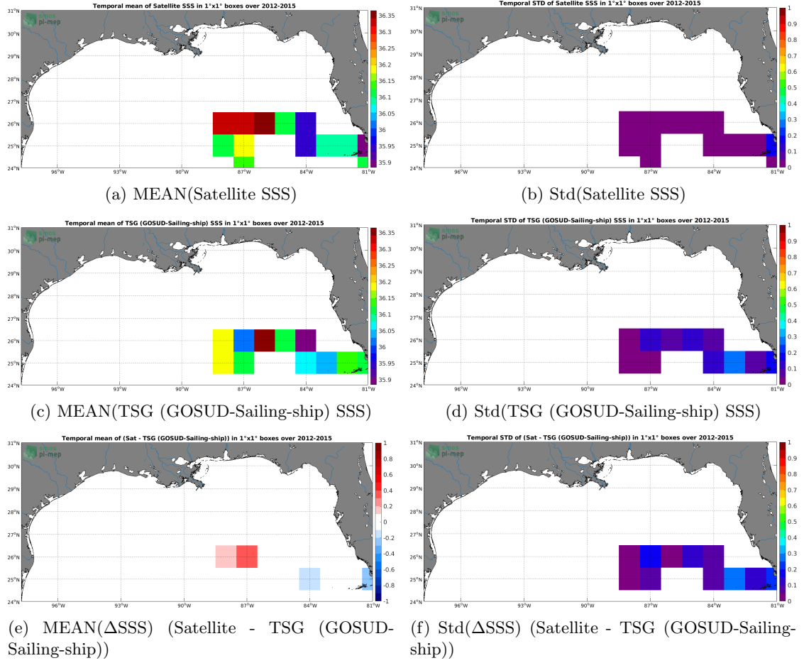
Figure 6: Temporal mean (left) and Std (right) of SSS from CCI SSS L4 Merged-OI v2.31 - 30-day running (ESA) (top), TSG (GOSUD-Sailing-ship) (middle), and of \Delta SSS (Satellite - TSG (GOSUD-Sailing-ship)). Only match-up pairs are used to generate these maps.
