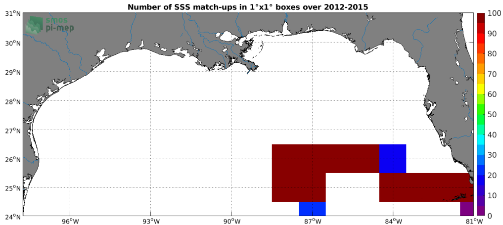
Figure 4: Number of SSS match-ups between TSG (GOSUD-Sailing-ship) SSS and the CCI SSS L4 Merged-OI v2.31 - 30-day running (ESA) SSS product for the Mississippi river plume Pi-MEP region over 1^\circ \times 1^\circ boxes and for the full satellite product period.
