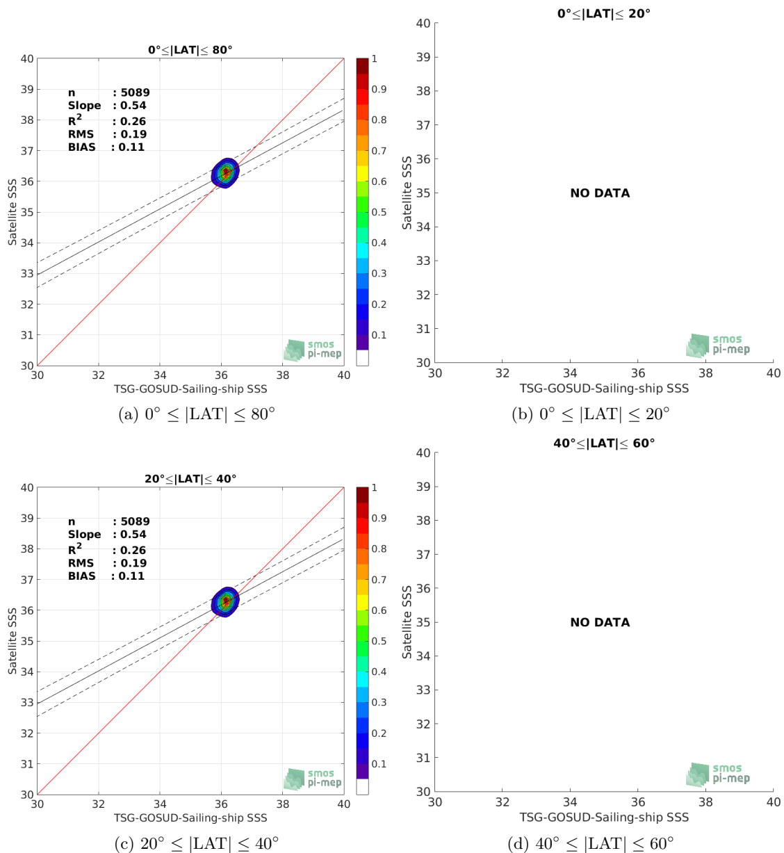
Figure 9: Contour maps of the concentration of CCI L4 Merged-OI v1.8 - 7-day running (ESA) SSS (y-axis) versus TSG-GOSUD-Sailing-ship SSS (x-axis) at match-up pairs for different latitude bands. For each plot, the red line shows x=y . The black thin and dashed lines indicate a linear fit through the data cloud and the \pm 95\% confidence levels, respectively. The number match-up pairs n , the slope and R^2 coefficient of the linear fit, the root mean square (RMS) and the mean bias between satellite and in situ data are indicated for each latitude band in each plots.
