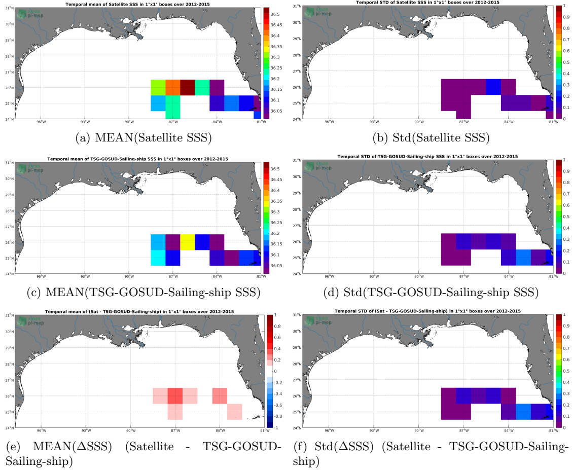
Figure 6: Temporal mean (left) and Std (right) of SSS from CCI L4 Merged-OI v1.8 - 7-day running (ESA) (top), TSG-GOSUD-Sailing-ship (middle), and of \Delta SSS (Satellite - TSG-GOSUD-Sailing-ship). Only match-up pairs are used to generate these maps.
