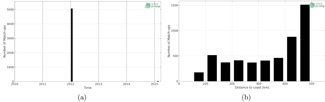
Figure 1: Number of match-ups between TSG-GOSUD-Sailing-ship and CCI L4 Merged-OI v1.8 - 7-day running (ESA) SSS as a function of time (a) and as function of the distance to coast (b) over the Mississippi river plume Pi-MEP region and for the full satellite product period.
