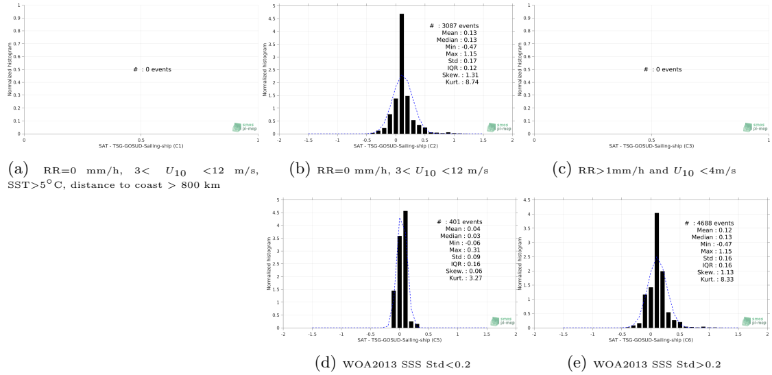
Figure 13: Normalized histogram of \Delta SSS (CCI L4 Merged-OI v1.8 - 7-day running (ESA) - TSG-GOSUD-Sailing-ship) for 5 different subdatasets corresponding to: RR=0 mm/h, 3 < U_{10} < 12 m/s, SST > 5°C, distance to coast > 800 km (a), RR=0 mm/h, 3 < U_{10} < 12 m/s (b), RR > 1mm/h and U_{10} < 4 m/s (c), WOA2013 SSS Std < 0.2 (d), WOA2013 SSS Std > 0.2 (e).
