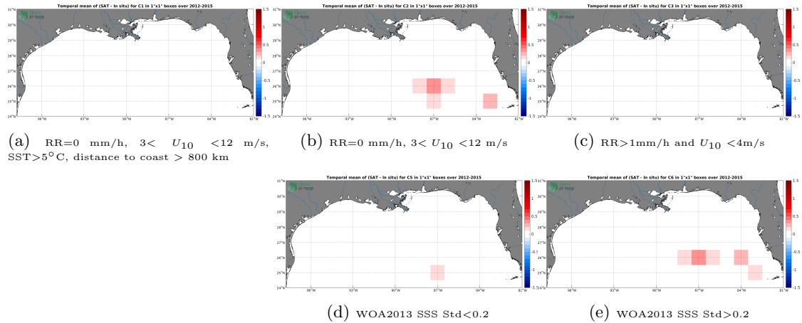
Figure 12: Temporal mean gridded over spatial boxes of size 1^{\circ}\times 1^{\circ} of \Delta SSS (CCI L4 Merged-OI v1.8 - 7-day running (ESA) - TSG-GOSUD-Sailing-ship) for 5 different subdatasets corresponding to:RR=0 mm/h, 3 < U_{10} < 12 m/s, SST >5^{\circ}\text{C} , distance to coast > 800 km (a), RR=0 mm/h, 3 < U_{10} < 12 m/s (b), RR >1 mm/h and U_{10} < 4 m/s (c), WOA2013 SSS Std <0.2 (d), WOA2013 SSS Std >0.2 (e).
