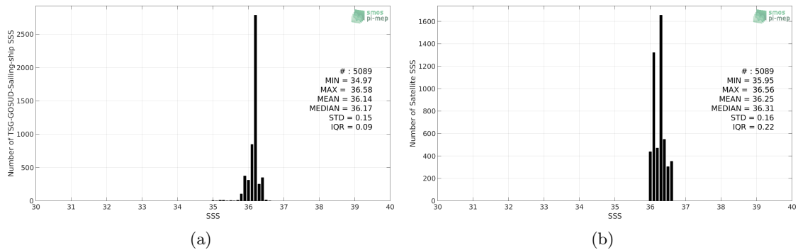
Figure 2: Histograms of SSS from TSG-GOSUD-Sailing-ship (a) and CCI L4 Merged-OI v1.8 - 7-day running (ESA) (b) considering all match-up pairs per bins of 0.1 over the Mississippi river plume Pi-MEP region and for the full satellite product period.
