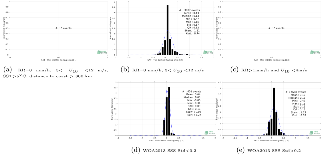
Figure 13: Normalized histogram of \Delta SSS (CCI-L4-ESA-MERGED-OI-V1.8-7DAY-RUNNING - TSG-GOSUD-Sailing-ship) for 5 different subdatasets corresponding to: RR=0 mm/h, 3 < U_{10} < 12 m/s, SST > 5°C, distance to coast > 800 km (a), RR=0 mm/h, 3 < U_{10} < 12 m/s (b), RR > 1mm/h and U_{10} < 4 m/s (c), WOA2013 SSS Std < 0.2 (d), WOA2013 SSS Std > 0.2 (e).
