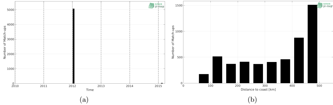
Figure 1: Number of match-ups between TSG-GOSUD-Sailing-ship and CCI-L4-ESA-MERGED-OI-V1.8-7DAY-RUNNING SSS as a function of time (a) and as function of the distance to coast (b) over the Mississippi river plume Pi-MEP region and for the full satellite product period.
