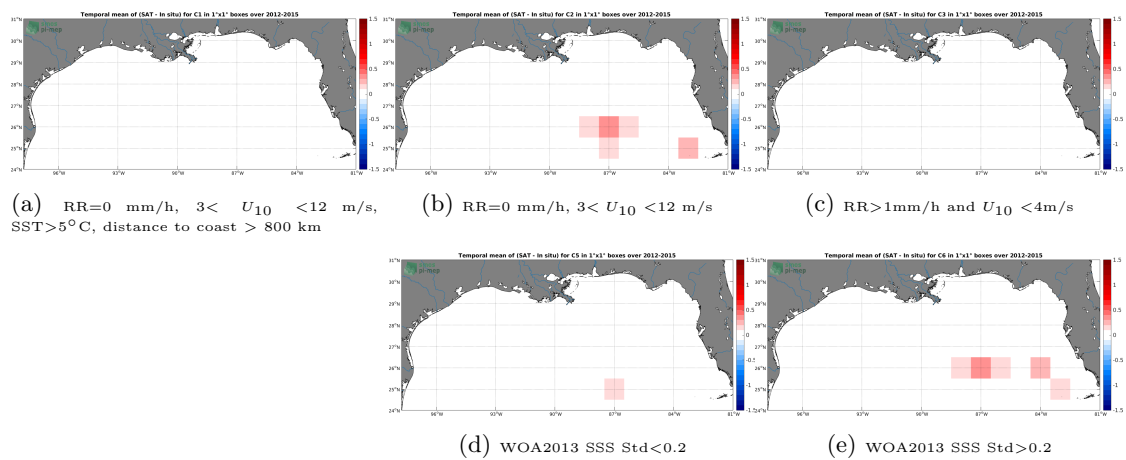
Figure 12: Temporal mean gridded over spatial boxes of size 1^\circ \times 1^\circ of \Delta SSS (CCI-L4-ESAMERGED-OI-V1.8-7DAY-RUNNING - TSG-GOSUD-Sailing-ship) for 5 different subdatasets corresponding to: RR=0 mm/h, 3 < U_{10} < 12 m/s, SST > 5°C, distance to coast > 800 km (a), RR=0 mm/h, 3 < U_{10} < 12 m/s (b), RR > 1mm/h and U_{10} < 4 m/s (c), WOA2013 SSS Std < 0.2 (d), WOA2013 SSS Std > 0.2 (e).
