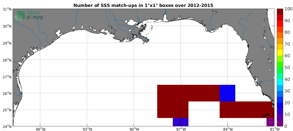
Figure 4: Number of SSS match-ups between TSG-GOSUD-Sailing-ship SSS and the CCI-L4-ESA-MERGED-OI-V1.8-7DAY-RUNNING SSS product for the Mississippi river plume Pi-MEP region over 1^\circ \times 1^\circ boxes and for the full satellite product period.
