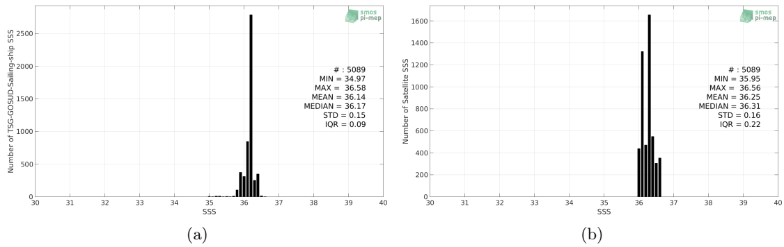
Figure 2: Histograms of SSS from TSG-GOSUD-Sailing-ship (a) and CCI-L4-ESA-MERGED-OI-V1.8-7DAY-RUNNING (b) considering all match-up pairs per bins of 0.1 over the Mississippi river plume Pi-MEP region and for the full satellite product period.
