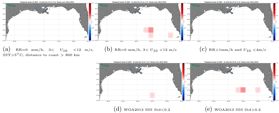
Figure 12: Temporal mean gridded over spatial boxes of size 1^{\circ}\times 1^{\circ} of \Delta SSS (CCI L4 Merged-OI v1.8 - 30-day running (ESA) - TSG-GOSUD-Sailing-ship) for 5 different subdatasets corresponding to:RR=0 mm/h, 3 < U_{10} < 12 m/s, SST >5^{\circ}\text{C} , distance to coast > 800 km (a), RR=0 mm/h, 3 < U_{10} < 12 m/s (b), RR >1 mm/h and U_{10} < 4 m/s (c), WOA2013 SSS Std <0.2 (d), WOA2013 SSS Std >0.2 (e).
