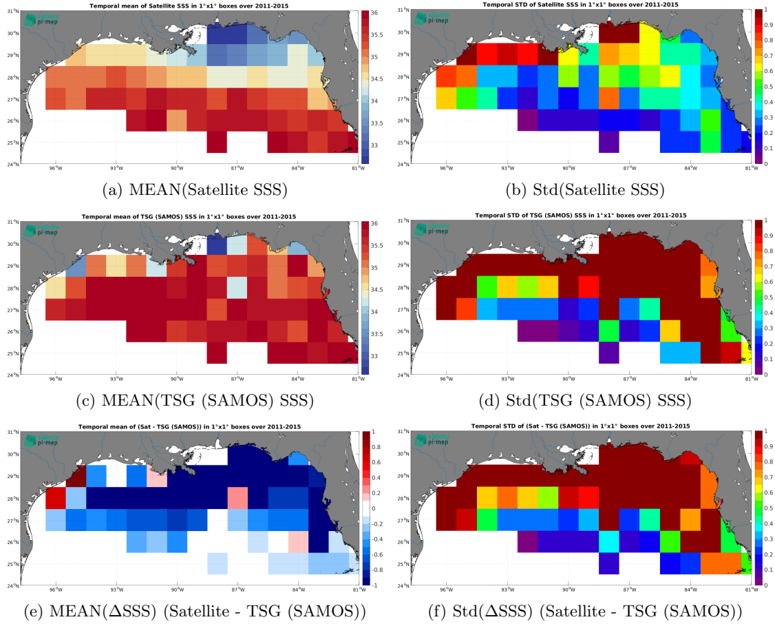
Figure 7: Temporal mean (left) and Std (right) of SSS from Aquarius SSS L4 OI v5 - Weekly (IPRC) (top), TSG (SAMOS) (middle), and of \Delta\text{SSS} (Satellite - TSG (SAMOS)). Only match-up pairs are used to generate these maps.
