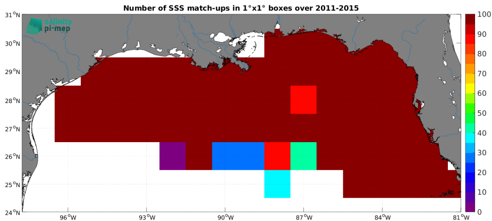
Figure 5: Number of SSS match-ups between TSG (SAMOS) SSS and the Aquarius SSS L4 OI v5 - Weekly (IPRC) SSS product for the Mississippi river plume Pi-MEP region over 1^\circ \times 1^\circ boxes and for the full satellite product period.
