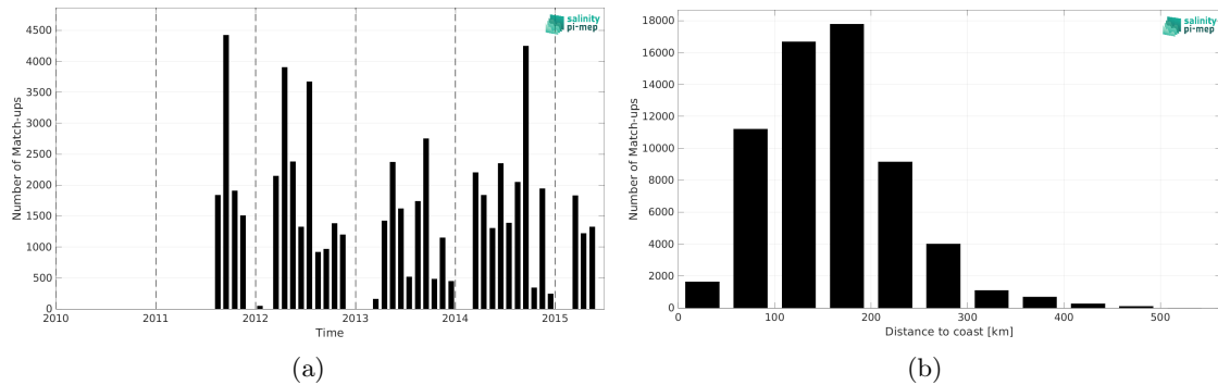
Figure 2: Number of match-ups between TSG (SAMOS) and Aquarius SSS L4 OI v5 - Weekly (IPRC) SSS as a function of time (a) and as function of the distance to coast (b) over the Mississippi river plume Pi-MEP region and for the full satellite product period.
