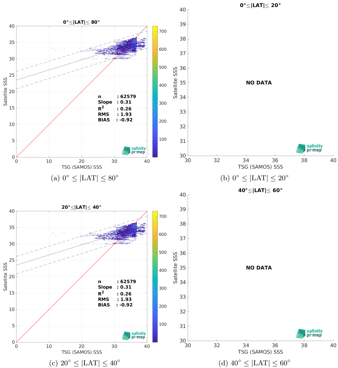
Figure 10: Contour maps of the concentration of Aquarius SSS L4 OI v5 - Weekly (IPRC) SSS (y-axis) versus TSG (SAMOS) SSS (x-axis) at match-up pairs for different latitude bands. For each plot, the red line shows x=y . The black thin and dashed lines indicate a linear fit through the data cloud and the \pm 95\% confidence levels, respectively. The number match-up pairs n , the slope and R^2 coefficient of the linear fit, the root mean square (RMS) and the mean bias between satellite and in situ data are indicated for each latitude band in each plots.
