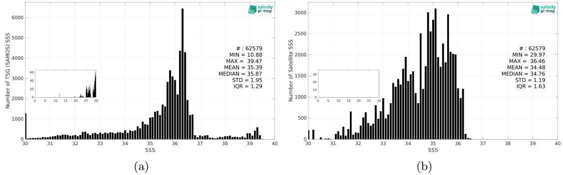
Figure 3: Histograms of SSS from TSG (SAMOS) (a) and Aquarius SSS L4 OI v5 - Weekly (IPRC) (b) considering all match-up pairs per bins of 0.1 over the Mississippi river plume Pi-MEP region and for the full satellite product period.
