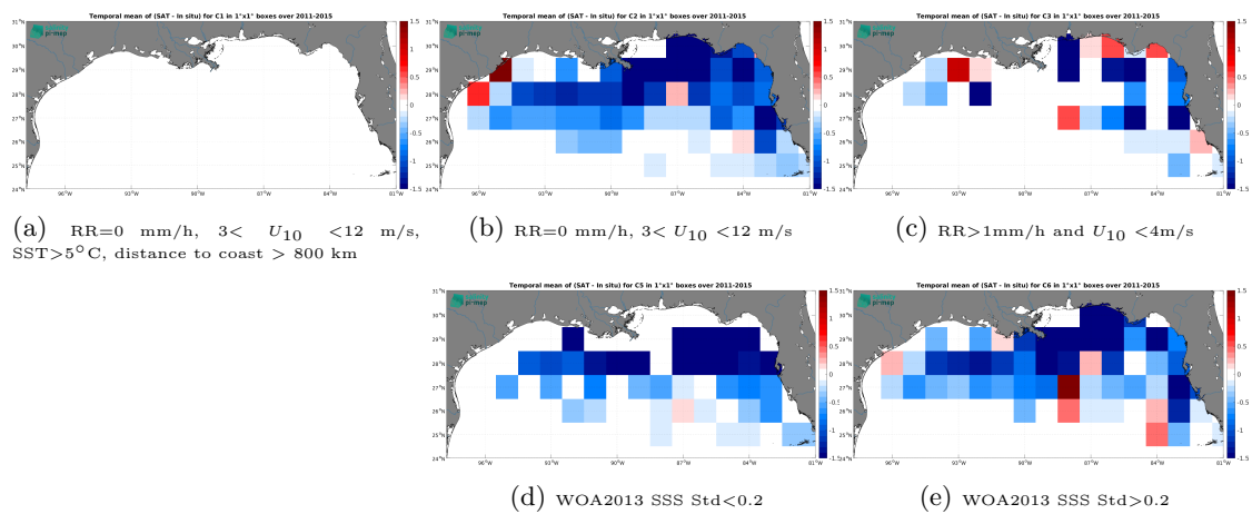
Figure 14: Temporal mean gridded over spatial boxes of size 1^\circ \times 1^\circ of \Delta SSS (Aquarius SSS L4 OI v5 - Weekly (IPRC) - TSG (SAMOS)) for 5 different subdatasets corresponding to:RR=0 mm/h, 3 < U_{10} < 12 m/s, SST >5^\circ C, distance to coast > 800 km (a), RR=0 mm/h, 3 < U_{10} < 12 m/s (b), RR >1 mm/h and U_{10} < 4 m/s (c), WOA2013 SSS Std <0.2 (d), WOA2013 SSS Std >0.2 (e).
