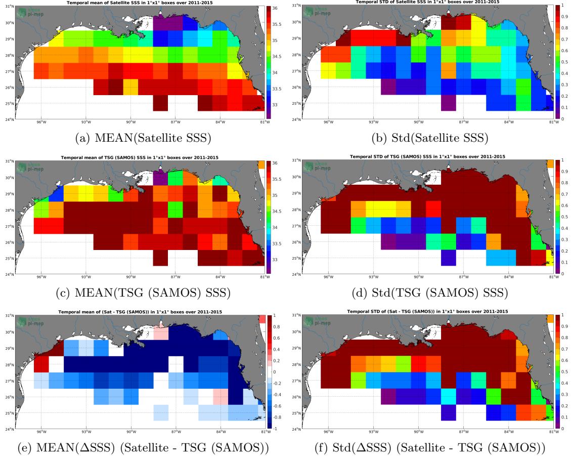
Figure 6: Temporal mean (left) and Std (right) of SSS from Aquarius SSS L4 OI v5 - Weekly (IPRC) (top), TSG (SAMOS) (middle), and of \Delta\text{SSS} (Satellite - TSG (SAMOS)). Only match-up pairs are used to generate these maps.
