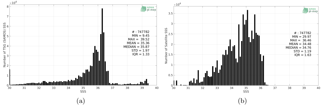
Figure 2: Histograms of SSS from TSG (SAMOS) (a) and Aquarius SSS L4 OI v5 - Weekly (IPRC) (b) considering all match-up pairs per bins of 0.1 over the Mississippi river plume Pi-MEP region and for the full satellite product period.
