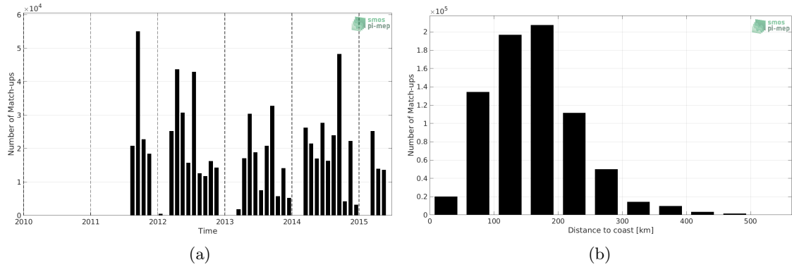
Figure 1: Number of match-ups between TSG (SAMOS) and Aquarius SSS L4 OI v5 - Weekly (IPRC) SSS as a function of time (a) and as function of the distance to coast (b) over the Mississippi river plume Pi-MEP region and for the full satellite product period.
