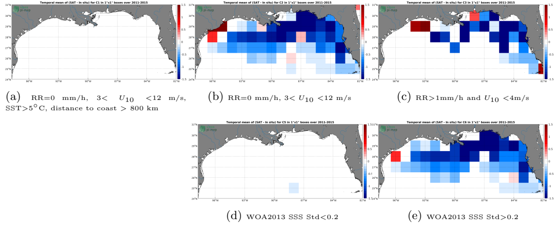
Figure 12: Temporal mean gridded over spatial boxes of size 1^{\circ}\times 1^{\circ} of \Delta\text{SSS} (Aquarius SSS L4 OI v5 - Weekly (IPRC) - TSG (SAMOS)) for 5 different subdatasets corresponding to: \text{RR}=0 mm/h, 3 < U_{10} < 12 m/s, \text{SST} > 5^{\circ}\text{C} , distance to coast > 800 km (a), \text{RR}=0 mm/h, 3 < U_{10} < 12 m/s (b), \text{RR} > 1 mm/h and U_{10} < 4 m/s (c), WOA2013 SSS Std < 0.2 (d), WOA2013 SSS Std > 0.2 (e).
