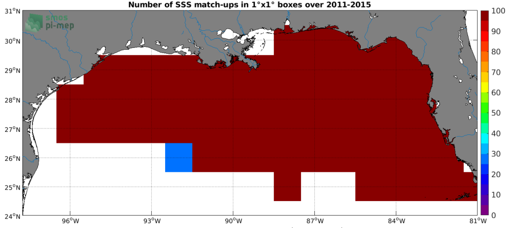
Figure 4: Number of SSS match-ups between TSG (SAMOS) SSS and the Aquarius SSS L4 OI v5 - Weekly (IPRC) SSS product for the Mississippi river plume Pi-MEP region over 1^\circ \times 1^\circ boxes and for the full satellite product period.
