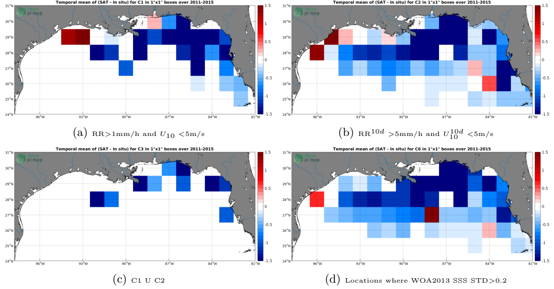
Figure 12: Temporal mean gridded over spatial boxes of size 1^\circ \times 1^\circ of \Delta SSS (Aquarius-L4-IPRC-V5-WEEKLY - TSG-SAMOS) for 4 different subdatasets corresponding to: RR > 1\text{mm/h} and U_{10} < 5\text{m/s} (a), RR^{10d} > 5\text{mm/h} and U_{10}^{10d} < 5\text{m/s} (b), C1 \cup C2 (c), Locations where WOA2013 SSS STD > 0.2 (d).
