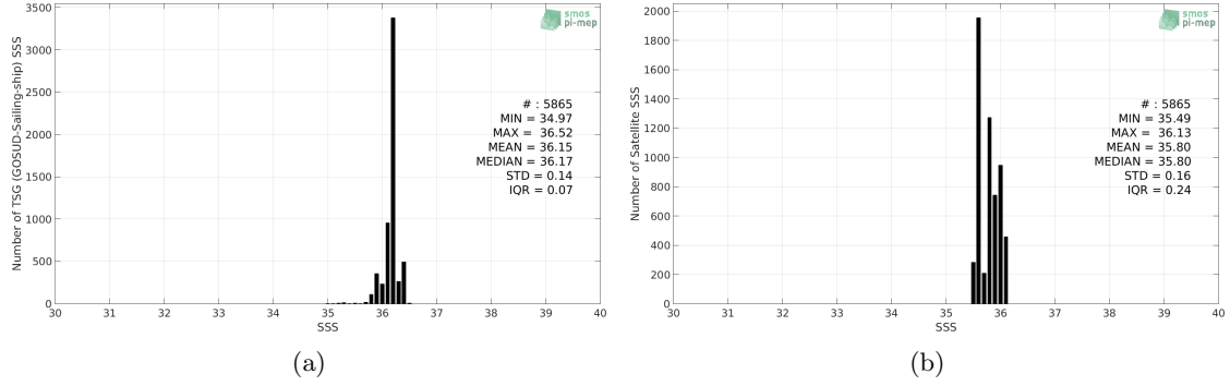
Figure 2: Histograms of SSS from TSG (GOSUD-Sailing-ship) (a) and Aquarius SSS L4 OI v5 - Weekly (IPRC) (b) considering all match-up pairs per bins of 0.1 over the Mississippi river plume Pi-MEP region and for the full satellite product period.
