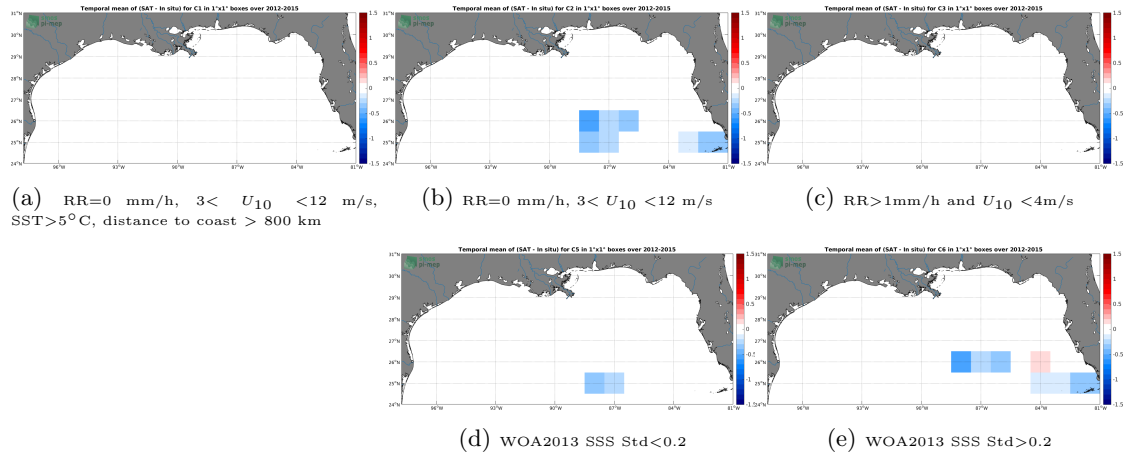
Figure 12: Temporal mean gridded over spatial boxes of size 1^\circ \times 1^\circ of \Delta SSS (Aquarius SSS L4 OI v5 - Weekly (IPRC) - TSG (GOSUD-Sailing-ship)) for 5 different subdatasets corresponding to: RR=0 mm/h, 3 < U_{10} < 12 m/s, SST > 5^\circ\text{C} , distance to coast > 800 km (a), RR=0 mm/h, 3 < U_{10} < 12 m/s (b), RR > 1 mm/h and U_{10} < 4 m/s (c), WOA2013 SSS Std < 0.2 (d), WOA2013 SSS Std > 0.2 (e).
