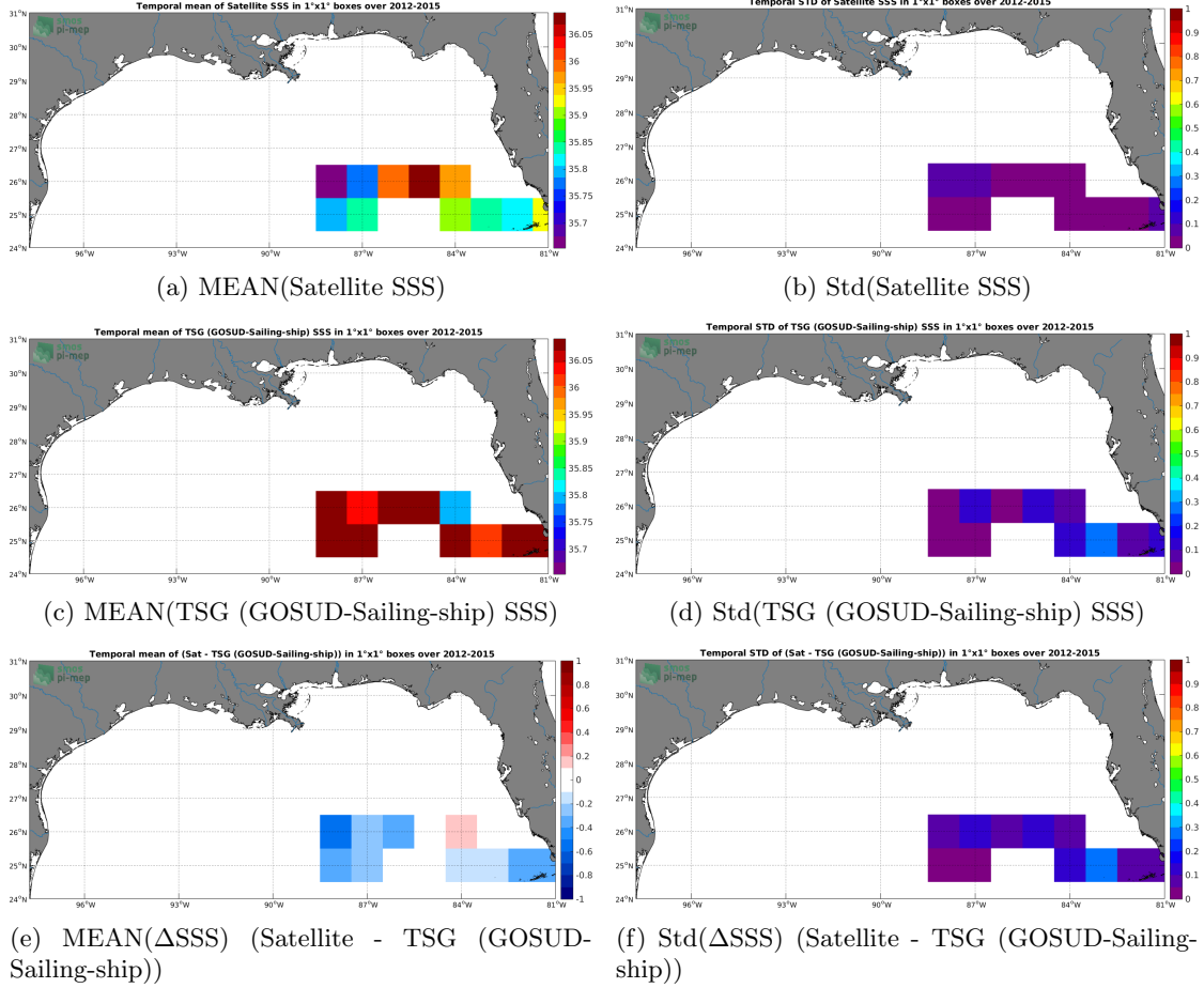
Figure 6: Temporal mean (left) and Std (right) of SSS from Aquarius SSS L4 OI v5 - Weekly (IPRC) (top), TSG (GOSUD-Sailing-ship) (middle), and of \Delta\text{SSS} (Satellite - TSG (GOSUD-Sailing-ship)). Only match-up pairs are used to generate these maps.
