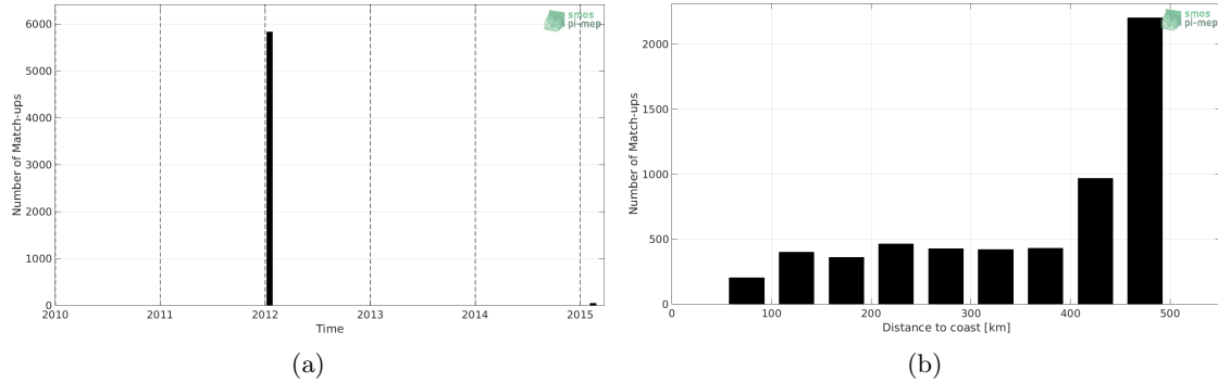
Figure 1: Number of match-ups between TSG (GOSUD-Sailing-ship) and Aquarius SSS L4 OI v5 - Weekly (IPRC) SSS as a function of time (a) and as function of the distance to coast (b) over the Mississippi river plume Pi-MEP region and for the full satellite product period.
