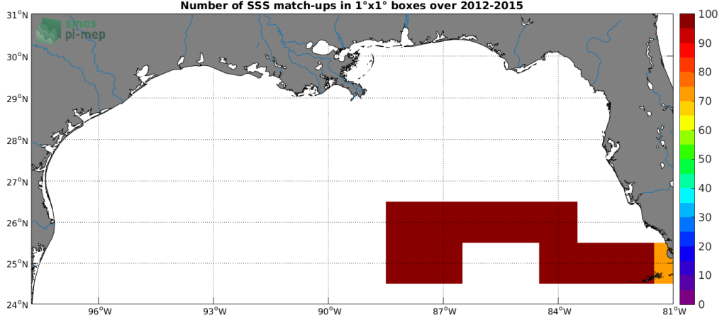
Figure 4: Number of SSS match-ups between TSG (GOSUD-Sailing-ship) SSS and the Aquarius SSS L4 OI v5 - Weekly (IPRC) SSS product for the Mississippi river plume Pi-MEP region over 1^\circ \times 1^\circ boxes and for the full satellite product period.
