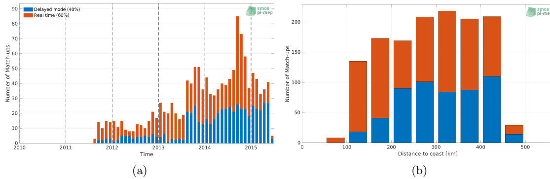
Figure 1: Number of match-ups between Argo and Aquarius SSS L4 OI v5 - Weekly (IPRC) SSS as a function of time (a) and as function of the distance to coast (b) over the Mississippi river plume Pi-MEP region and for the full satellite product period.
