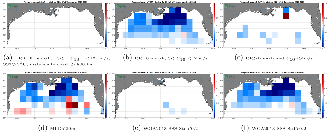
Figure 12: Temporal mean gridded over spatial boxes of size 1^{\circ} \times 1^{\circ} of \Delta\text{SSS} (Aquarius SSS L4 OI v5 - Weekly (IPRC) - Argo) for 6 different subdatasets corresponding to: \text{RR}=0 mm/h, 3 < U_{10} < 12 m/s, \text{SST} > 5^{\circ}\text{C} , distance to coast > 800 km (a), \text{RR}=0 mm/h, 3 < U_{10} < 12 m/s (b), \text{RR} > 1 mm/h and U_{10} < 4 m/s (c), \text{MLD} < 20\text{m} (d), \text{WOA2013 SSS Std} < 0.2 (e), \text{WOA2013 SSS Std} > 0.2 (f).
