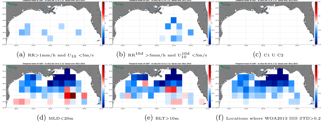
Figure 12: Temporal mean gridded over spatial boxes of size 1^\circ \times 1^\circ of \Delta SSS (Aquarius-L4-IPRC-V5-WEEKLY - Argo) for 6 different subdatasets corresponding to: RR > 1\text{mm/h} and U_{10} < 5\text{m/s} (a), RR^{10d} > 5\text{mm/h} and U_{10}^{10d} < 5\text{m/s} (b), C1 U C2 (c), MLD < 20\text{m} (d), BLT > 10\text{m} (e), Locations where WOA2013 SSS STD > 0.2 (f).
