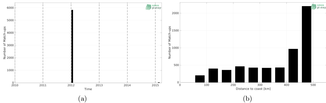
Figure 1: Number of match-ups between TSG (GOSUD-Sailing-ship) and Aquarius SSS L4 OI v5 - Monthly (IPRC) SSS as a function of time (a) and as function of the distance to coast (b) over the Mississippi river plume Pi-MEP region and for the full satellite product period.
