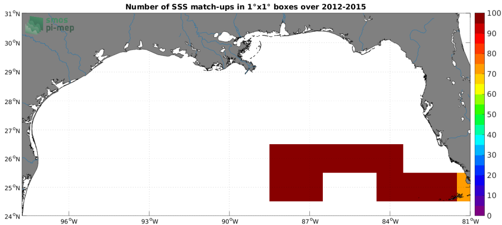
Figure 4: Number of SSS match-ups between TSG (GOSUD-Sailing-ship) SSS and the Aquarius SSS L4 OI v5 - Monthly (IPRC) SSS product for the Mississippi river plume Pi-MEP region over 1^\circ \times 1^\circ boxes and for the full satellite product period.
