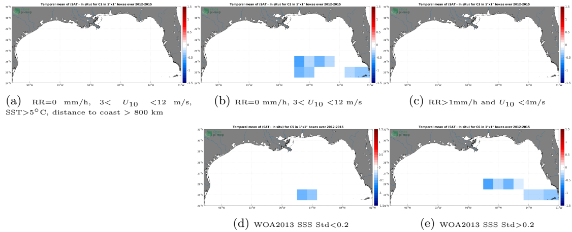
Figure 12: Temporal mean gridded over spatial boxes of size 1^{\circ}\times 1^{\circ} of \Delta SSS (Aquarius SSS L4 OI v5 - Monthly (IPRC) - TSG (GOSUD-Sailing-ship)) for 5 different subdatasets corresponding to: RR=0 mm/h, 3 < U_{10} < 12 m/s, SST > 5^{\circ}\text{C} , distance to coast > 800 km (a), RR=0 mm/h, 3 < U_{10} < 12 m/s (b), RR > 1 mm/h and U_{10} < 4 m/s (c), WOA2013 SSS Std < 0.2 (d), WOA2013 SSS Std > 0.2 (e).
