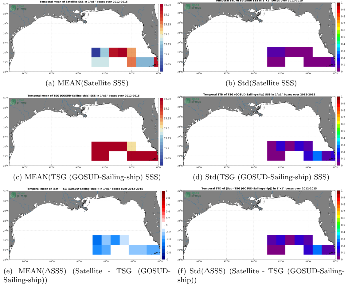
Figure 6: Temporal mean (left) and Std (right) of SSS from Aquarius SSS L4 OI v5 - Monthly (IPRC) (top), TSG (GOSUD-Sailing-ship) (middle), and of \Delta\text{SSS} (Satellite - TSG (GOSUD-Sailing-ship)). Only match-up pairs are used to generate these maps.
