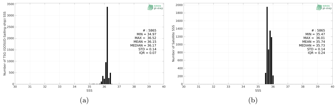
Figure 2: Histograms of SSS from TSG (GOSUD-Sailing-ship) (a) and Aquarius SSS L4 OI v5 - Monthly (IPRC) (b) considering all match-up pairs per bins of 0.1 over the Mississippi river plume Pi-MEP region and for the full satellite product period.
