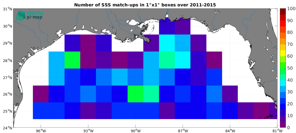
Figure 5: Number of SSS match-ups between Argo SSS and the Aquarius SSS L4 OI v5 - Monthly (IPRC) SSS product for the Mississippi river plume Pi-MEP region over 1^\circ \times 1^\circ boxes and for the full satellite product period.
