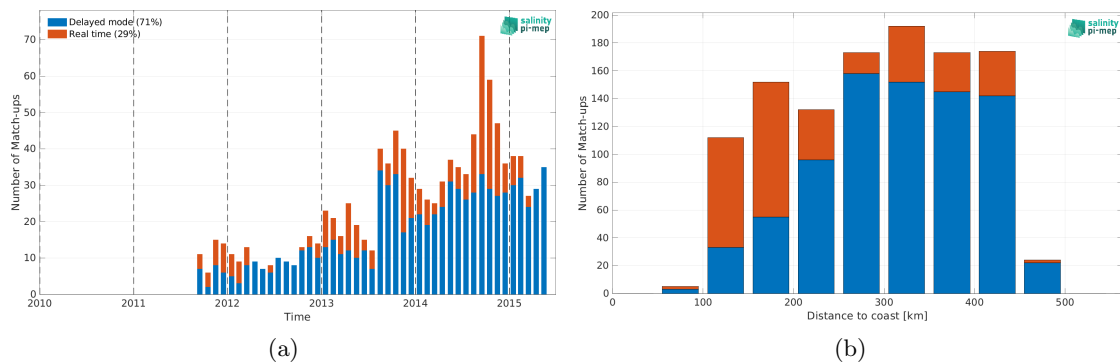
Figure 2: Number of match-ups between Argo and Aquarius SSS L4 OI v5 - Monthly (IPRC) SSS as a function of time (a) and as function of the distance to coast (b) over the Mississippi river plume Pi-MEP region and for the full satellite product period.
