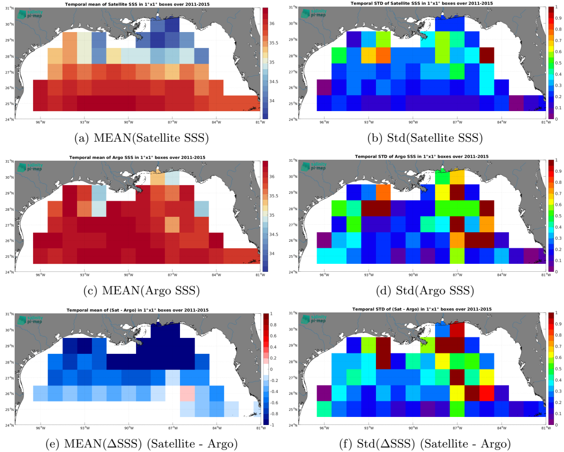
Figure 7: Temporal mean (left) and Std (right) of SSS from Aquarius SSS L4 OI v5 - Monthly (IPRC) (top), Argo (middle), and of \Delta\text{SSS} (Satellite - Argo). Only match-up pairs are used to generate these maps.
