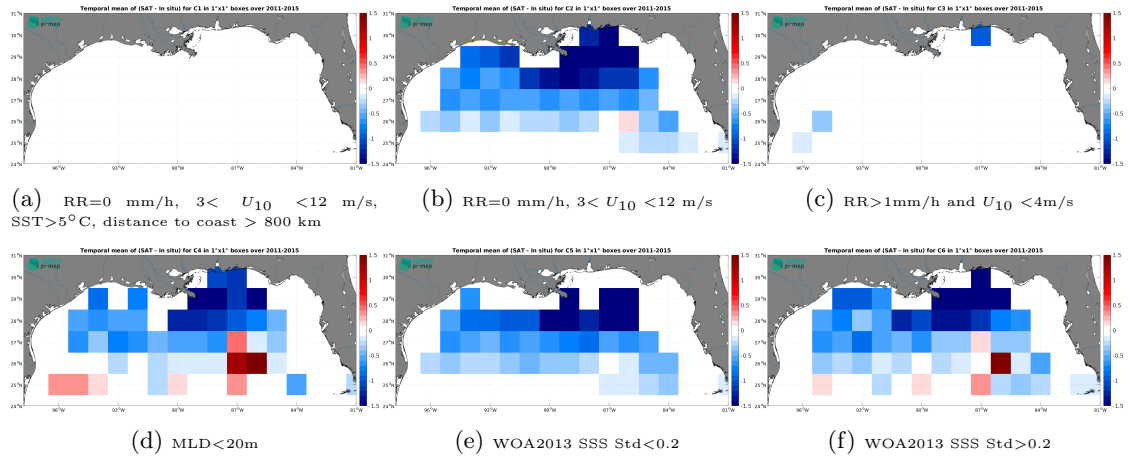
Figure 14: Temporal mean gridded over spatial boxes of size 1^\circ \times 1^\circ of \Delta SSS (Aquarius SSS L4 OI v5 - Monthly (IPRC) - Argo) for 6 different subdatasets corresponding to:RR=0 mm/h, 3 < U_{10} < 12 m/s, SST > 5°C, distance to coast > 800 km (a), RR=0 mm/h, 3 < U_{10} < 12 m/s (b), RR > 1mm/h and U_{10} < 4 m/s (c),MLD < 20m (d),WOA2013 SSS Std < 0.2 (e),WOA2013 SSS Std > 0.2 (f).
