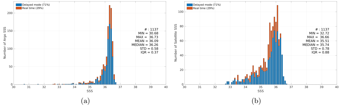
Figure 3: Histograms of SSS from Argo (a) and Aquarius SSS L4 OI v5 - Monthly (IPRC) (b) considering all match-up pairs per bins of 0.1 over the Mississippi river plume Pi-MEP region and for the full satellite product period.
