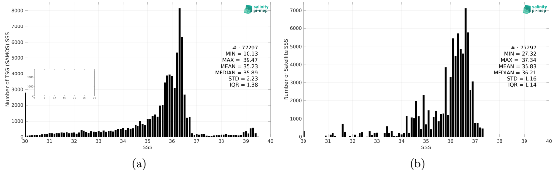
Figure 2: Histograms of SSS from TSG (SAMOS) (a) and Aquarius SSS L3 OR v5 - 7-Day running (NASA-GSFC) (b) considering all match-up pairs per bins of 0.1 over the Mississippi river plume Pi-MEP region and for the full satellite product period.
