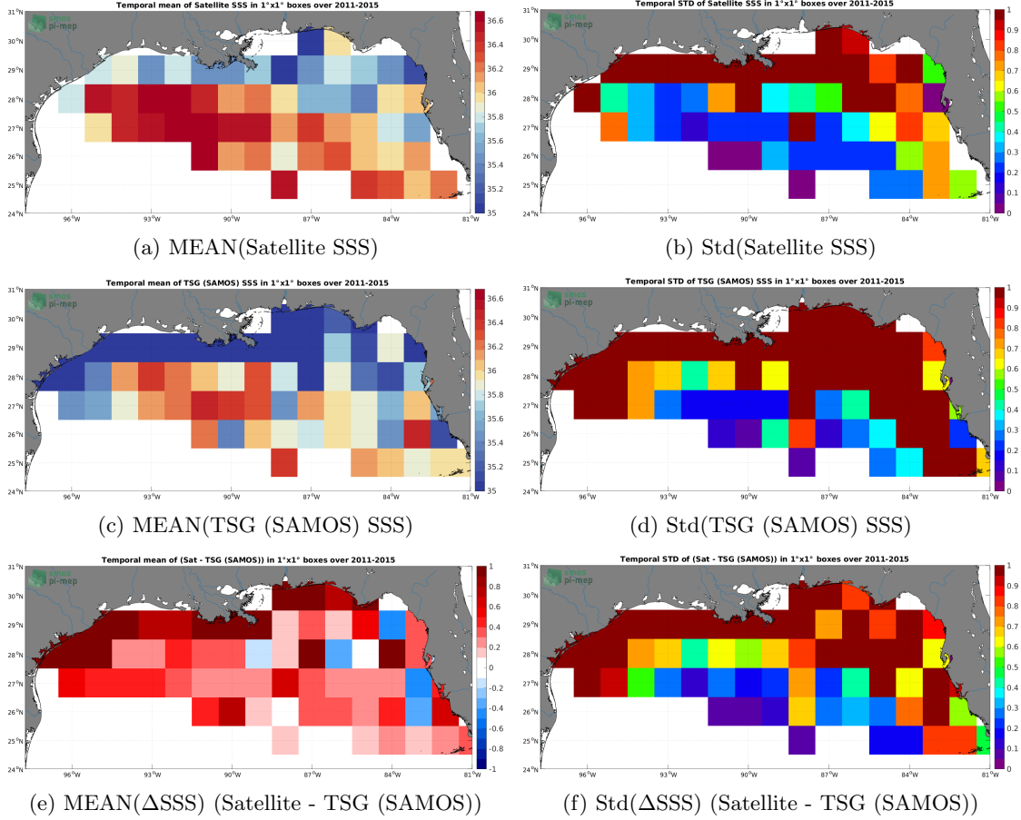
Figure 6: Temporal mean (left) and Std (right) of SSS from Aquarius SSS L3 OR v5 - 7-Day running (NASA-GSFC) (top), TSG (SAMOS) (middle), and of \Delta\text{SSS} (Satellite - TSG (SAMOS)). Only match-up pairs are used to generate these maps.
