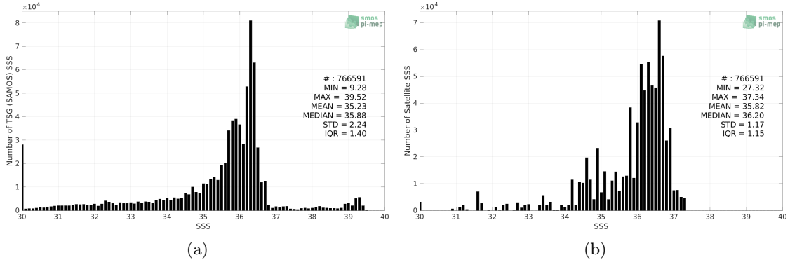
Figure 2: Histograms of SSS from TSG (SAMOS) (a) and Aquarius SSS L3 OR v5 - 7-Day running (NASA-GSFC) (b) considering all match-up pairs per bins of 0.1 over the Mississippi river plume Pi-MEP region and for the full satellite product period.
