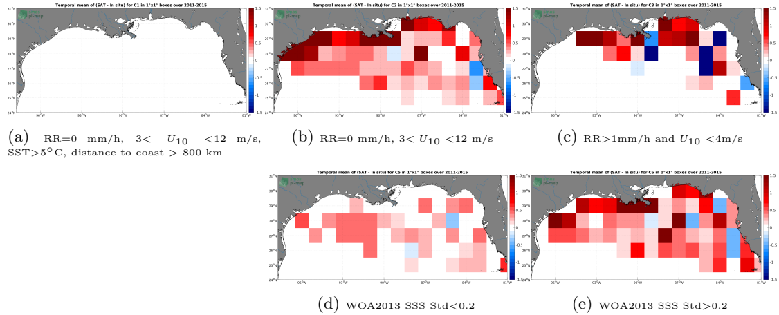
Figure 12: Temporal mean gridded over spatial boxes of size 1^{\circ}\times 1^{\circ} of \Delta\text{SSS} (Aquarius SSS L3 OR v5 - 7-Day running (NASA-GSFC) - TSG (SAMOS)) for 5 different subdatasets corresponding to:RR=0 mm/h, 3 < U_{10} < 12 m/s, SST >5^{\circ}\text{C} , distance to coast > 800 km (a), RR=0 mm/h, 3 < U_{10} < 12 m/s (b), RR >1 mm/h and U_{10} < 4 m/s (c), WOA2013 SSS Std <0.2 (d), WOA2013 SSS Std >0.2 (e).
