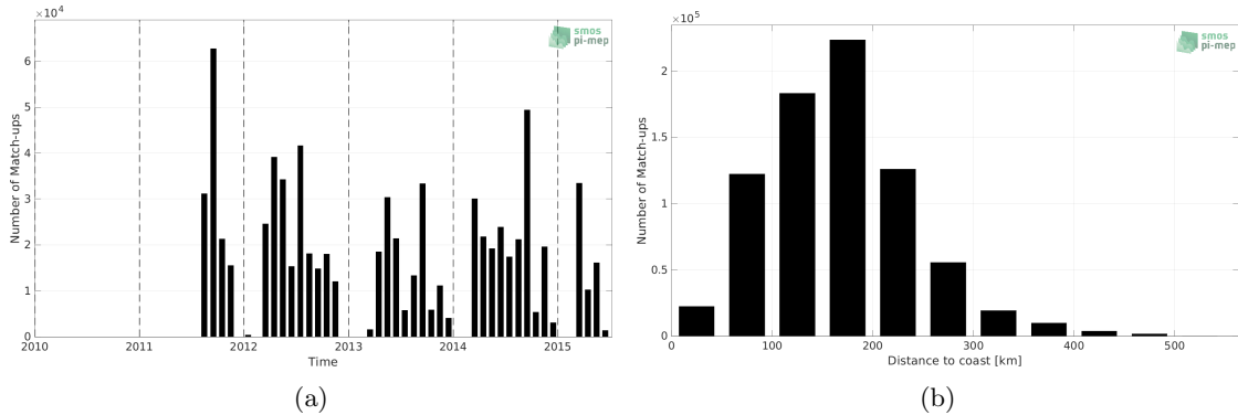
Figure 1: Number of match-ups between TSG (SAMOS) and Aquarius SSS L3 OR v5 - 7-Day running (NASA-GSFC) SSS as a function of time (a) and as function of the distance to coast (b) over the Mississippi river plume Pi-MEP region and for the full satellite product period.
