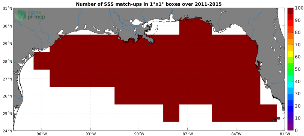
Figure 4: Number of SSS match-ups between TSG (SAMOS) SSS and the Aquarius SSS L3 OR v5 - 7-Day running (NASA-GSFC) SSS product for the Mississippi river plume Pi-MEP region over 1^\circ \times 1^\circ boxes and for the full satellite product period.
