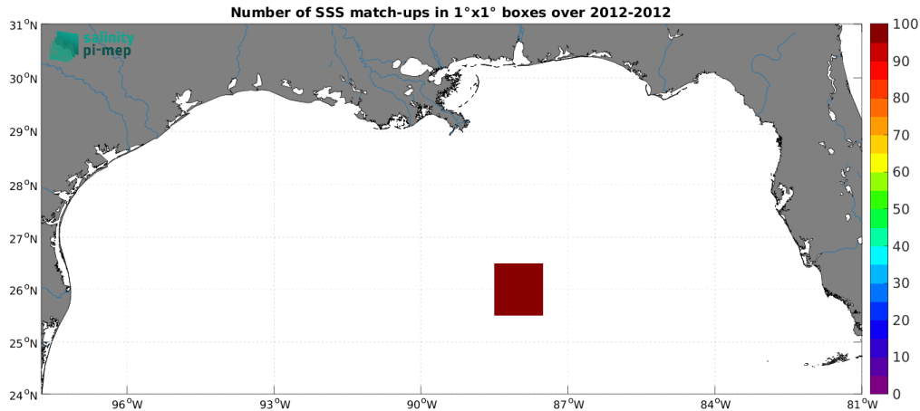
Figure 5: Number of SSS match-ups between TSG (GOSUD-Sailing-ship) SSS and the Aquarius SSS L3 OR v5 - 7-Day running (NASA-GSFC) SSS product for the Mississippi river plume Pi-MEP region over 1^\circ \times 1^\circ boxes and for the full satellite product period.
