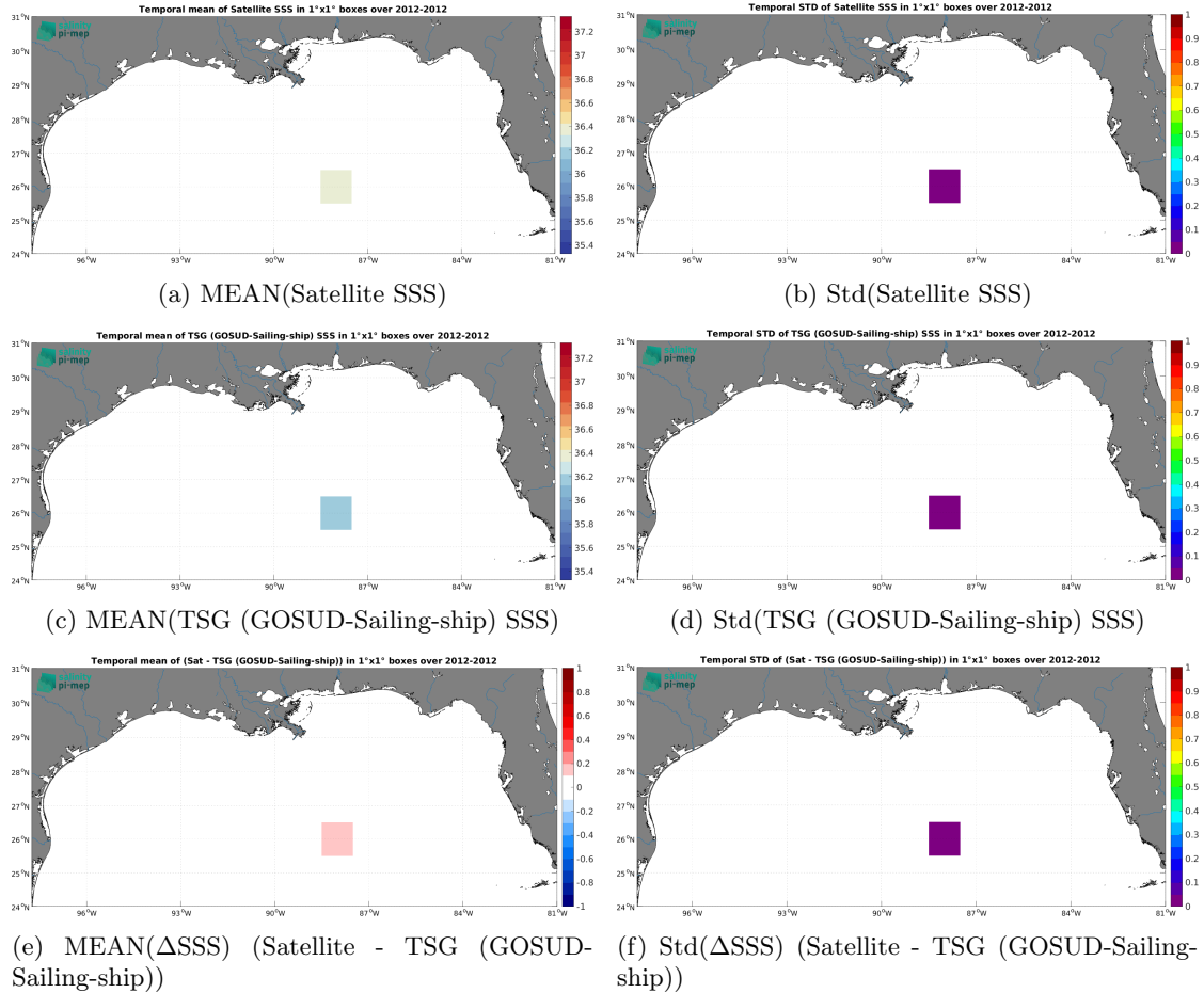
Figure 7: Temporal mean (left) and Std (right) of SSS from Aquarius SSS L3 OR v5 - 7-Day running (NASA-GSFC) (top), TSG (GOSUD-Sailing-ship) (middle), and of \Delta\text{SSS} (Satellite - TSG (GOSUD-Sailing-ship)). Only match-up pairs are used to generate these maps.
