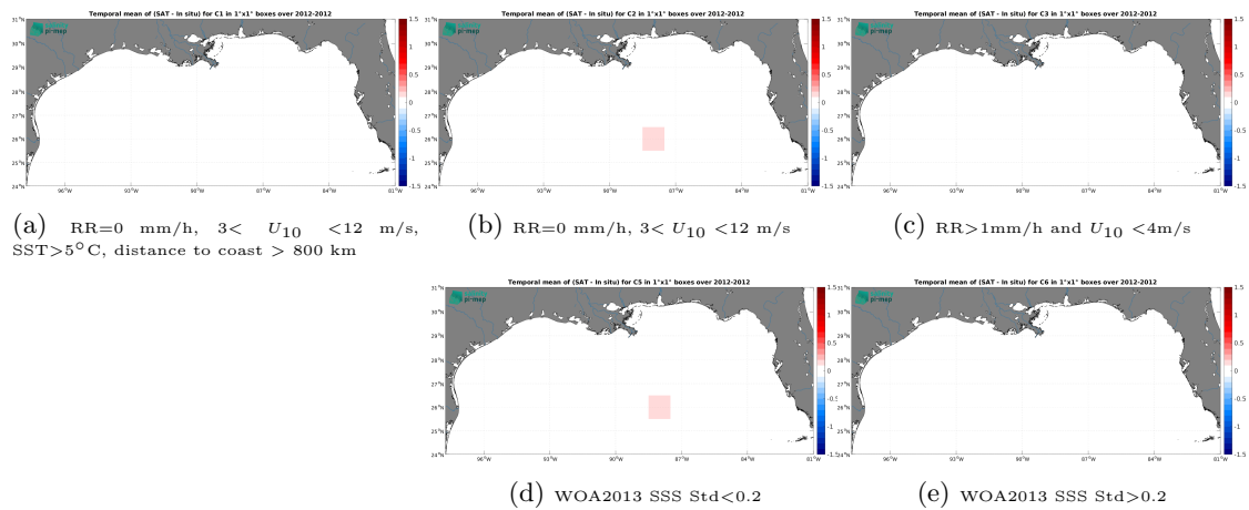
Figure 14: Temporal mean gridded over spatial boxes of size 1^\circ \times 1^\circ of \Delta SSS (Aquarius SSS L3 OR v5 - 7-Day running (NASA-GSFC) - TSG (GOSUD-Sailing-ship)) for 5 different subdatasets corresponding to:RR=0 mm/h, 3 < U_{10} < 12 m/s, SST >5^\circ\text{C} , distance to coast > 800 km (a), RR=0 mm/h, 3 < U_{10} < 12 m/s (b), RR >1 mm/h and U_{10} < 4 m/s (c), WOA2013 SSS Std <0.2 (d), WOA2013 SSS Std >0.2 (e).
