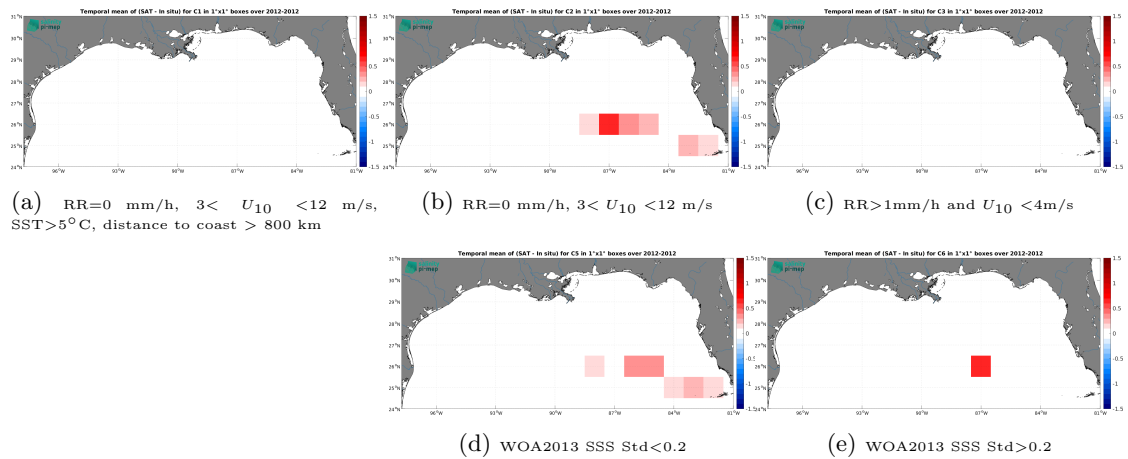
Figure 12: Temporal mean gridded over spatial boxes of size 1^{\circ}\times 1^{\circ} of \Delta SSS (Aquarius SSS L3 OR v5 - 7-Day running (NASA-GSFC) - TSG (GOSUD-Sailing-ship)) for 5 different subdatasets corresponding to:RR=0 mm/h, 3 < U_{10} < 12 m/s, SST >5^{\circ}\text{C} , distance to coast > 800 km (a), RR=0 mm/h, 3 < U_{10} < 12 m/s (b), RR >1 mm/h and U_{10} < 4 m/s (c), WOA2013 SSS Std <0.2 (d), WOA2013 SSS Std >0.2 (e).
