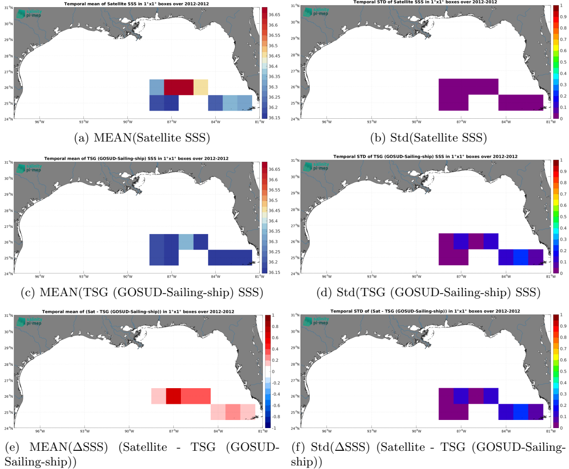
Figure 6: Temporal mean (left) and Std (right) of SSS from Aquarius SSS L3 OR v5 - 7-Day running (NASA-GSFC) (top), TSG (GOSUD-Sailing-ship) (middle), and of \Delta\text{SSS} (Satellite - TSG (GOSUD-Sailing-ship)). Only match-up pairs are used to generate these maps.
