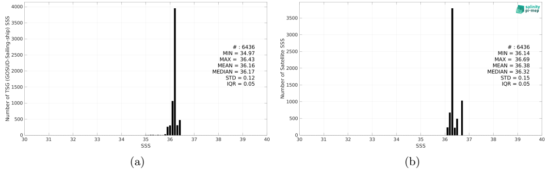
Figure 2: Histograms of SSS from TSG (GOSUD-Sailing-ship) (a) and Aquarius SSS L3 OR v5 - 7-Day running (NASA-GSFC) (b) considering all match-up pairs per bins of 0.1 over the Mississippi river plume Pi-MEP region and for the full satellite product period.
