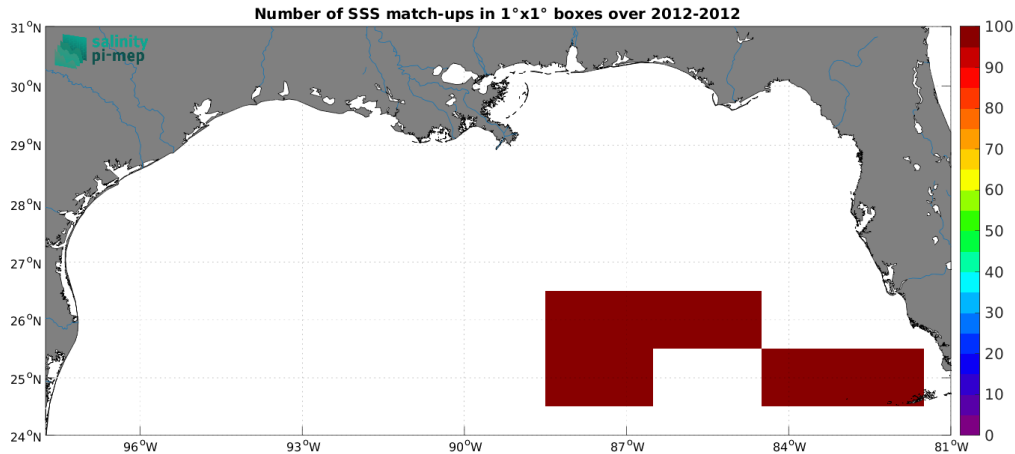
Figure 4: Number of SSS match-ups between TSG (GOSUD-Sailing-ship) SSS and the Aquarius SSS L3 OR v5 - 7-Day running (NASA-GSFC) SSS product for the Mississippi river plume Pi-MEP region over 1^\circ \times 1^\circ boxes and for the full satellite product period.
