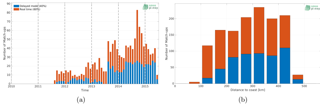
Figure 1: Number of match-ups between Argo and Aquarius SSS L3 OR v5 - 7-Day running (NASA-GSFC) SSS as a function of time (a) and as function of the distance to coast (b) over the Mississippi river plume Pi-MEP region and for the full satellite product period.
