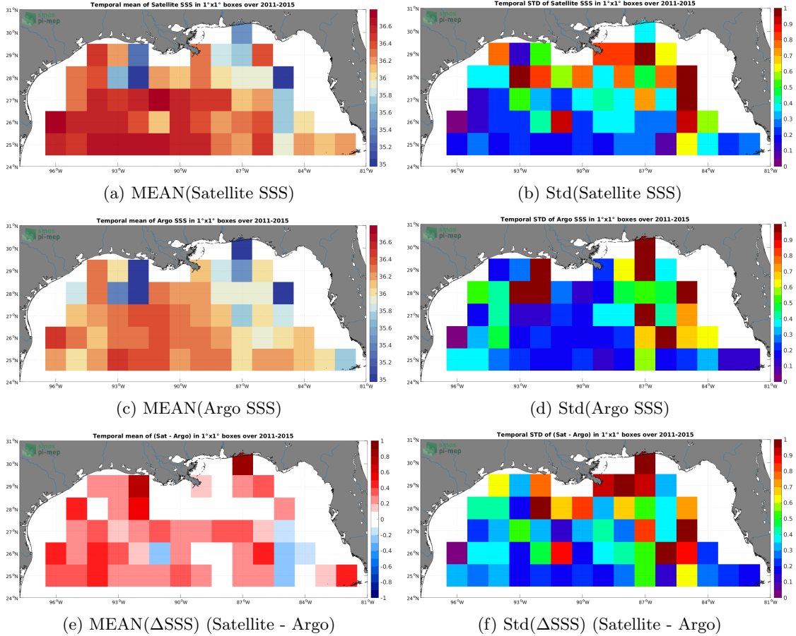
Figure 6: Temporal mean (left) and Std (right) of SSS from Aquarius SSS L3 OR v5 - 7-Day running (NASA-GSFC) (top), Argo (middle), and of \Delta\text{SSS} (Satellite - Argo). Only match-up pairs are used to generate these maps.
