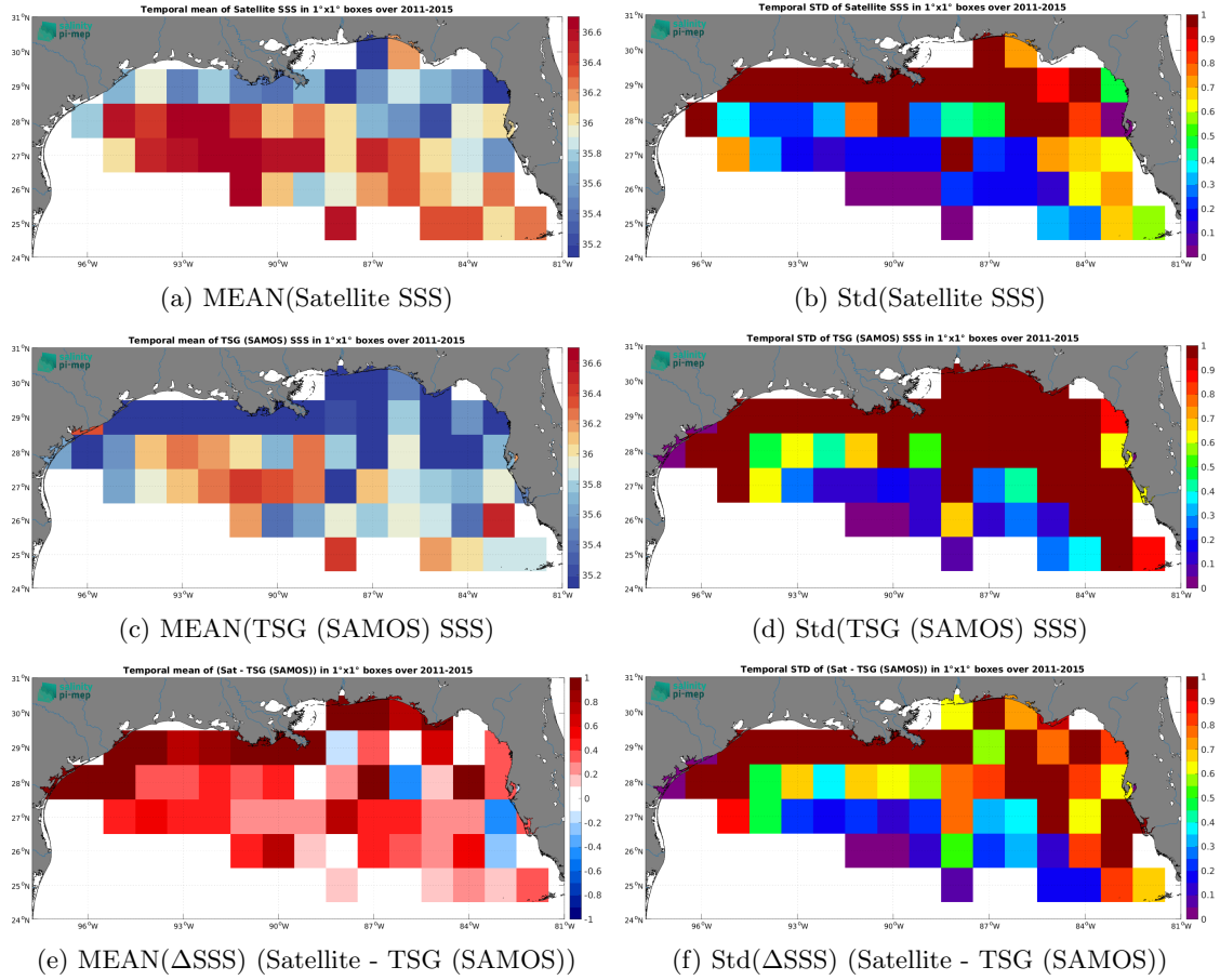
Figure 7: Temporal mean (left) and Std (right) of SSS from Aquarius SSS L3 OR v5 - 7-Day running - Rain mask (NASA-GSFC) (top), TSG (SAMOS) (middle), and of \Delta\text{SSS} (Satellite - TSG (SAMOS)). Only match-up pairs are used to generate these maps.
