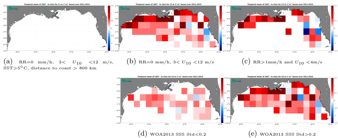
Figure 14: Temporal mean gridded over spatial boxes of size 1^\circ \times 1^\circ of \Delta SSS (Aquarius SSS L3 OR v5 - 7-Day running - Rain mask (NASA-GSFC) - TSG (SAMOS)) for 5 different subdatasets corresponding to: RR=0 mm/h, 3 < U_{10} < 12 m/s, SST > 5^\circ\text{C} , distance to coast > 800 km (a), RR=0 mm/h, 3 < U_{10} < 12 m/s (b), RR > 1 mm/h and U_{10} < 4 m/s (c), WOA2013 SSS Std < 0.2 (d), WOA2013 SSS Std > 0.2 (e).
