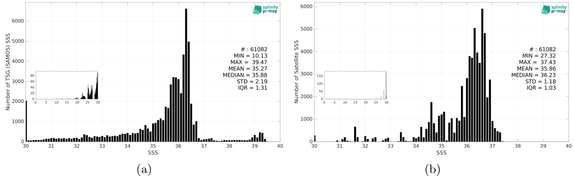
Figure 3: Histograms of SSS from TSG (SAMOS) (a) and Aquarius SSS L3 OR v5 - 7-Day running - Rain mask (NASA-GSFC) (b) considering all match-up pairs per bins of 0.1 over the Mississippi river plume Pi-MEP region and for the full satellite product period.
