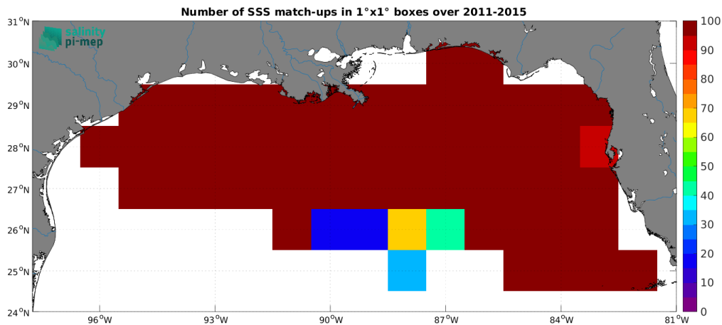
Figure 5: Number of SSS match-ups between TSG (SAMOS) SSS and the Aquarius SSS L3 OR v5 - 7-Day running - Rain mask (NASA-GSFC) SSS product for the Mississippi river plume Pi-MEP region over 1^\circ \times 1^\circ boxes and for the full satellite product period.
