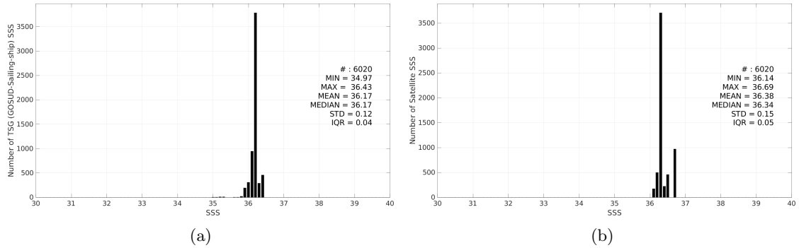
Figure 3: Histograms of SSS from TSG (GOSUD-Sailing-ship) (a) and Aquarius SSS L3 OR v5 - 7-Day running - Rain mask (NASA-GSFC) (b) considering all match-up pairs per bins of 0.1 over the Mississippi river plume Pi-MEP region and for the full satellite product period.
