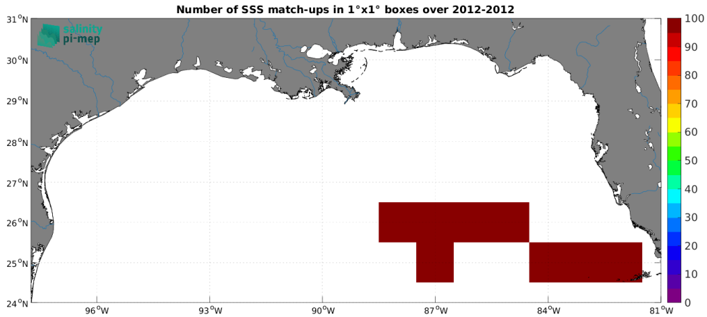
Figure 5: Number of SSS match-ups between TSG (GOSUD-Sailing-ship) SSS and the Aquarius SSS L3 OR v5 - 7-Day running - Rain mask (NASA-GSFC) SSS product for the Mississippi river plume Pi-MEP region over 1^\circ \times 1^\circ boxes and for the full satellite product period.
