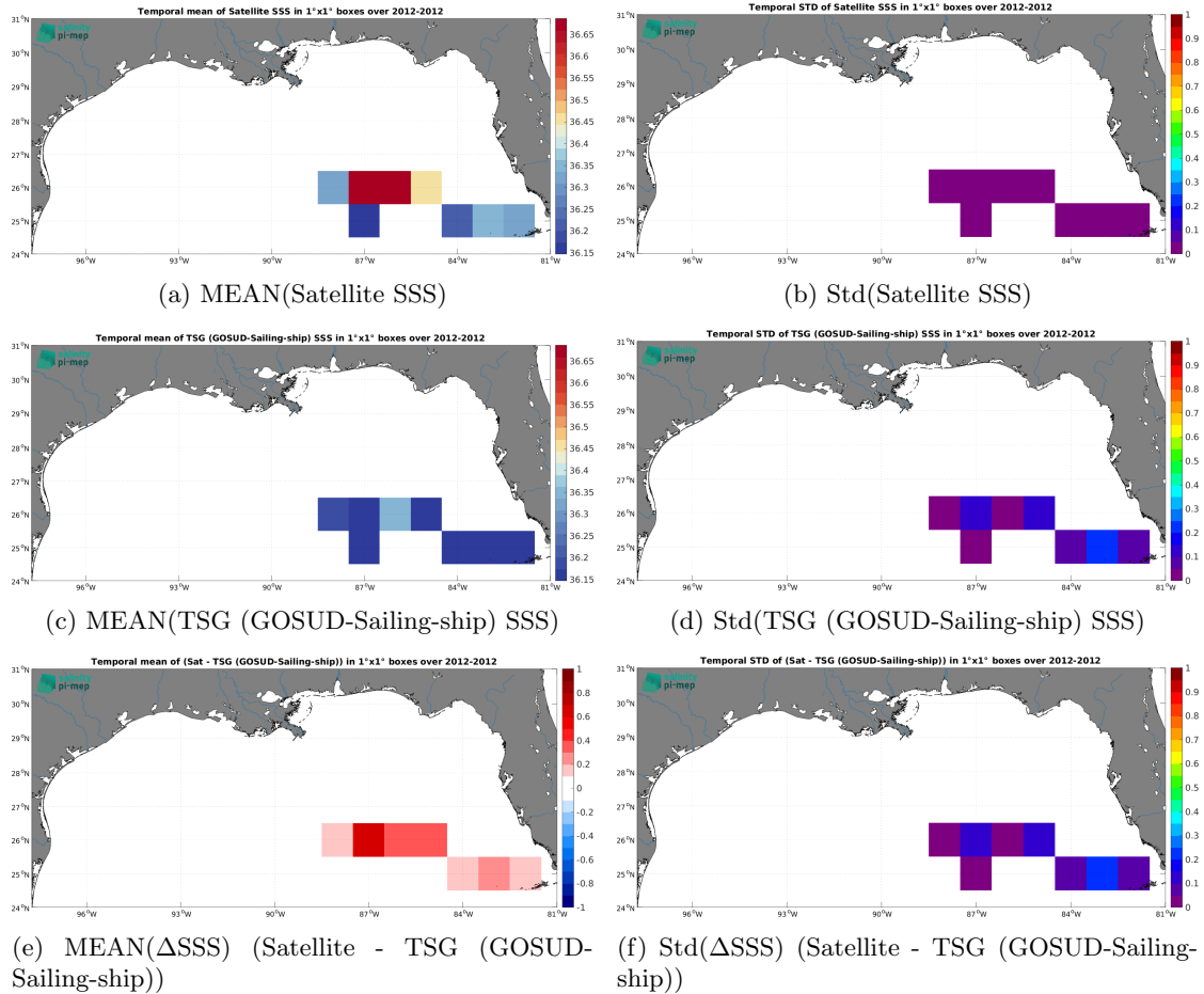
Figure 7: Temporal mean (left) and Std (right) of SSS from Aquarius SSS L3 OR v5 - 7-Day running - Rain mask (NASA-GSFC) (top), TSG (GOSUD-Sailing-ship) (middle), and of \Delta\text{SSS} (Satellite - TSG (GOSUD-Sailing-ship)). Only match-up pairs are used to generate these maps.
