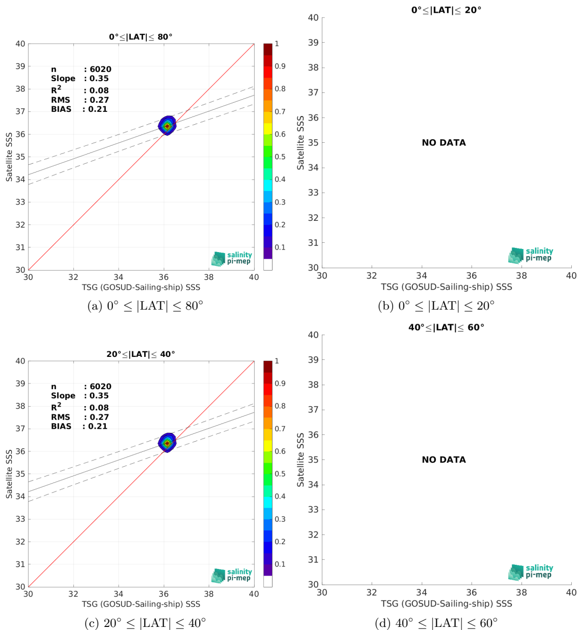
Figure 10: Contour maps of the concentration of Aquarius SSS L3 OR v5 - 7-Day running - Rain mask (NASA-GSFC) SSS (y-axis) versus TSG (GOSUD-Sailing-ship) SSS (x-axis) at match-up pairs for different latitude bands. For each plot, the red line shows x=y . The black thin and dashed lines indicate a linear fit through the data cloud and the \pm 95\% confidence levels, respectively. The number match-up pairs n , the slope and R^2 coefficient of the linear fit, the root mean square (RMS) and the mean bias between satellite and in situ data are indicated for each latitude band in each plots.
