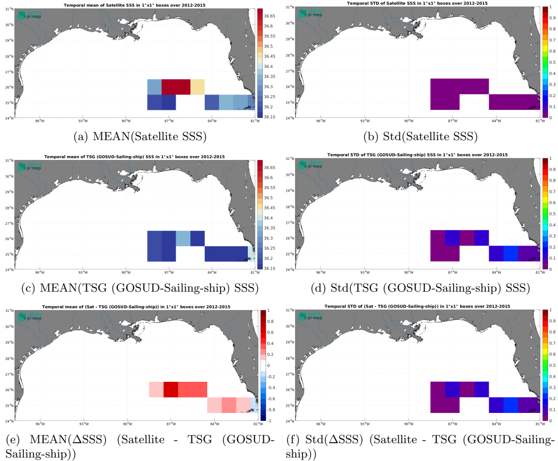
Figure 6: Temporal mean (left) and Std (right) of SSS from Aquarius SSS L3 OR v5 - 7-Day running - Rain mask (NASA-GSFC) (top), TSG (GOSUD-Sailing-ship) (middle), and of \Delta\text{SSS} (Satellite - TSG (GOSUD-Sailing-ship)). Only match-up pairs are used to generate these maps.
