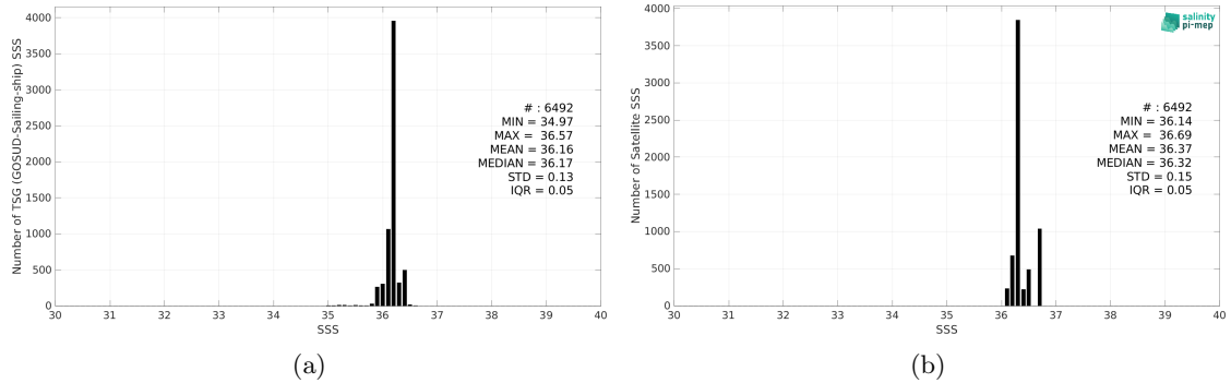
Figure 2: Histograms of SSS from TSG (GOSUD-Sailing-ship) (a) and Aquarius SSS L3 OR v5 - 7-Day running - Rain mask (NASA-GSFC) (b) considering all match-up pairs per bins of 0.1 over the Mississippi river plume Pi-MEP region and for the full satellite product period.
