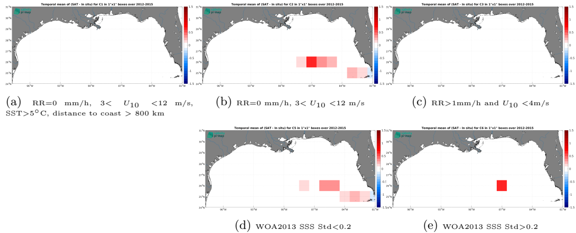
Figure 12: Temporal mean gridded over spatial boxes of size 1^{\circ}\times 1^{\circ} of \Delta SSS (Aquarius SSS L3 OR v5 - 7-Day running - Rain mask (NASA-GSFC) - TSG (GOSUD-Sailing-ship)) for 5 different subdatasets corresponding to:RR=0 mm/h, 3 < U_{10} < 12 m/s, SST >5^{\circ}\text{C} , distance to coast > 800 km (a), RR=0 mm/h, 3 < U_{10} < 12 m/s (b), RR >1 mm/h and U_{10} < 4 m/s (c), WOA2013 SSS Std <0.2 (d), WOA2013 SSS Std >0.2 (e).
