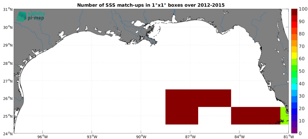
Figure 4: Number of SSS match-ups between TSG (GOSUD-Sailing-ship) SSS and the Aquarius SSS L3 OR v5 - 7-Day running - Rain mask (NASA-GSFC) SSS product for the Mississippi river plume Pi-MEP region over 1^\circ \times 1^\circ boxes and for the full satellite product period.
