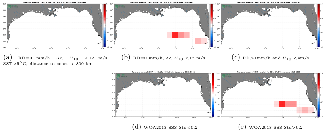
Figure 12: Temporal mean gridded over spatial boxes of size 1^\circ \times 1^\circ of \Delta SSS (Aquarius SSS L3 OR v5 - 7-Day running - Rain mask (NASA-GSFC) - TSG (GOSUD-Sailing-ship)) for 5 different subdatasets corresponding to:RR=0 mm/h, 3 < U_{10} < 12 m/s, SST >5^\circ\text{C} , distance to coast > 800 km (a), RR=0 mm/h, 3 < U_{10} < 12 m/s (b), RR >1 mm/h and U_{10} < 4 m/s (c), WOA2013 SSS Std <0.2 (d), WOA2013 SSS Std >0.2 (e).
