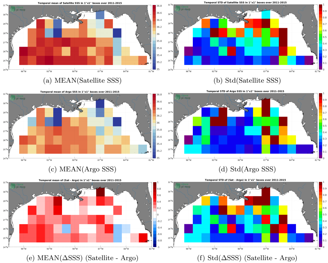
Figure 6: Temporal mean (left) and Std (right) of SSS from Aquarius SSS L3 OR v5 - 7-Day running - Rain mask (NASA-GSFC) (top), Argo (middle), and of \Delta SSS (Satellite - Argo). Only match-up pairs are used to generate these maps.
