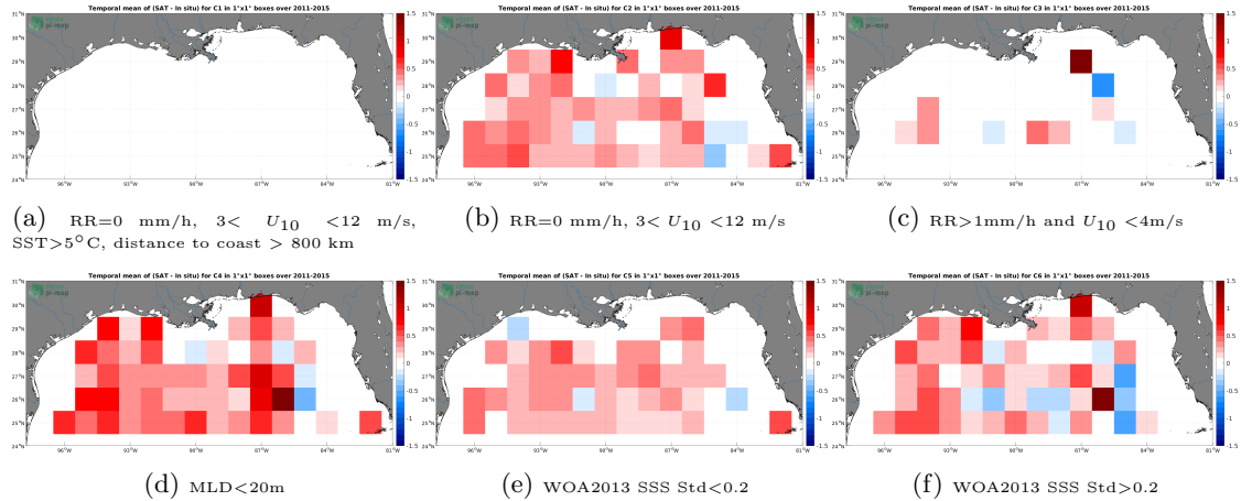
Figure 12: Temporal mean gridded over spatial boxes of size 1^{\circ}\times 1^{\circ} of \Delta\text{SSS} (Aquarius SSS L3 OR v5 - 7-Day running - Rain mask (NASA-GSFC) - Argo) for 6 different subdatasets corresponding to: RR=0 mm/h, 3 < U_{10} < 12 m/s, SST > 5^{\circ}\text{C} , distance to coast > 800 km (a), RR=0 mm/h, 3 < U_{10} < 12 m/s (b), RR > 1\text{mm/h} and U_{10} < 4\text{m/s} (c), MLD < 20\text{m} (d), WOA2013 SSS Std < 0.2 (e), WOA2013 SSS Std > 0.2 (f).
