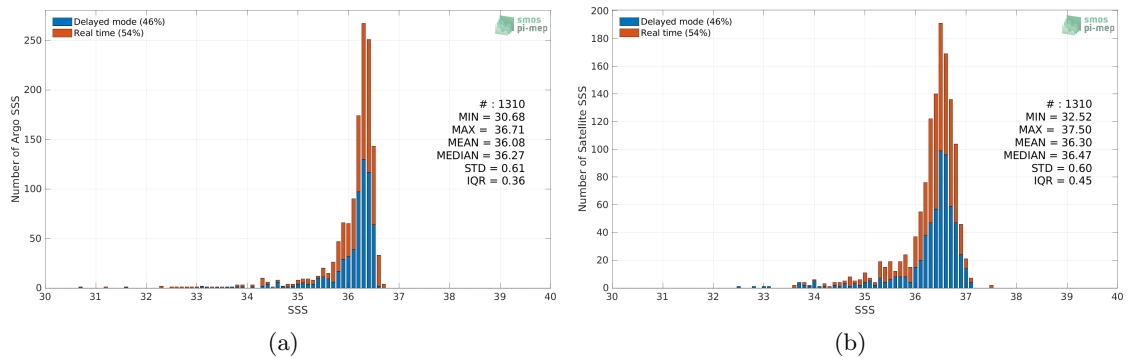
Figure 2: Histograms of SSS from Argo (a) and Aquarius SSS L3 OR v5 - 7-Day running - Rain mask (NASA-GSFC) (b) considering all match-up pairs per bins of 0.1 over the Mississippi river plume Pi-MEP region and for the full satellite product period.
