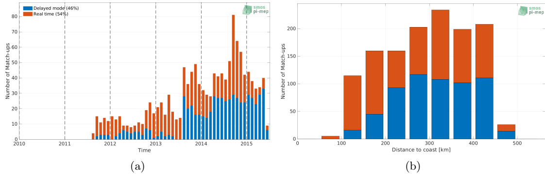
Figure 1: Number of match-ups between Argo and Aquarius SSS L3 OR v5 - 7-Day running - Rain mask (NASA-GSFC) SSS as a function of time (a) and as function of the distance to coast (b) over the Mississippi river plume Pi-MEP region and for the full satellite product period.
