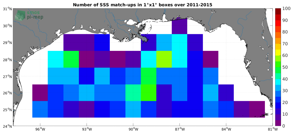
Figure 4: Number of SSS match-ups between Argo SSS and the Aquarius SSS L3 OR v5 - 7-Day running - Rain mask (NASA-GSFC) SSS product for the Mississippi river plume Pi-MEP region over 1^\circ \times 1^\circ boxes and for the full satellite product period.
