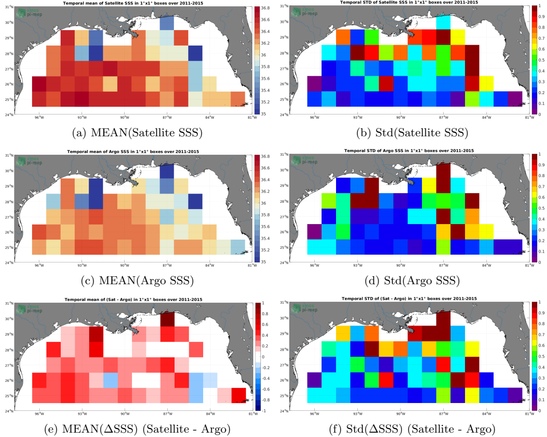
Figure 6: Temporal mean (left) and Std (right) of SSS from Aquarius SSS L3 OR v5 - 7-Day running - Rain mask (NASA-GSFC) (top), Argo (middle), and of \Delta\text{SSS} (Satellite - Argo). Only match-up pairs are used to generate these maps.
