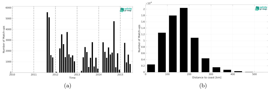
Figure 2: Number of match-ups between TSG (SAMOS) and Aquarius SSS L3 OR v5 - Monthly (NASA-GSFC) SSS as a function of time (a) and as function of the distance to coast (b) over the Mississippi river plume Pi-MEP region and for the full satellite product period.
