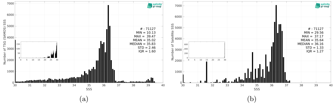
Figure 3: Histograms of SSS from TSG (SAMOS) (a) and Aquarius SSS L3 OR v5 - Monthly (NASA-GSFC) (b) considering all match-up pairs per bins of 0.1 over the Mississippi river plume Pi-MEP region and for the full satellite product period.
