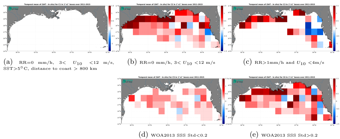
Figure 14: Temporal mean gridded over spatial boxes of size 1^\circ \times 1^\circ of \Delta SSS (Aquarius SSS L3 OR v5 - Monthly (NASA-GSFC) - TSG (SAMOS)) for 5 different subdatasets corresponding to: RR=0 mm/h, 3 < U_{10} < 12 m/s, SST > 5°C, distance to coast > 800 km (a), RR=0 mm/h, 3 < U_{10} < 12 m/s (b), RR > 1mm/h and U_{10} < 4 m/s (c), WOA2013 SSS Std < 0.2 (d), WOA2013 SSS Std > 0.2 (e).
