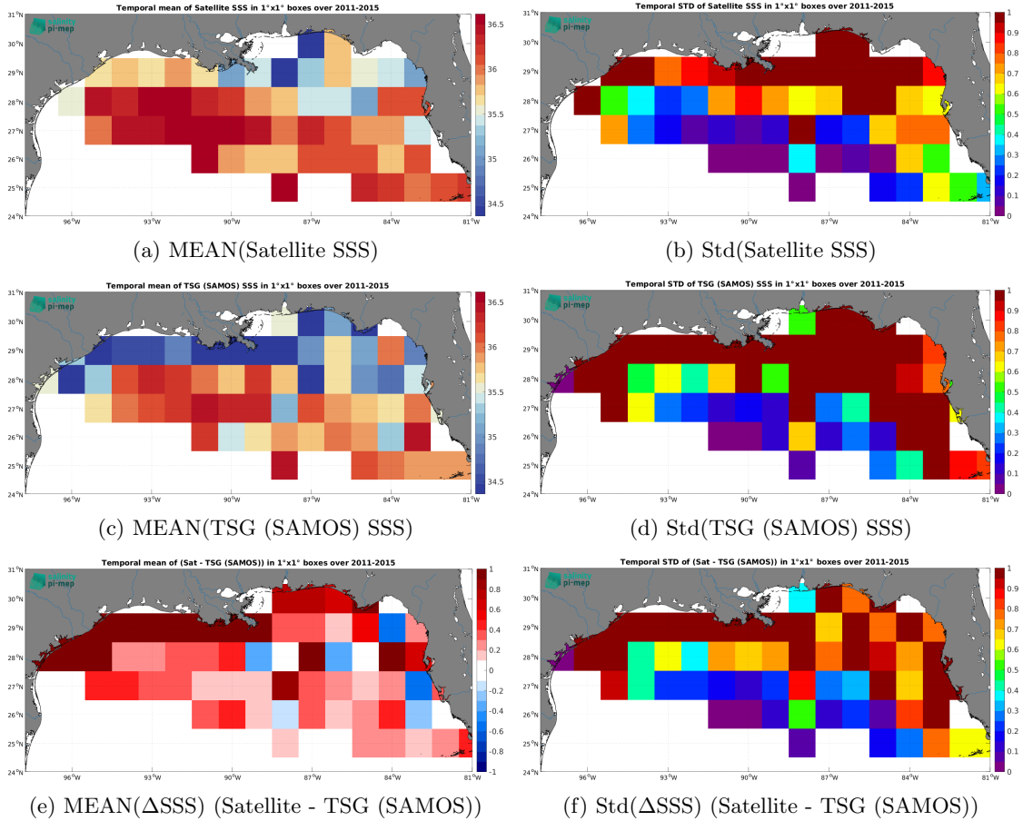
Figure 7: Temporal mean (left) and Std (right) of SSS from Aquarius SSS L3 OR v5 - Monthly (NASA-GSFC) (top), TSG (SAMOS) (middle), and of \Delta\text{SSS} (Satellite - TSG (SAMOS)). Only match-up pairs are used to generate these maps.
