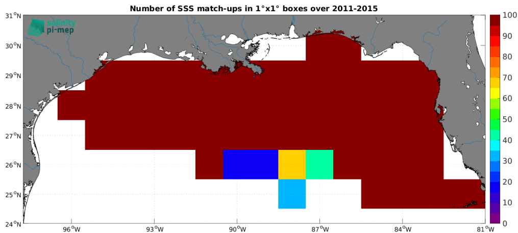
Figure 5: Number of SSS match-ups between TSG (SAMOS) SSS and the Aquarius SSS L3 OR v5 - Monthly (NASA-GSFC) SSS product for the Mississippi river plume Pi-MEP region over 1^\circ \times 1^\circ boxes and for the full satellite product period.
