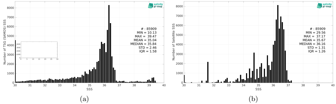
Figure 2: Histograms of SSS from TSG (SAMOS) (a) and Aquarius SSS L3 OR v5 - Monthly (NASA-GSFC) (b) considering all match-up pairs per bins of 0.1 over the Mississippi river plume Pi-MEP region and for the full satellite product period.
