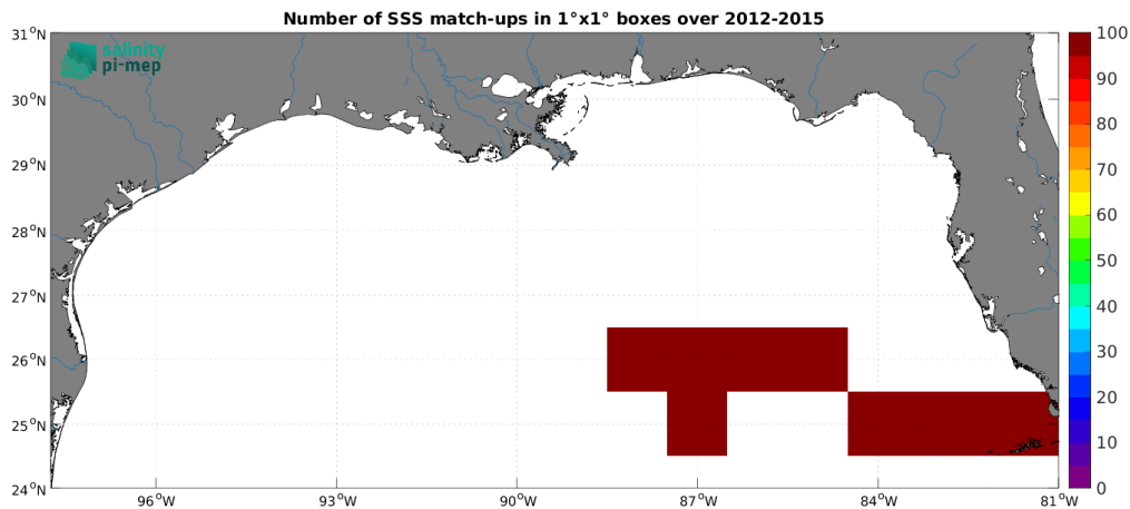
Figure 5: Number of SSS match-ups between TSG (GOSUD-Sailing-ship) SSS and the Aquarius SSS L3 OR v5 - Monthly (NASA-GSFC) SSS product for the Mississippi river plume Pi-MEP region over 1^\circ \times 1^\circ boxes and for the full satellite product period.
