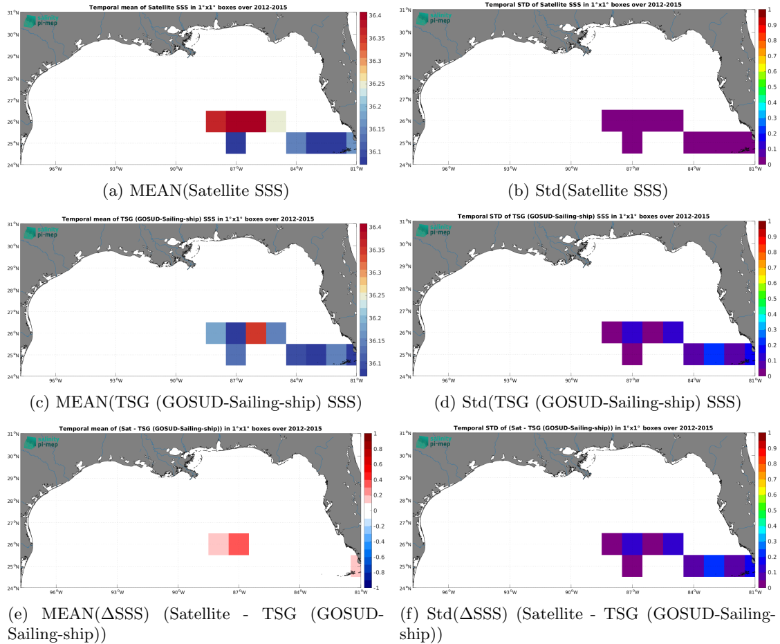
Figure 7: Temporal mean (left) and Std (right) of SSS from Aquarius SSS L3 OR v5 - Monthly (NASA-GSFC) (top), TSG (GOSUD-Sailing-ship) (middle), and of \Delta\text{SSS} (Satellite - TSG (GOSUD-Sailing-ship)). Only match-up pairs are used to generate these maps.
