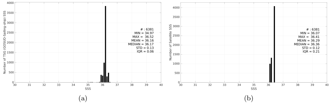
Figure 3: Histograms of SSS from TSG (GOSUD-Sailing-ship) (a) and Aquarius SSS L3 OR v5 - Monthly (NASA-GSFC) (b) considering all match-up pairs per bins of 0.1 over the Mississippi river plume Pi-MEP region and for the full satellite product period.
