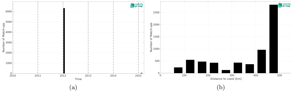
Figure 2: Number of match-ups between TSG (GOSUD-Sailing-ship) and Aquarius SSS L3 OR v5 - Monthly (NASA-GSFC) SSS as a function of time (a) and as function of the distance to coast (b) over the Mississippi river plume Pi-MEP region and for the full satellite product period.
