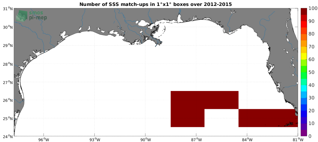
Figure 4: Number of SSS match-ups between TSG (GOSUD-Sailing-ship) SSS and the Aquarius SSS L3 OR v5 - Monthly (NASA-GSFC) SSS product for the Mississippi river plume Pi-MEP region over 1^\circ \times 1^\circ boxes and for the full satellite product period.
