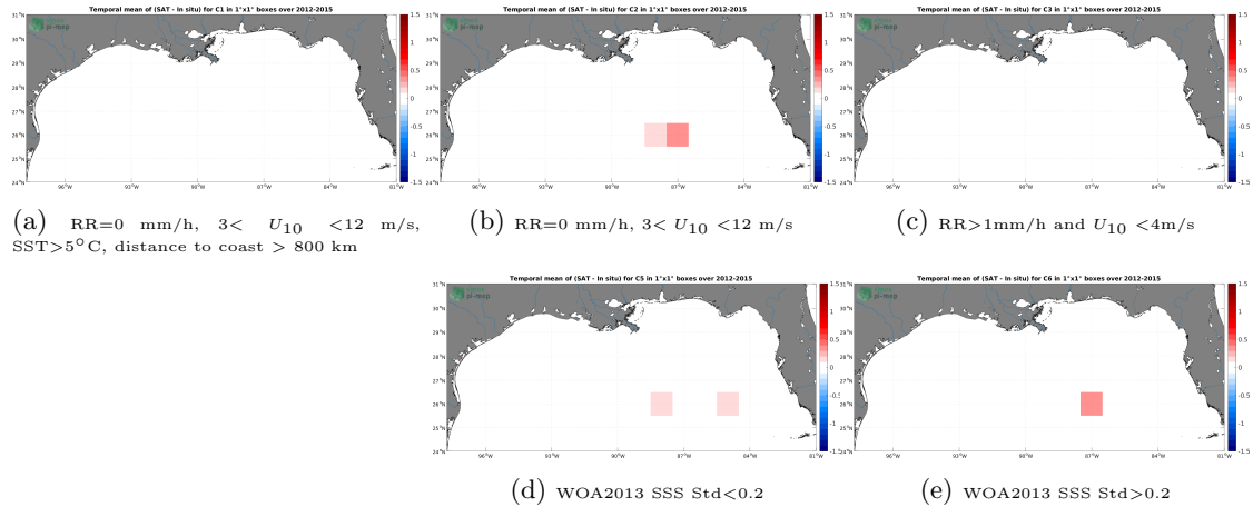
Figure 12: Temporal mean gridded over spatial boxes of size 1^{\circ}\times 1^{\circ} of \Delta SSS (Aquarius SSS L3 OR v5 - Monthly (NASA-GSFC) - TSG (GOSUD-Sailing-ship)) for 5 different subdatasets corresponding to:RR=0 mm/h, 3 < U_{10} < 12 m/s, SST >5^{\circ}\text{C} , distance to coast > 800 km (a), RR=0 mm/h, 3 < U_{10} < 12 m/s (b), RR >1 mm/h and U_{10} < 4 m/s (c), WOA2013 SSS Std <0.2 (d), WOA2013 SSS Std >0.2 (e).
