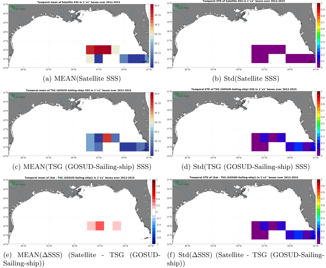
Figure 6: Temporal mean (left) and Std (right) of SSS from Aquarius SSS L3 OR v5 - Monthly (NASA-GSFC) (top), TSG (GOSUD-Sailing-ship) (middle), and of \Delta\text{SSS} (Satellite - TSG (GOSUD-Sailing-ship)). Only match-up pairs are used to generate these maps.
