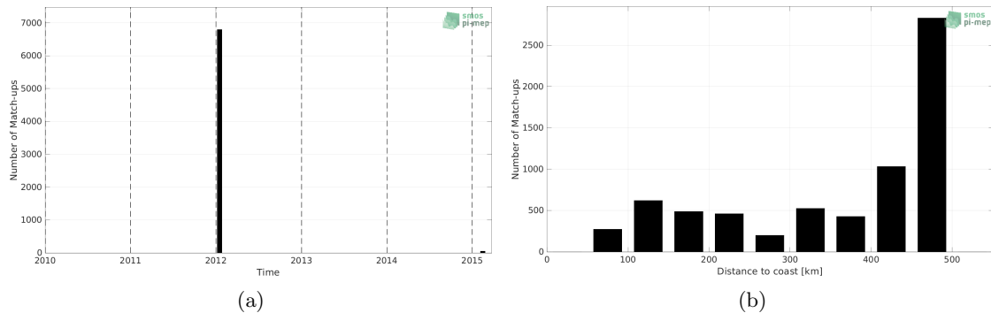
Figure 1: Number of match-ups between TSG (GOSUD-Sailing-ship) and Aquarius SSS L3 OR v5 - Monthly (NASA-GSFC) SSS as a function of time (a) and as function of the distance to coast (b) over the Mississippi river plume Pi-MEP region and for the full satellite product period.
