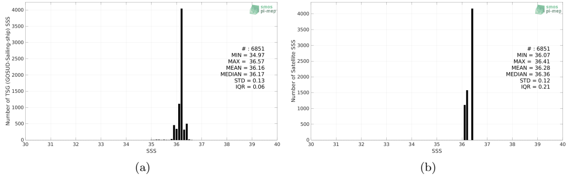
Figure 2: Histograms of SSS from TSG (GOSUD-Sailing-ship) (a) and Aquarius SSS L3 OR v5 - Monthly (NASA-GSFC) (b) considering all match-up pairs per bins of 0.1 over the Mississippi river plume Pi-MEP region and for the full satellite product period.
