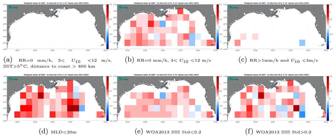
Figure 14: Temporal mean gridded over spatial boxes of size 1^\circ \times 1^\circ of \Delta SSS (Aquarius SSS L3 OR v5 - Monthly (NASA-GSFC) - Argo) for 6 different subdatasets corresponding to: RR=0 mm/h, 3 < U_{10} < 12 m/s, SST > 5^\circ\text{C} , distance to coast > 800 km (a), RR=0 mm/h, 3 < U_{10} < 12 m/s (b), RR > 1 mm/h and U_{10} < 4 m/s (c), MLD < 20 m (d), WOA2013 SSS Std < 0.2 (e), WOA2013 SSS Std > 0.2 (f).
