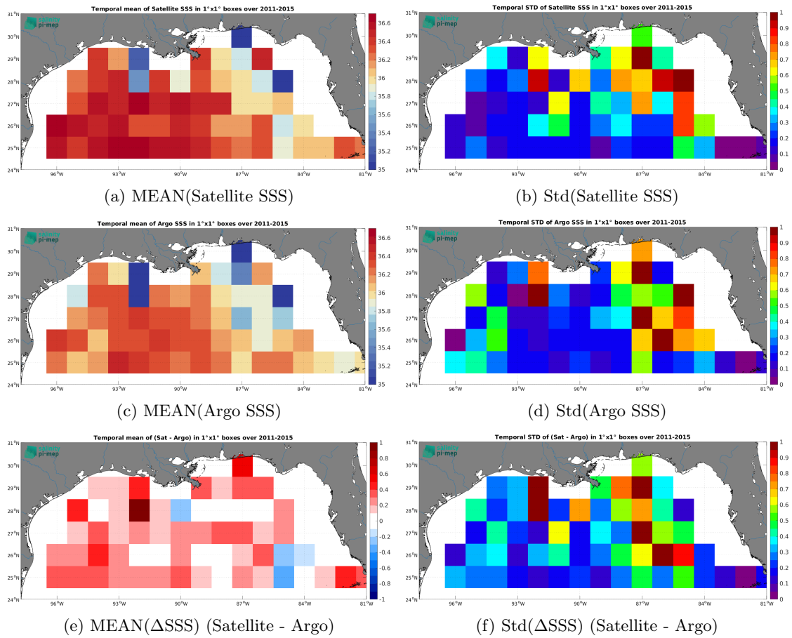
Figure 7: Temporal mean (left) and Std (right) of SSS from Aquarius SSS L3 OR v5 - Monthly (NASA-GSFC) (top), Argo (middle), and of \Delta SSS (Satellite - Argo). Only match-up pairs are used to generate these maps.
