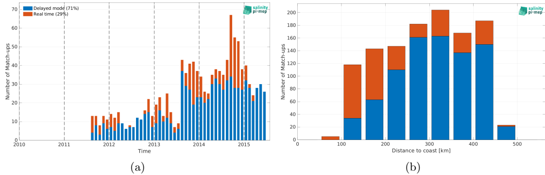
Figure 2: Number of match-ups between Argo and Aquarius SSS L3 OR v5 - Monthly (NASA-GSFC) SSS as a function of time (a) and as function of the distance to coast (b) over the Mississippi river plume Pi-MEP region and for the full satellite product period.
