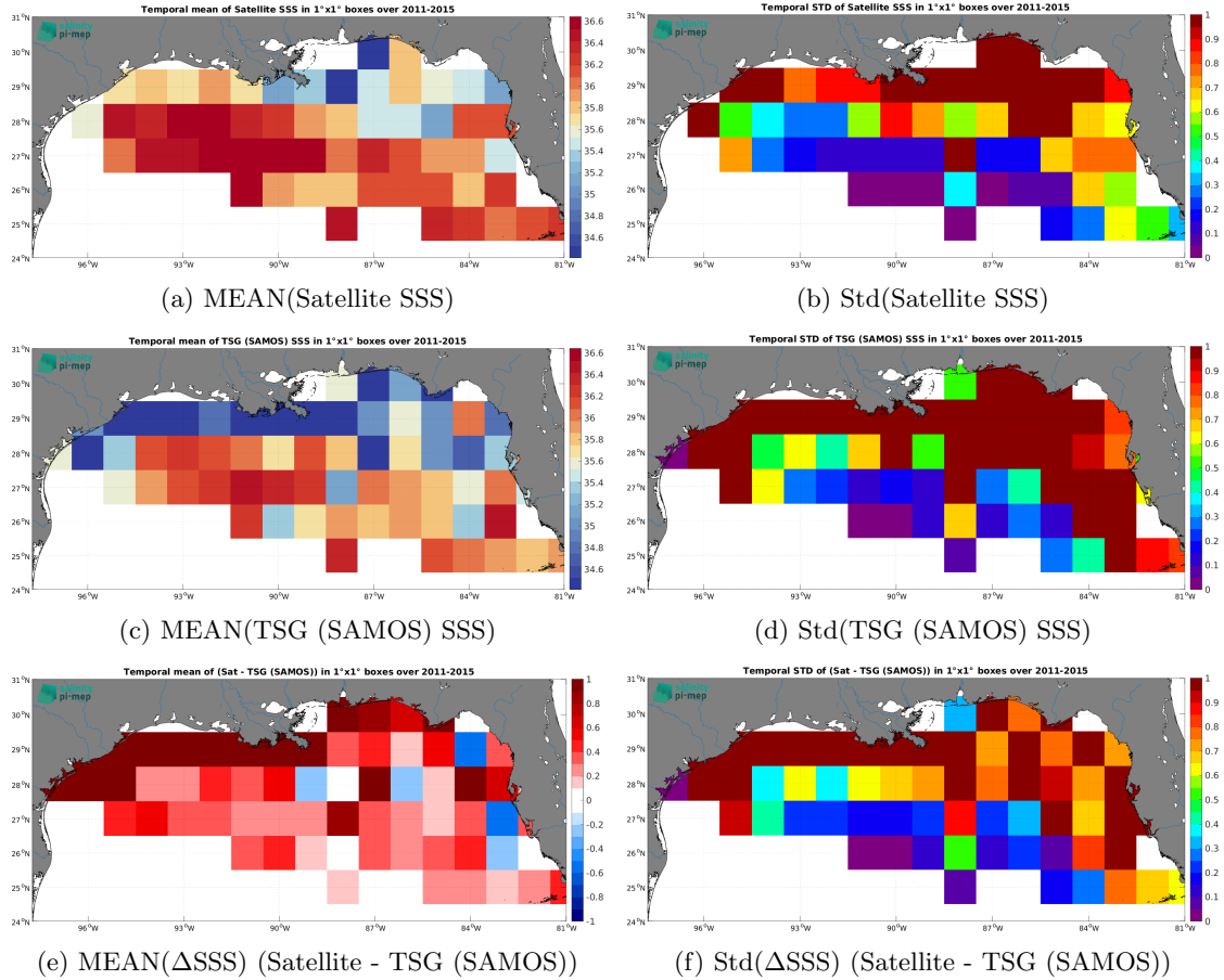
Figure 7: Temporal mean (left) and Std (right) of SSS from Aquarius SSS L3 OR v5 - Monthly - Rain mask (NASA-GSFC) (top), TSG (SAMOS) (middle), and of \Delta\text{SSS} (Satellite - TSG (SAMOS)). Only match-up pairs are used to generate these maps.
