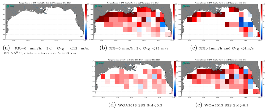
Figure 14: Temporal mean gridded over spatial boxes of size 1^\circ \times 1^\circ of \Delta SSS (Aquarius SSS L3 OR v5 - Monthly - Rain mask (NASA-GSFC) - TSG (SAMOS)) for 5 different subdatasets corresponding to:RR=0 mm/h, 3 < U_{10} < 12 m/s, SST>5°C, distance to coast > 800 km (a), RR=0 mm/h, 3 < U_{10} < 12 m/s (b), RR>1mm/h and U_{10} < 4 m/s (c), WOA2013 SSS Std<0.2 (d), WOA2013 SSS Std>0.2 (e).
