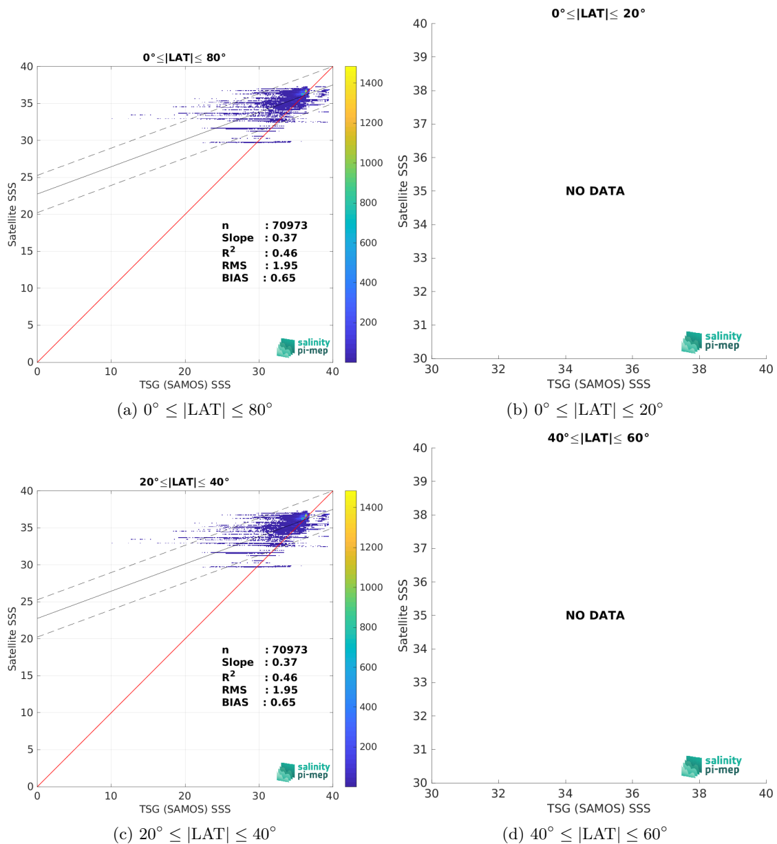
Figure 10: Contour maps of the concentration of Aquarius SSS L3 OR v5 - Monthly - Rain mask (NASA-GSFC) SSS (y-axis) versus TSG (SAMOS) SSS (x-axis) at match-up pairs for different latitude bands. For each plot, the red line shows x=y . The black thin and dashed lines indicate a linear fit through the data cloud and the \pm 95\% confidence levels, respectively. The number match-up pairs n , the slope and R^2 coefficient of the linear fit, the root mean square (RMS) and the mean bias between satellite and in situ data are indicated for each latitude band in each plots.
