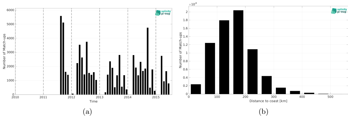
Figure 2: Number of match-ups between TSG (SAMOS) and Aquarius SSS L3 OR v5 - Monthly - Rain mask (NASA-GSFC) SSS as a function of time (a) and as function of the distance to coast (b) over the Mississippi river plume Pi-MEP region and for the full satellite product period.
