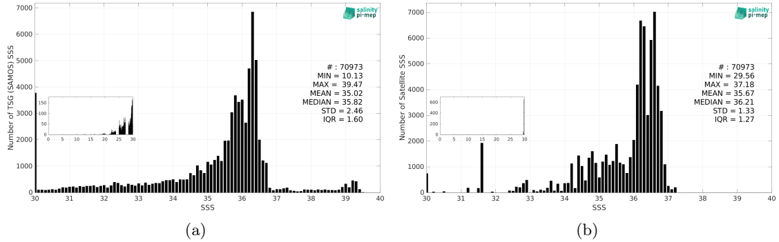
Figure 3: Histograms of SSS from TSG (SAMOS) (a) and Aquarius SSS L3 OR v5 - Monthly - Rain mask (NASA-GSFC) (b) considering all match-up pairs per bins of 0.1 over the Mississippi river plume Pi-MEP region and for the full satellite product period.
