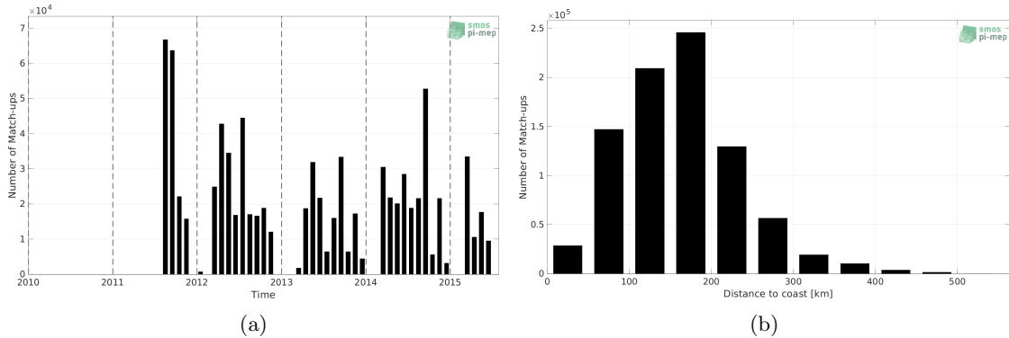
Figure 1: Number of match-ups between TSG (SAMOS) and Aquarius SSS L3 OR v5 - Monthly - Rain mask (NASA-GSFC) SSS as a function of time (a) and as function of the distance to coast (b) over the Mississippi river plume Pi-MEP region and for the full satellite product period.
