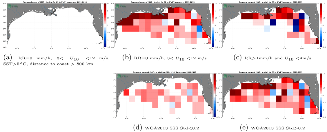
Figure 12: Temporal mean gridded over spatial boxes of size 1^{\circ}\times 1^{\circ} of \Delta\text{SSS} (Aquarius SSS L3 OR v5 - Monthly - Rain mask (NASA-GSFC) - TSG (SAMOS)) for 5 different subdatasets corresponding to:RR=0 mm/h, 3 < U_{10} < 12 m/s, SST >5^{\circ}\text{C} , distance to coast > 800 km (a), RR=0 mm/h, 3 < U_{10} < 12 m/s (b), RR >1 mm/h and U_{10} < 4 m/s (c), WOA2013 SSS Std <0.2 (d), WOA2013 SSS Std >0.2 (e).
