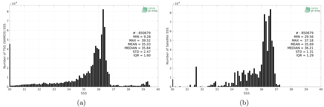
Figure 2: Histograms of SSS from TSG (SAMOS) (a) and Aquarius SSS L3 OR v5 - Monthly - Rain mask (NASA-GSFC) (b) considering all match-up pairs per bins of 0.1 over the Mississippi river plume Pi-MEP region and for the full satellite product period.
