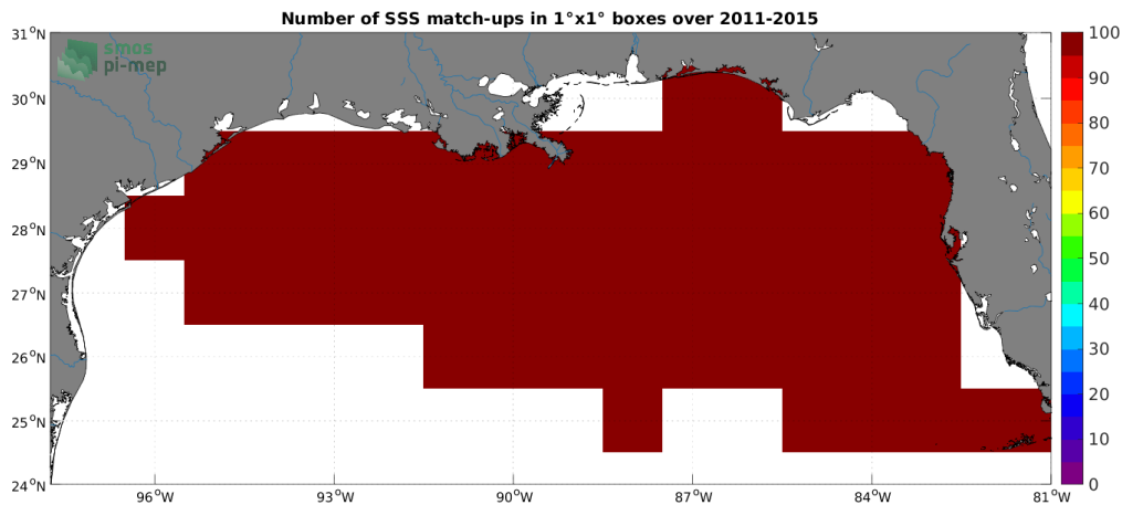
Figure 4: Number of SSS match-ups between TSG (SAMOS) SSS and the Aquarius SSS L3 OR v5 - Monthly - Rain mask (NASA-GSFC) SSS product for the Mississippi river plume Pi-MEP region over 1^\circ \times 1^\circ boxes and for the full satellite product period.
