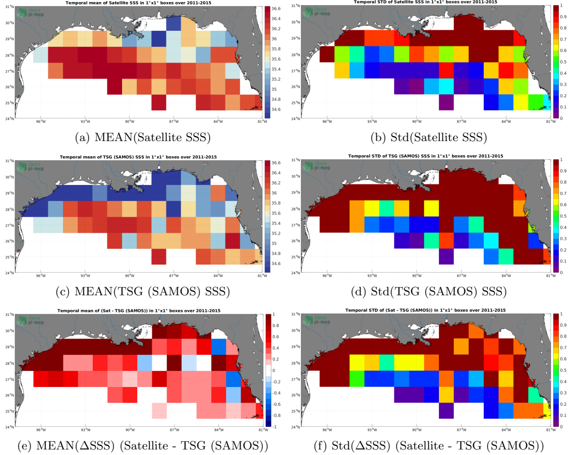
Figure 6: Temporal mean (left) and Std (right) of SSS from Aquarius SSS L3 OR v5 - Monthly - Rain mask (NASA-GSFC) (top), TSG (SAMOS) (middle), and of \Delta\text{SSS} (Satellite - TSG (SAMOS)). Only match-up pairs are used to generate these maps.
