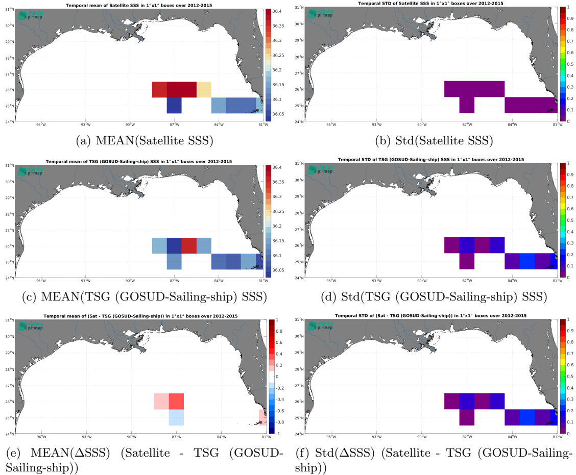
Figure 7: Temporal mean (left) and Std (right) of SSS from Aquarius SSS L3 OR v5 - Monthly - Rain mask (NASA-GSFC) (top), TSG (GOSUD-Sailing-ship) (middle), and of \Delta\text{SSS} (Satellite - TSG (GOSUD-Sailing-ship)). Only match-up pairs are used to generate these maps.
