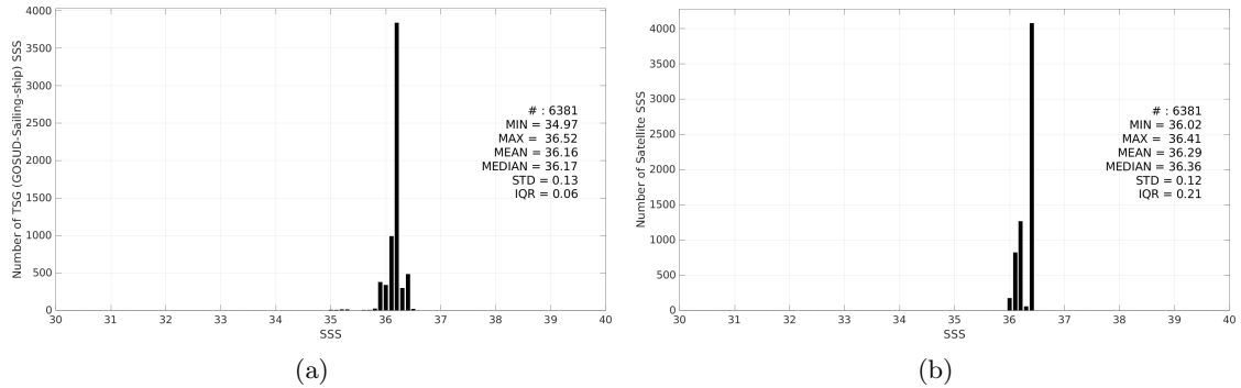
Figure 3: Histograms of SSS from TSG (GOSUD-Sailing-ship) (a) and Aquarius SSS L3 OR v5 - Monthly - Rain mask (NASA-GSFC) (b) considering all match-up pairs per bins of 0.1 over the Mississippi river plume Pi-MEP region and for the full satellite product period.
