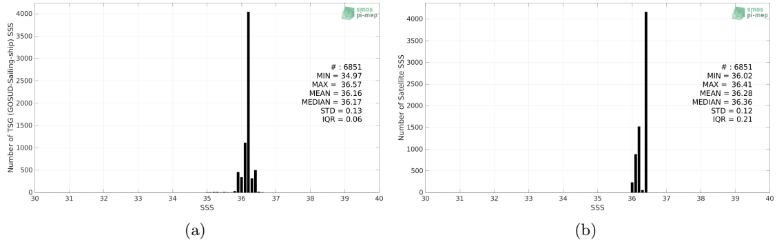
Figure 2: Histograms of SSS from TSG (GOSUD-Sailing-ship) (a) and Aquarius SSS L3 OR v5 - Monthly - Rain mask (NASA-GSFC) (b) considering all match-up pairs per bins of 0.1 over the Mississippi river plume Pi-MEP region and for the full satellite product period.
