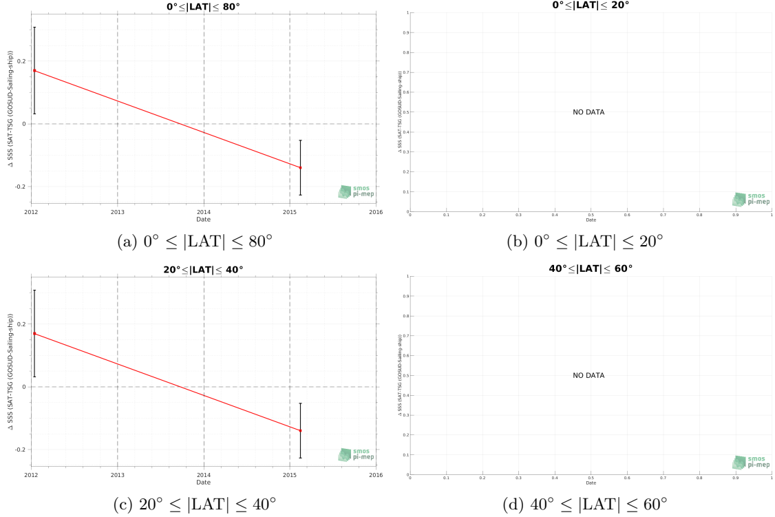
Figure 10: Monthly median (red curves) of \Delta SSS (Satellite - in situ ) between Aquarius SSS L3 OR v5 - Monthly - Rain mask (NASA-GSFC) and TSG (GOSUD-Sailing-ship) SSS as function of the geophysical conditions at match-up points. The median and std of \Delta SSS (Satellite - TSG (GOSUD-Sailing-ship)) is thus evaluated as function of the
