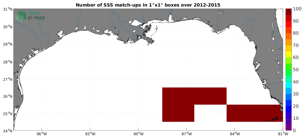
Figure 4: Number of SSS match-ups between TSG (GOSUD-Sailing-ship) SSS and the Aquarius SSS L3 OR v5 - Monthly - Rain mask (NASA-GSFC) SSS product for the Mississippi river plume Pi-MEP region over 1^\circ \times 1^\circ boxes and for the full satellite product period.
