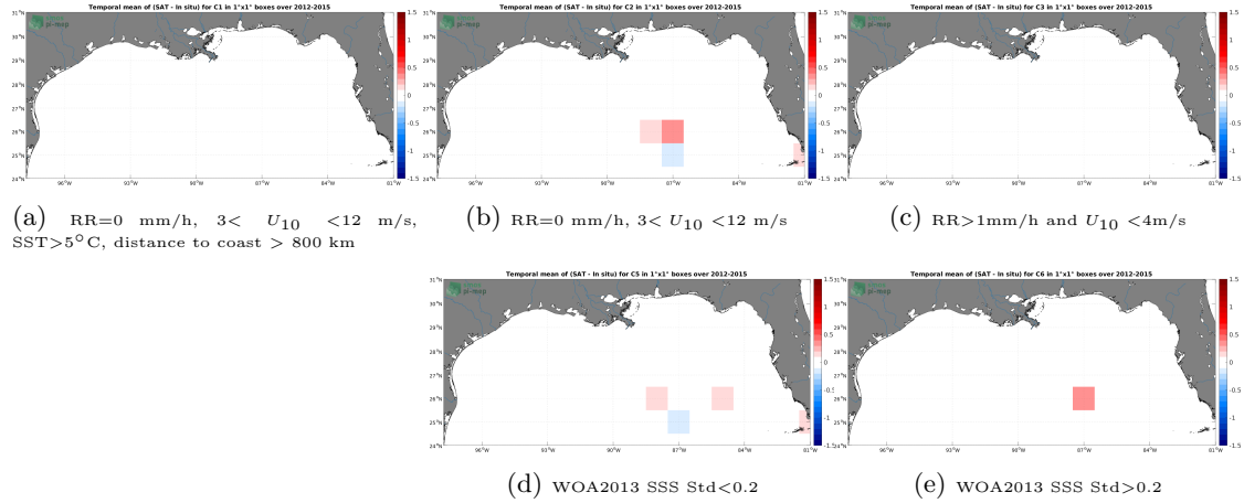
Figure 12: Temporal mean gridded over spatial boxes of size 1^{\circ}\times 1^{\circ} of \Delta SSS (Aquarius SSS L3 OR v5 - Monthly - Rain mask (NASA-GSFC) - TSG (GOSUD-Sailing-ship)) for 5 different subdatasets corresponding to:RR=0 mm/h, 3 < U_{10} < 12 m/s, SST >5^{\circ}\text{C} , distance to coast > 800 km (a), RR=0 mm/h, 3 < U_{10} < 12 m/s (b), RR >1 mm/h and U_{10} < 4 m/s (c), WOA2013 SSS Std <0.2 (d), WOA2013 SSS Std >0.2 (e).
