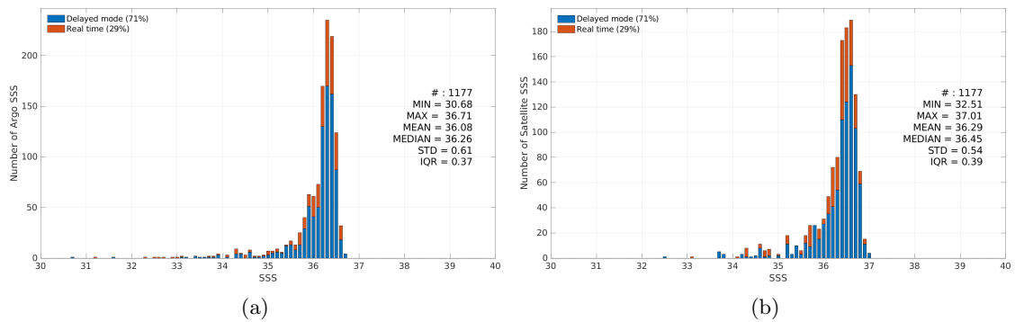
Figure 3: Histograms of SSS from Argo (a) and Aquarius SSS L3 OR v5 - Monthly - Rain mask (NASA-GSFC) (b) considering all match-up pairs per bins of 0.1 over the Mississippi river plume Pi-MEP region and for the full satellite product period.
