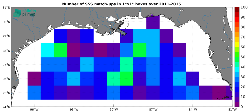
Figure 5: Number of SSS match-ups between Argo SSS and the Aquarius SSS L3 OR v5 - Monthly - Rain mask (NASA-GSFC) SSS product for the Mississippi river plume Pi-MEP region over 1^\circ \times 1^\circ boxes and for the full satellite product period.
