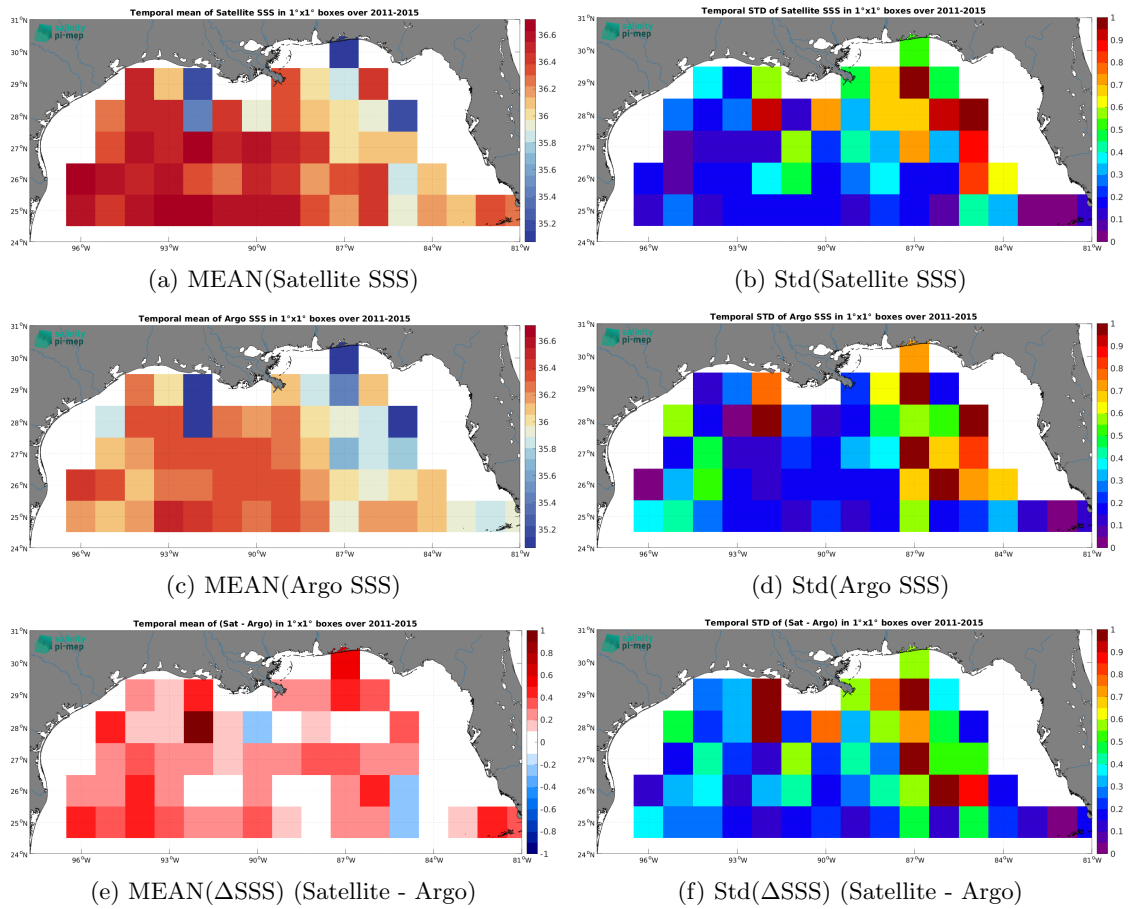
Figure 7: Temporal mean (left) and Std (right) of SSS from Aquarius SSS L3 OR v5 - Monthly - Rain mask (NASA-GSFC) (top), Argo (middle), and of \Delta SSS (Satellite - Argo). Only match-up pairs are used to generate these maps.
