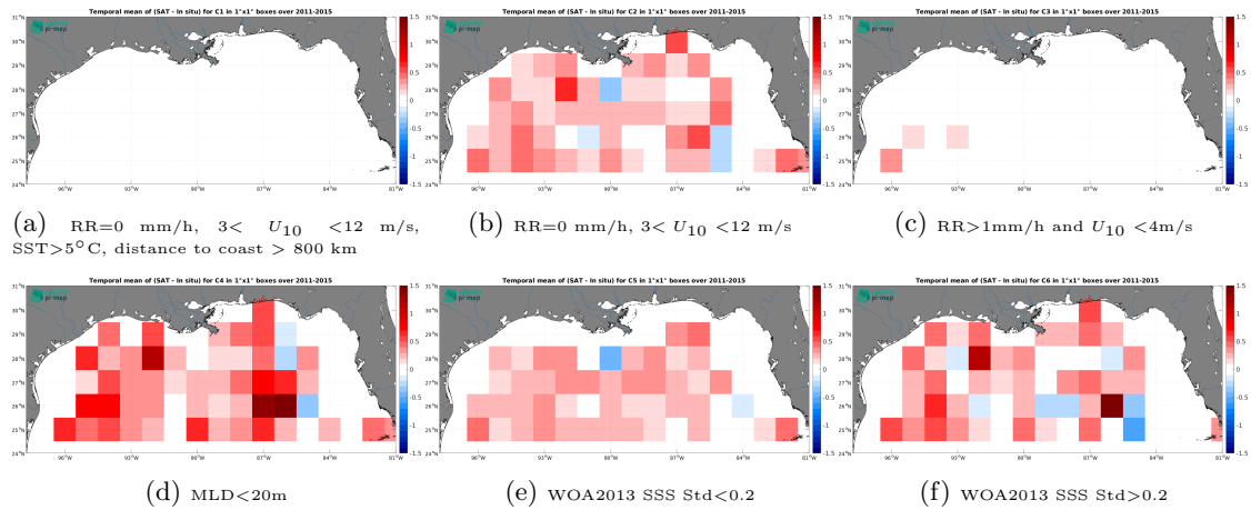
Figure 14: Temporal mean gridded over spatial boxes of size 1^\circ \times 1^\circ of \Delta\text{SSS} (Aquarius SSS L3 OR v5 - Monthly - Rain mask (NASA-GSFC) - Argo) for 6 different subdatasets corresponding to:RR=0 mm/h, 3 < U_{10} < 12 m/s, SST>5°C, distance to coast > 800 km (a), RR=0 mm/h, 3 < U_{10} < 12 m/s (b), RR>1mm/h and U_{10} < 4 m/s (c),MLD<20m (d),WOA2013 SSS Std<0.2 (e),WOA2013 SSS Std>0.2 (f).
