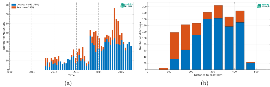
Figure 2: Number of match-ups between Argo and Aquarius SSS L3 OR v5 - Monthly - Rain mask (NASA-GSFC) SSS as a function of time (a) and as function of the distance to coast (b) over the Mississippi river plume Pi-MEP region and for the full satellite product period.
