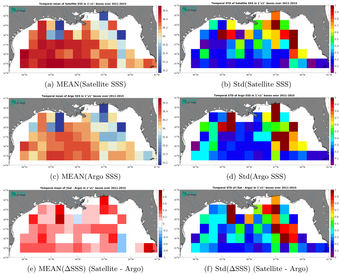
Figure 6: Temporal mean (left) and Std (right) of SSS from Aquarius SSS L3 OR v5 - Monthly - Rain mask (NASA-GSFC) (top), Argo (middle), and of \Delta SSS (Satellite - Argo). Only match-up pairs are used to generate these maps.
