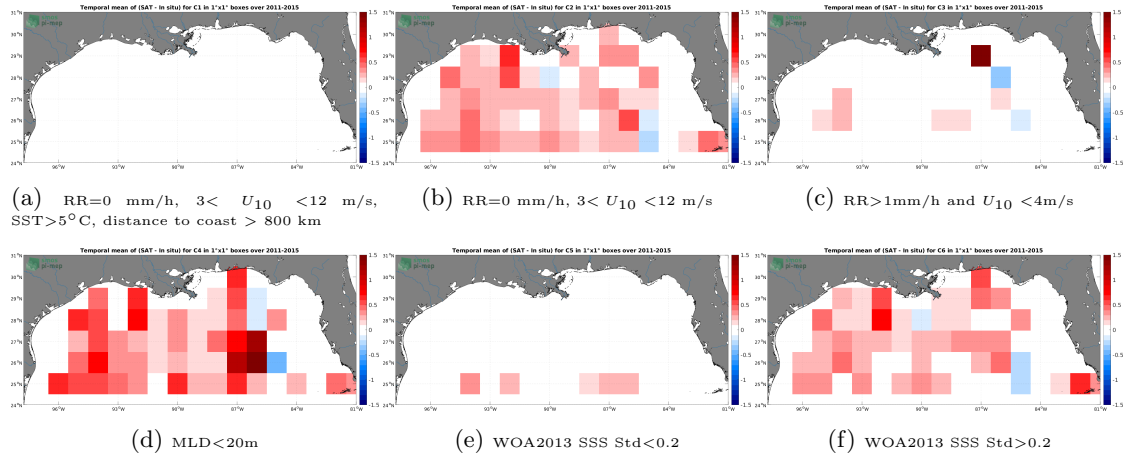
Figure 12: Temporal mean gridded over spatial boxes of size 1^{\circ}\times 1^{\circ} of \Delta\text{SSS} (Aquarius SSS L3 OR v5 - Monthly - Rain mask (NASA-GSFC) - Argo) for 6 different subdatasets corresponding to:RR=0 mm/h, 3 < U_{10} < 12 m/s, SST >5^{\circ}\text{C} , distance to coast > 800 km (a), RR=0 mm/h, 3 < U_{10} < 12 m/s (b), RR >1\text{mm/h} and U_{10} < 4\text{m/s} (c),MLD <20\text{m} (d),WOA2013 SSS Std <0.2 (e),WOA2013 SSS Std >0.2 (f).
