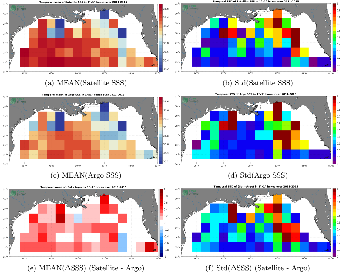
Figure 6: Temporal mean (left) and Std (right) of SSS from Aquarius SSS L3 OR v5 - Monthly - Rain mask (NASA-GSFC) (top), Argo (middle), and of \Delta\text{SSS} (Satellite - Argo). Only match-up pairs are used to generate these maps.
