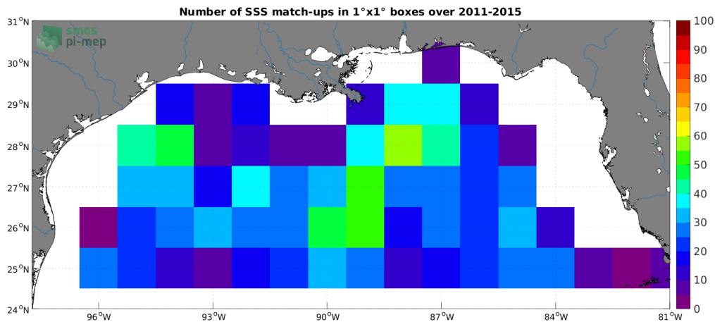
Figure 4: Number of SSS match-ups between Argo SSS and the Aquarius SSS L3 OR v5 - Monthly - Rain mask (NASA-GSFC) SSS product for the Mississippi river plume Pi-MEP region over 1^\circ \times 1^\circ boxes and for the full satellite product period.
