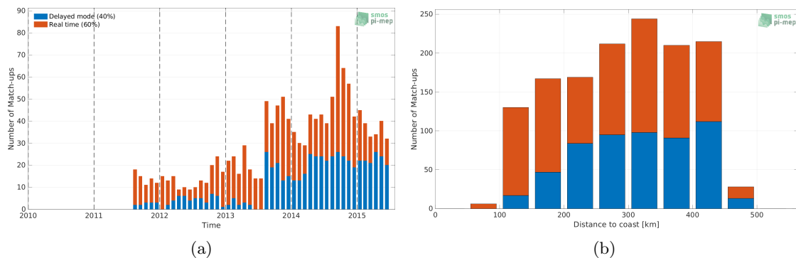
Figure 1: Number of match-ups between Argo and Aquarius SSS L3 OR v5 - Monthly - Rain mask (NASA-GSFC) SSS as a function of time (a) and as function of the distance to coast (b) over the Mississippi river plume Pi-MEP region and for the full satellite product period.
