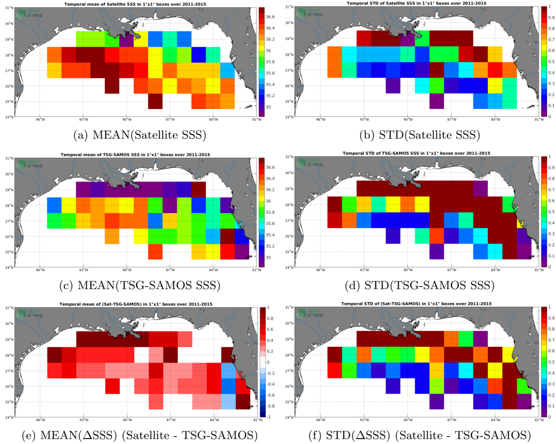
Figure 6: Temporal mean (left) and STD (right) of SSS from Aquarius-L3-JPL-V5-7DAY-RUNNING (top), TSG-SAMOS (middle), and of \Delta SSS (Satellite - TSG-SAMOS). Only match-up pairs are used to generate these maps.
