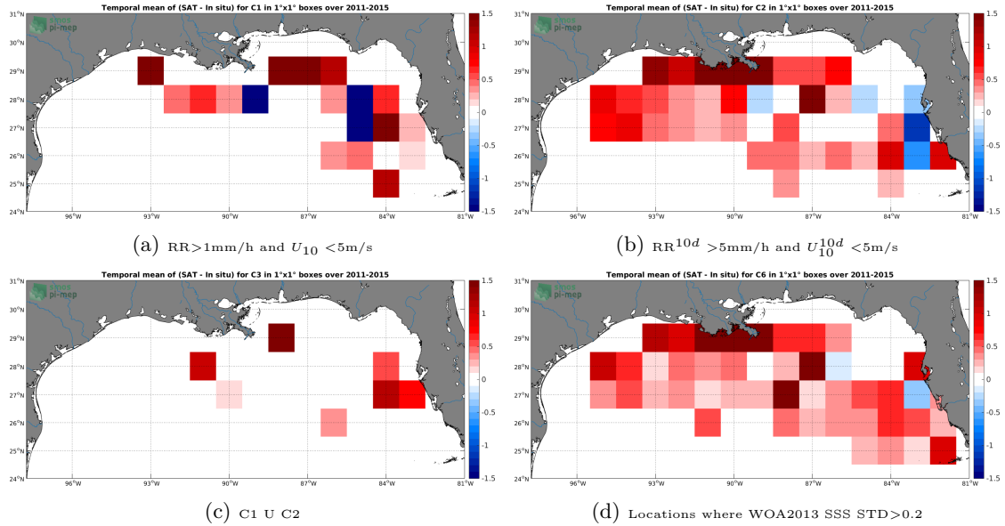
Figure 12: Temporal mean gridded over spatial boxes of size 1^\circ \times 1^\circ of \Delta SSS (Aquarius-L3-JPL-V5-7DAY-RUNNING - TSG-SAMOS) for 4 different subdatasets corresponding to: RR > 1\text{mm/h} and U_{10} < 5\text{m/s} (a), RR^{10d} > 5\text{mm/h} and U_{10}^{10d} < 5\text{m/s} (b), C1 U C2 (c), Locations where WOA2013 SSS STD > 0.2 (d).
