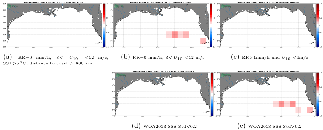
Figure 12: Temporal mean gridded over spatial boxes of size 1^\circ \times 1^\circ of \Delta SSS (Aquarius SSS L3 CAP v5 - 7-Day running (JPL) - TSG (GOSUD-Sailing-ship)) for 5 different subdatasets corresponding to: RR=0 mm/h, 3 < U_{10} < 12 m/s, SST > 5^\circ\text{C} , distance to coast > 800 km (a), RR=0 mm/h, 3 < U_{10} < 12 m/s (b), RR > 1 mm/h and U_{10} < 4 m/s (c), WOA2013 SSS Std < 0.2 (d), WOA2013 SSS Std > 0.2 (e).
