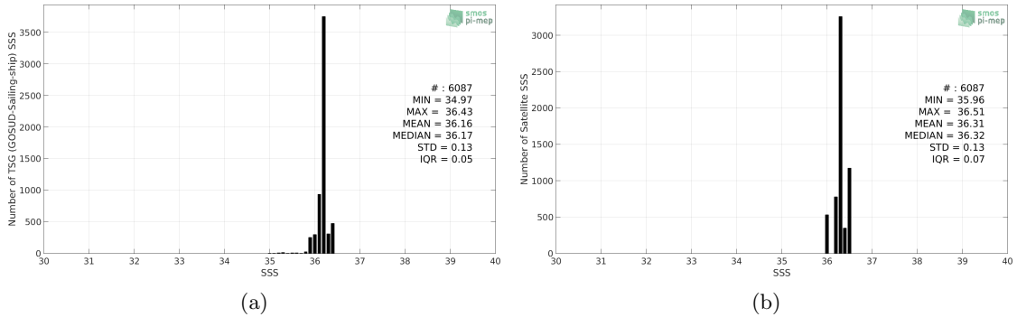
Figure 2: Histograms of SSS from TSG (GOSUD-Sailing-ship) (a) and Aquarius SSS L3 CAP v5 - 7-Day running (JPL) (b) considering all match-up pairs per bins of 0.1 over the Mississippi river plume Pi-MEP region and for the full satellite product period.
