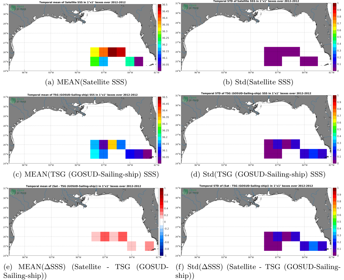
Figure 6: Temporal mean (left) and Std (right) of SSS from Aquarius SSS L3 CAP v5 - 7-Day running (JPL) (top), TSG (GOSUD-Sailing-ship) (middle), and of \Delta\text{SSS} (Satellite - TSG (GOSUD-Sailing-ship)). Only match-up pairs are used to generate these maps.
