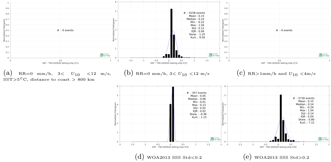
Figure 13: Normalized histogram of \Delta\text{SSS} (Aquarius-L3-JPL-V5-7DAY-RUNNING - TSG-GOSUD-Sailing-ship) for 5 different subdatasets corresponding to: RR=0 mm/h, 3 < U_{10} < 12 m/s, SST > 5^{\circ}\text{C} , distance to coast > 800 km (a), RR=0 mm/h, 3 < U_{10} < 12 m/s (b), RR > 1\text{mm/h} and U_{10} < 4\text{m/s} (c), WOA2013 SSS Std < 0.2 (d), WOA2013 SSS Std > 0.2 (e).
