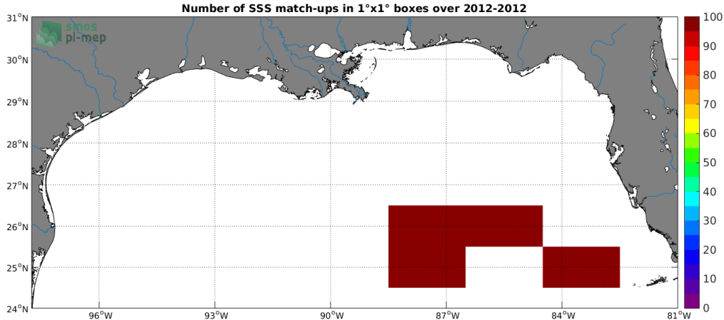
Figure 4: Number of SSS match-ups between TSG-GOSUD-Sailing-ship SSS and the Aquarius-L3-JPL-V5-7DAY-RUNNING SSS product for the Mississippi river plume Pi-MEP region over 1°x1° boxes and for the full satellite product period.
