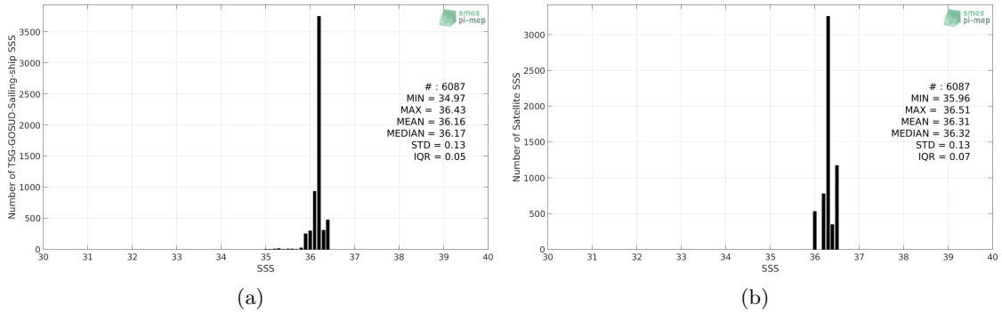
Figure 2: Histograms of SSS from TSG-GOSUD-Sailing-ship (a) and Aquarius-L3-JPL-V5-7DAY-RUNNING (b) considering all match-up pairs per bins of 0.1 over the Mississippi river plume Pi-MEP region and for the full satellite product period.
