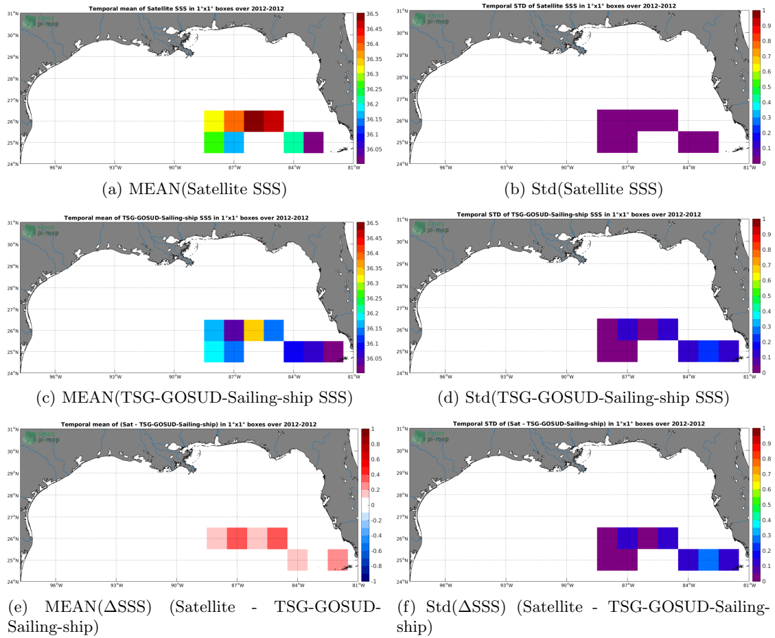
Figure 6: Temporal mean (left) and Std (right) of SSS from Aquarius-L3-JPL-V5-7DAY-RUNNING (top), TSG-GOSUD-Sailing-ship (middle), and of \Delta SSS (Satellite - TSG-GOSUD-Sailing-ship). Only match-up pairs are used to generate these maps.
