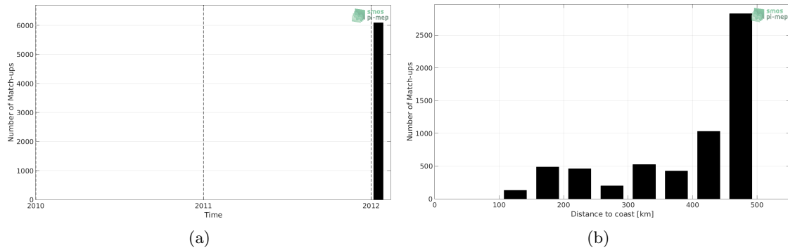
Figure 1: Number of match-ups between TSG-GOSUD-Sailing-ship and Aquarius-L3-JPL-V5-7DAY-RUNNING SSS as a function of time (a) and as function of the distance to coast (b) over the Mississippi river plume Pi-MEP region and for the full satellite product period.
